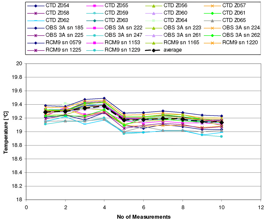
Figure 4-13: Temperature measurements
