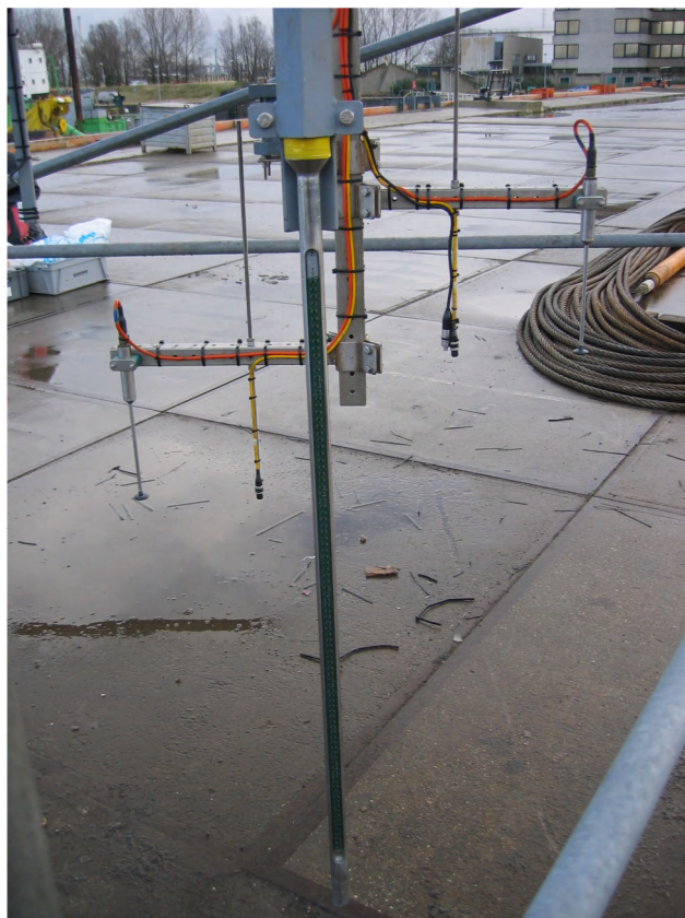
Figure 2-3: ARGUS ASM-IV
