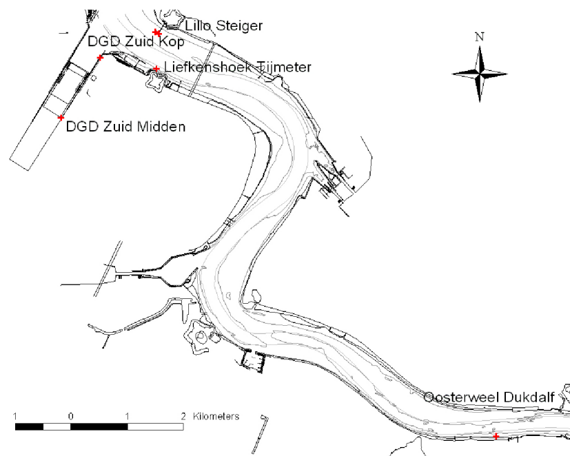
Calibration measurements - 15/03/2006 & 14/04/2006
