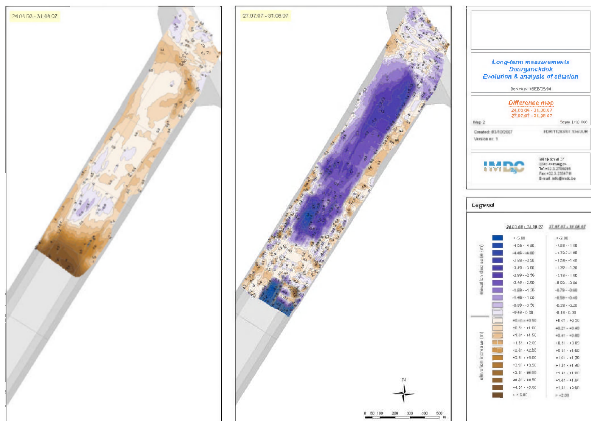
Figure 4-4: Difference charts of the depth sounding on 31/08/07: in reference to t_{0e} (left), and to the previous measurement (right) on 27/07/07
