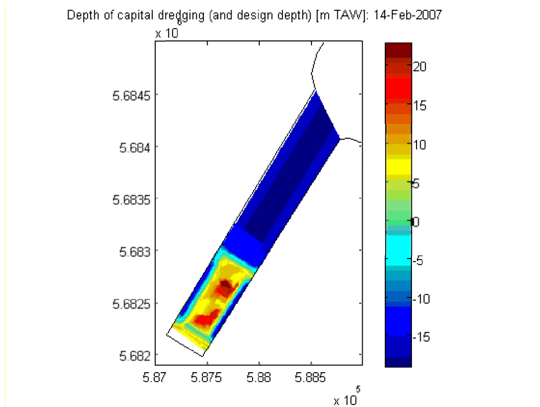
Figure 5-2: Depth before capital dredging works started from the dockside in February 2007 (for the operational part of the dock, the design depth is showed)
