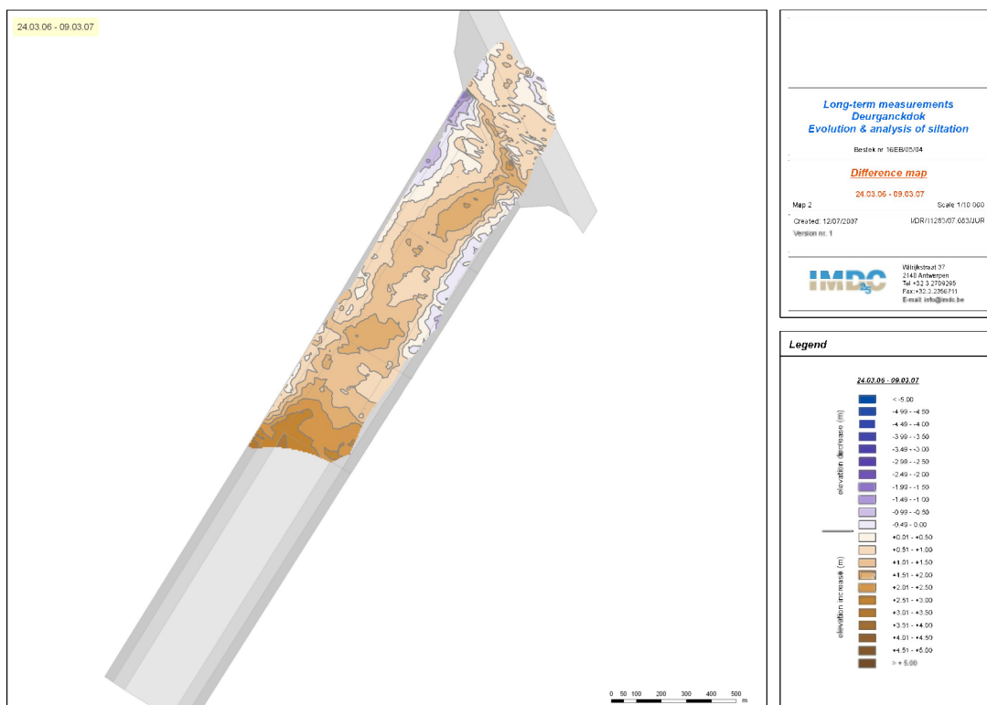
Figure 4-4: Difference charts of the depth sounding on 9/03/07 in reference to t_{oe}
