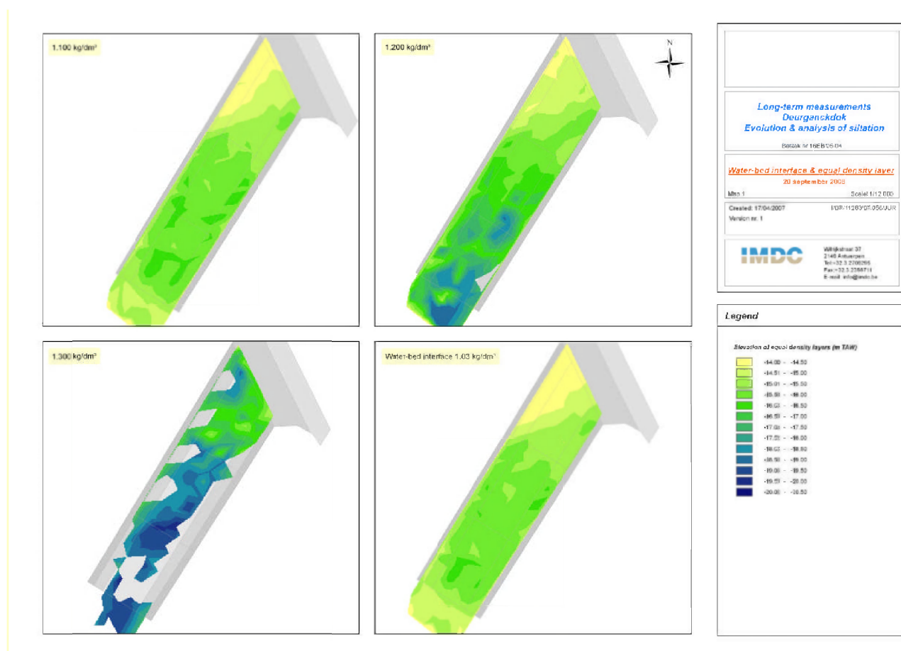
Figure 4-8: Map of the depth of the water-bed interface and equal density layers for 20/09/06
