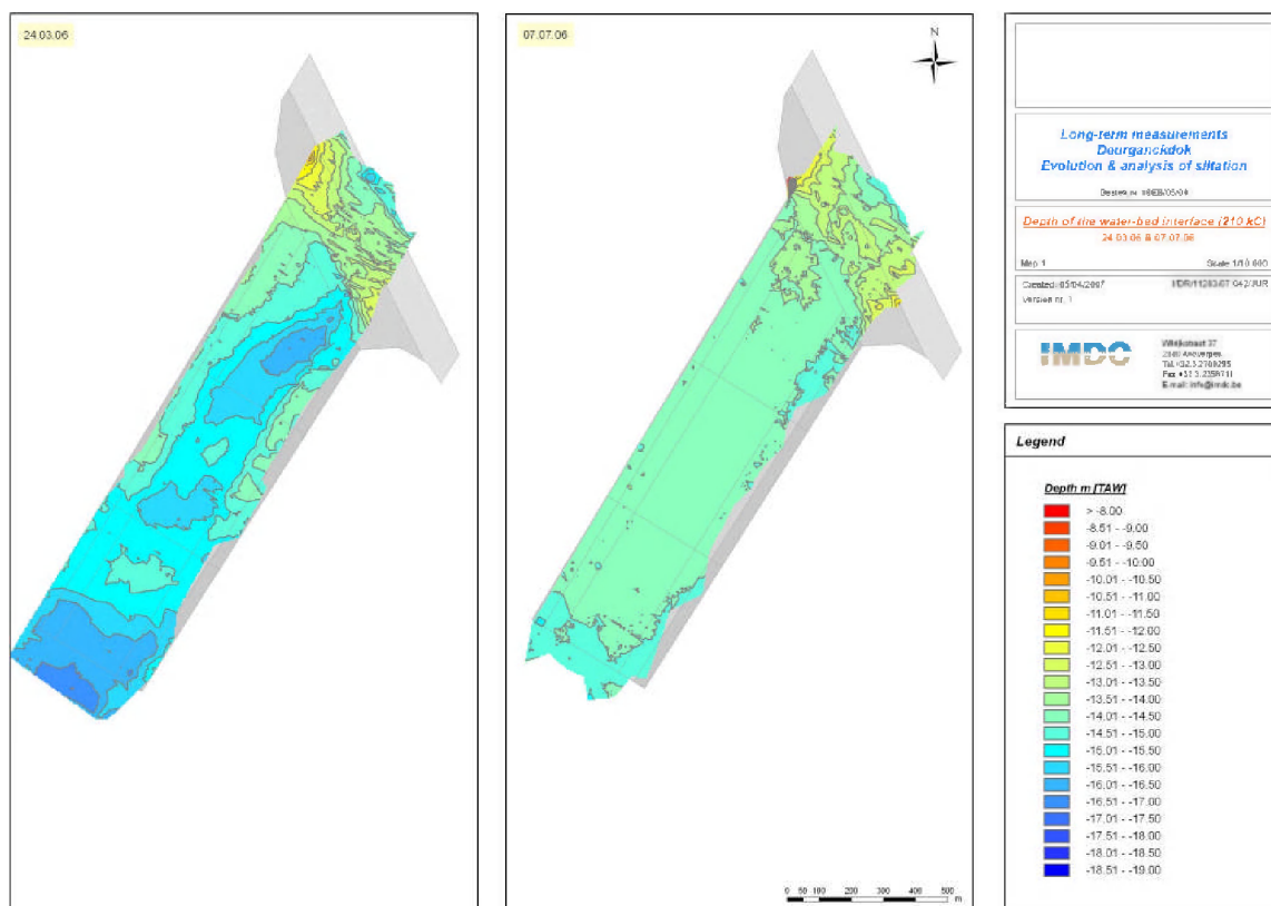
Figure 4-3: Example of a map showing depth of water-bed interface (210 kC) for 24/03/06 and 7/07/06
