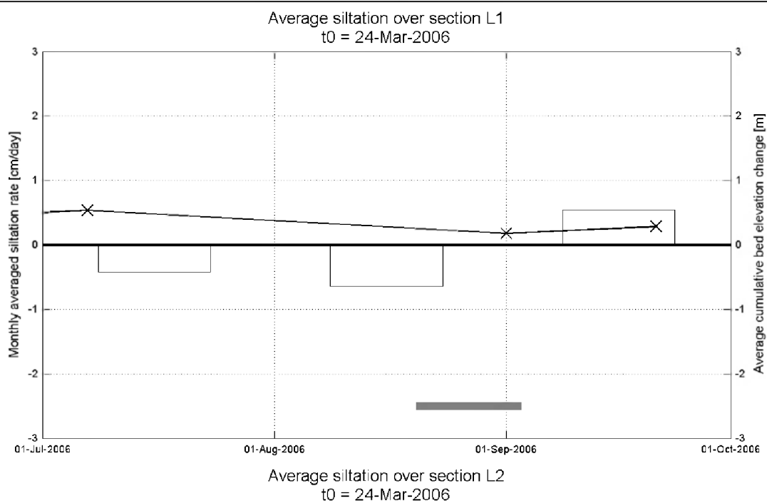
Figure 4-6: Volumetric siltation rate for section L1
