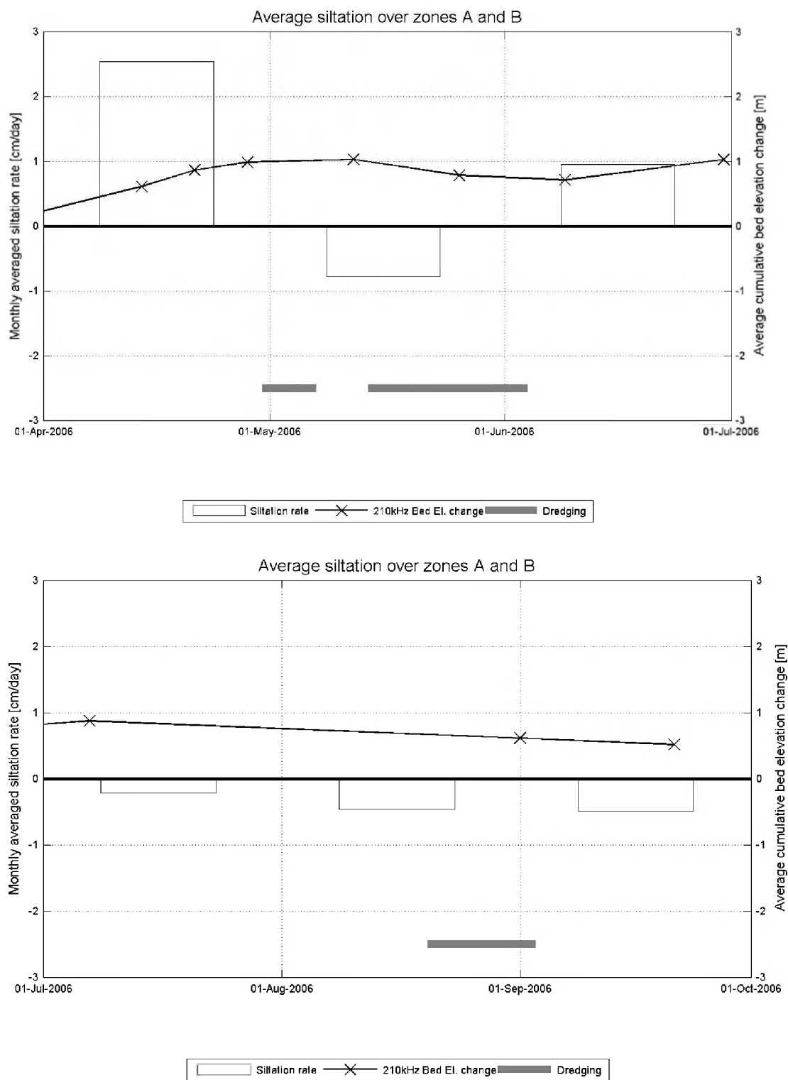
Figure 5-1: Monthly averaged siltation rate [cm/day] for the former (April – July 2006) and the present measurement period (July – September 2006) ( t_{0e} : 24/03/2006)
