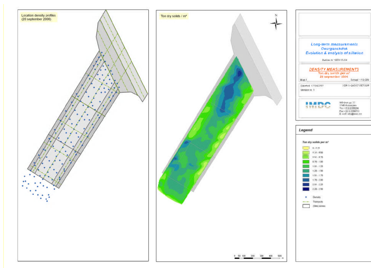
Figure 4-9: Map showing the location of the density profiles (left) and the calculation of TDS (right) on 20/09/06
