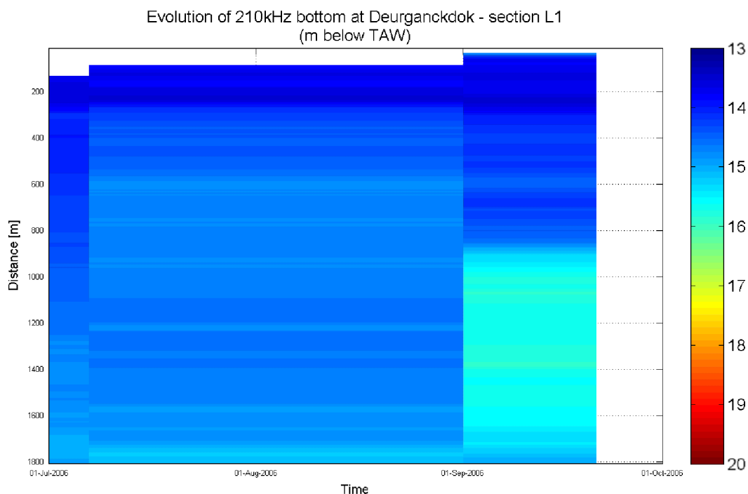
Figure 4-5: Graph of Evolution of the water-bed interface (210 kC) for section L1
