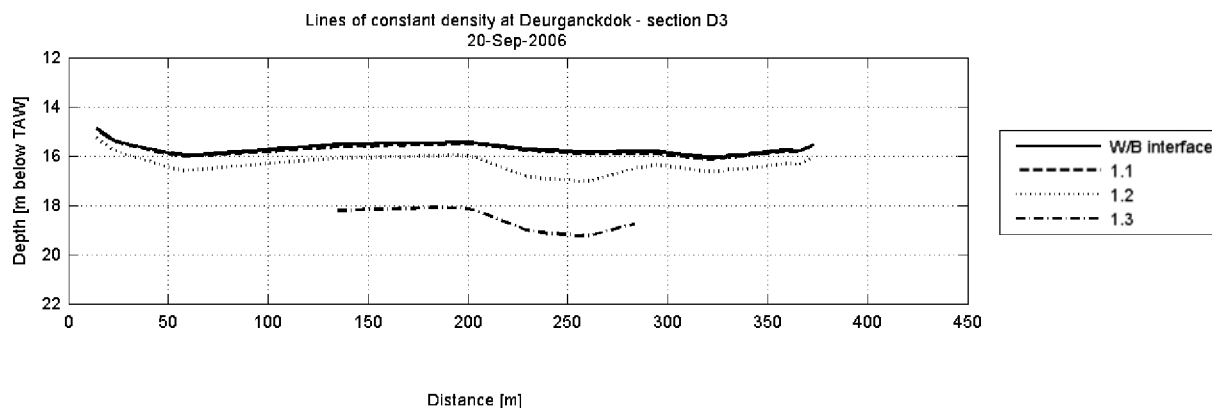
Figure 4-7: Depth of water-bed interface and equal density layers in section D3 on 20 September 2006
