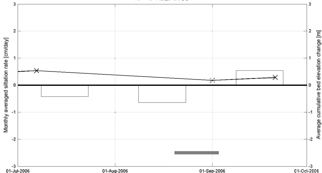
Average siltation over section L2 t0 = 24-Mar-2006
