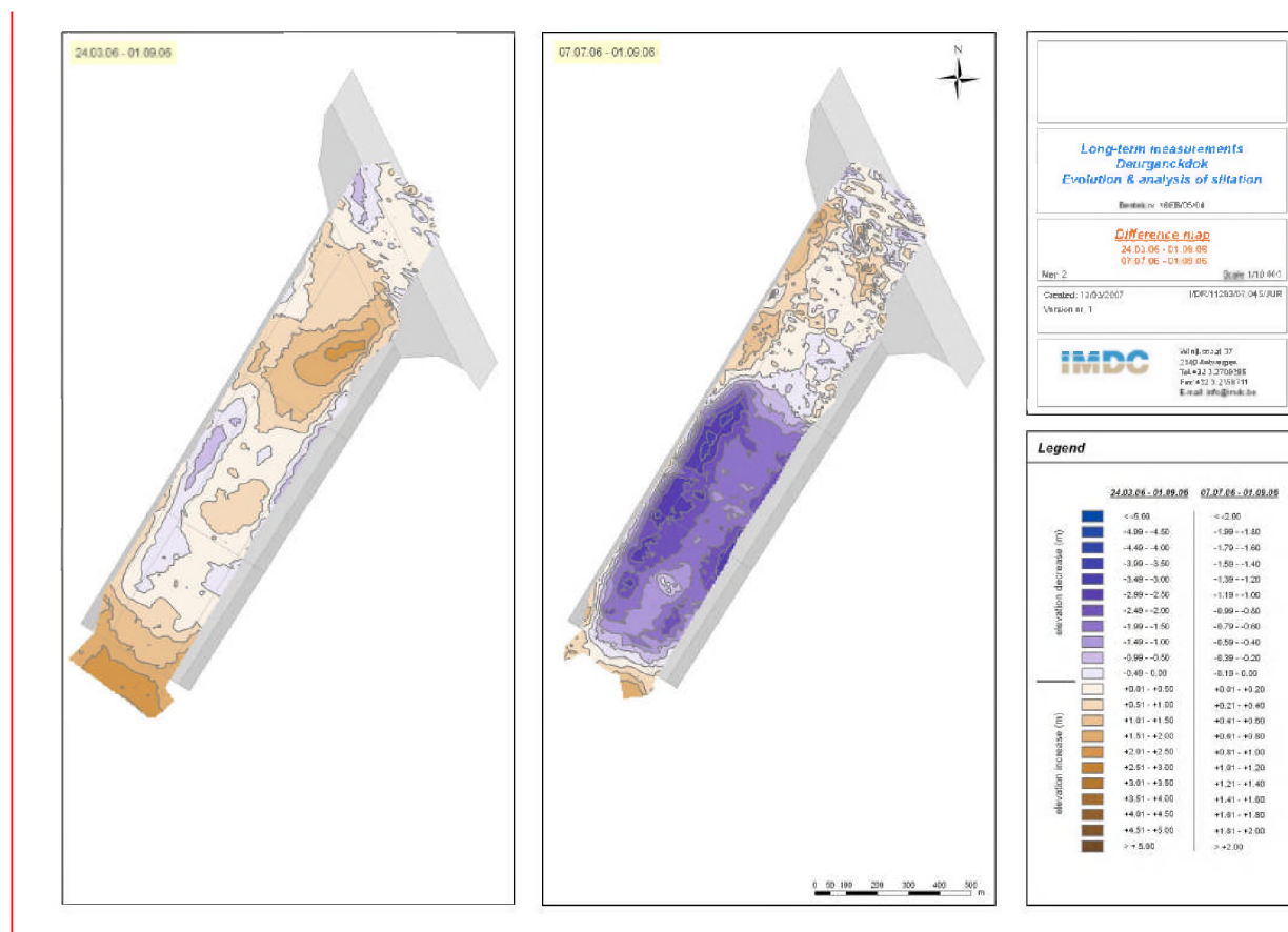
Figure 4-4: Difference charts of the depth sounding on 1/09/06: in reference to t_{0e} (left), and to the previous measurement (right) on 7/07/06
