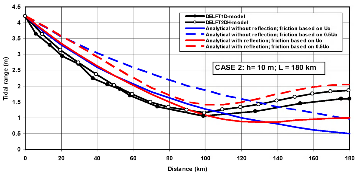
Figure A7 Computed tidal range for prismatic channel CASE 2 based on DELFT1D-model and Analytical model
