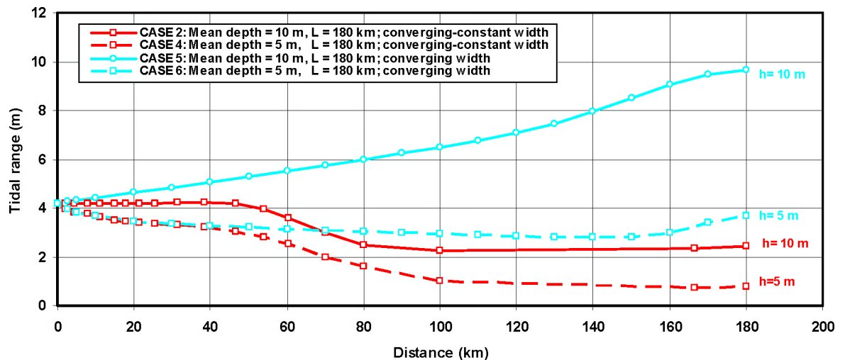
Figure B12 Comparison of computed tidal ranges for converging-prismatic channel and converging channel based on DELFT1D-model
