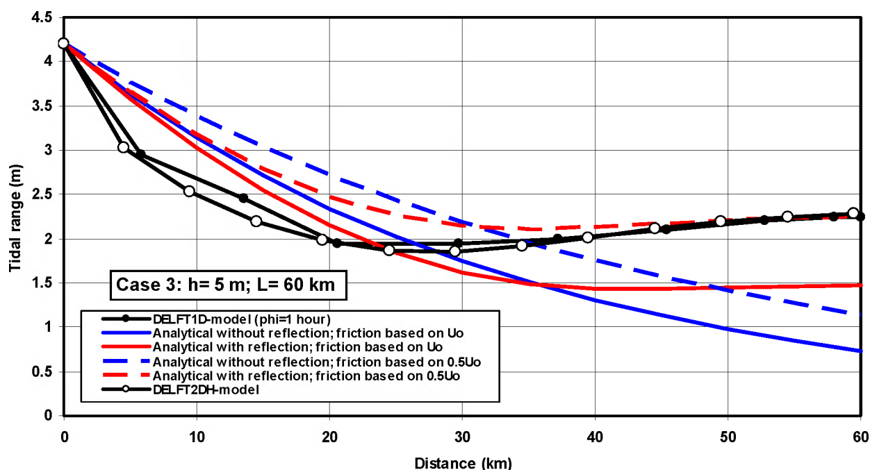
Figure A6 Computed tidal range for prismatic channel CASE 3 (DELFT1D and Analytical model)
