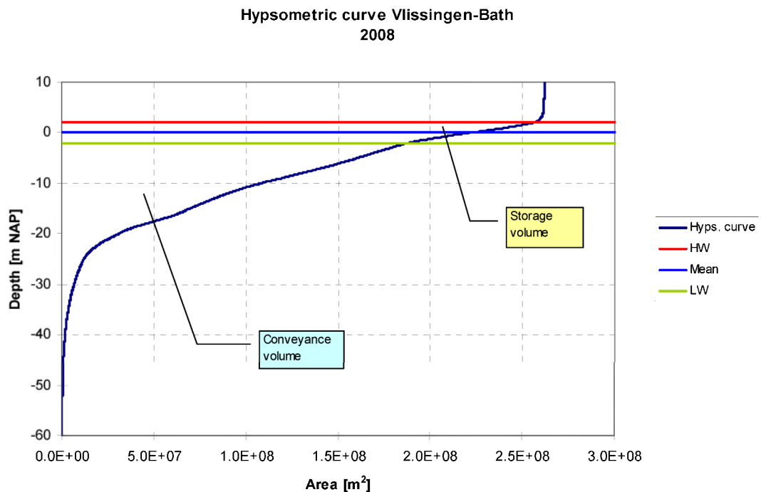
Figure 4.12 Hypsometry for the section Vlissingen-Bath in the year 2008 (Deltares, 2010).
