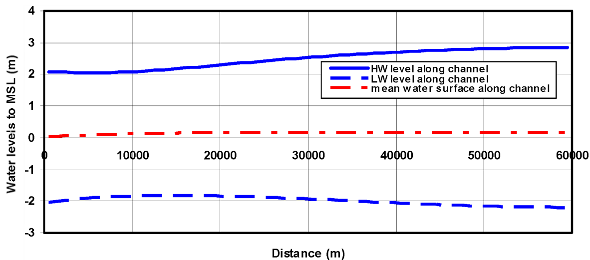
Figure A9 Computed tidal range and mean surface level for prismatic channel CASE 1 ( L=60 km, h=10 m) based on DELFT2DH-model
