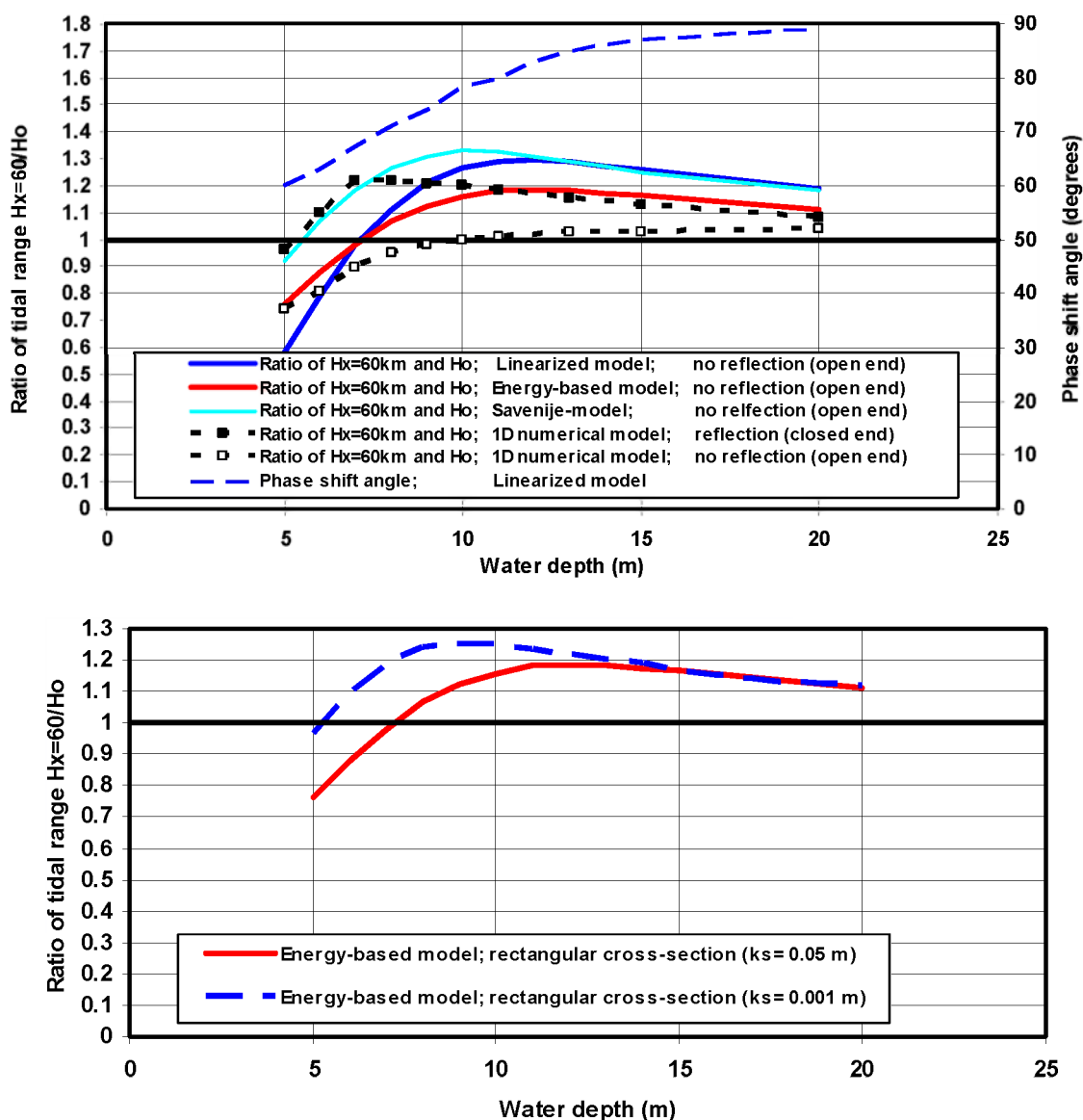
Figure 4.9 Ratio H_{x=60km}/H_o for a converging channel (Scheldt Estuary) Top: Results of various methods ( k_s = 0.05 m = constant) Bottom: Effect of k_s for energy-based method
