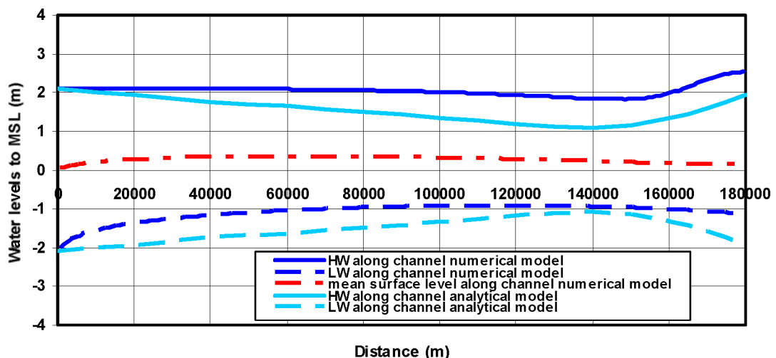
Figure B18 Computed tidal range and mean surface level for converging channel CASE 6 ( L = 180 km, h = 5 m) based on DELFT2DH-model
