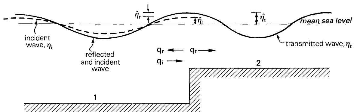
Figure 2.2 Wave reflection at discontinuity
