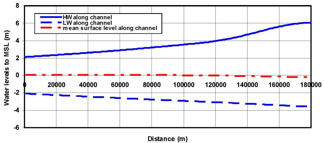
Figure B17 Computed tidal range and mean surface level for converging channel CASE 5 ( L = 180 km, h = 10 m) based on DELFT2DH-model
