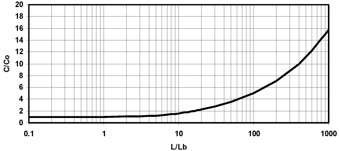
Figure 3.2 Ratio c/c_0 as function of L/L_b
