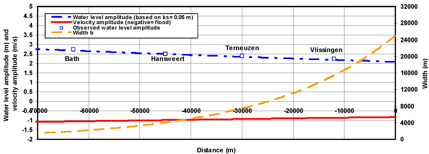
Figure 4.6 Water level amplitude and velocity amplitude along estuary, Scheldt Estuary
