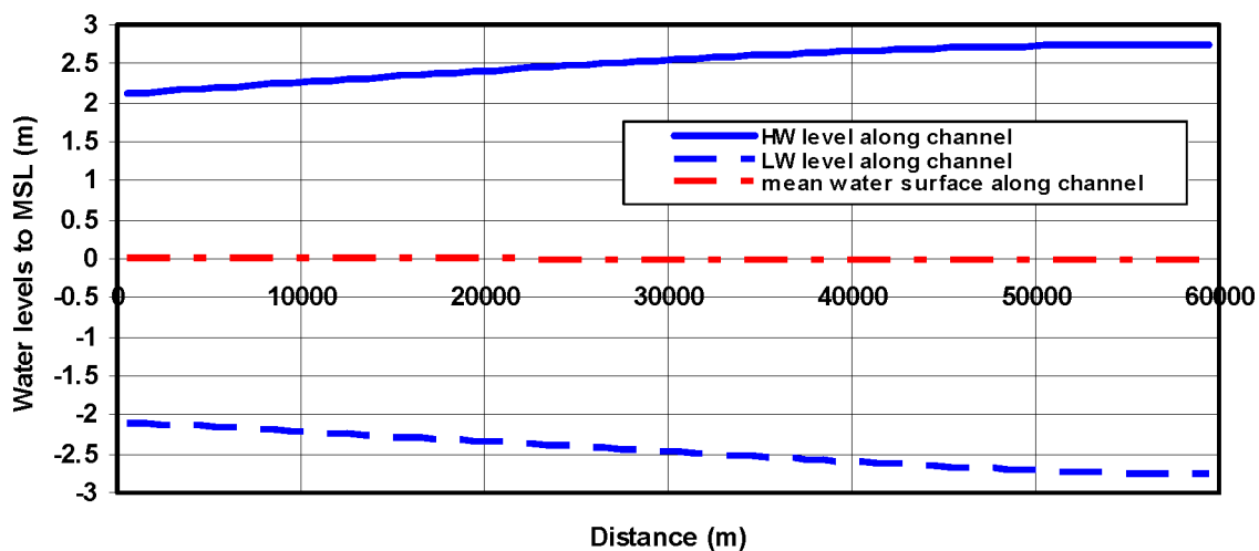
Figure B13 Computed tidal range and mean surface level for converging channel CASE 1 ( L = 60 km, h = 10 m) based on DELFT2DH-model
