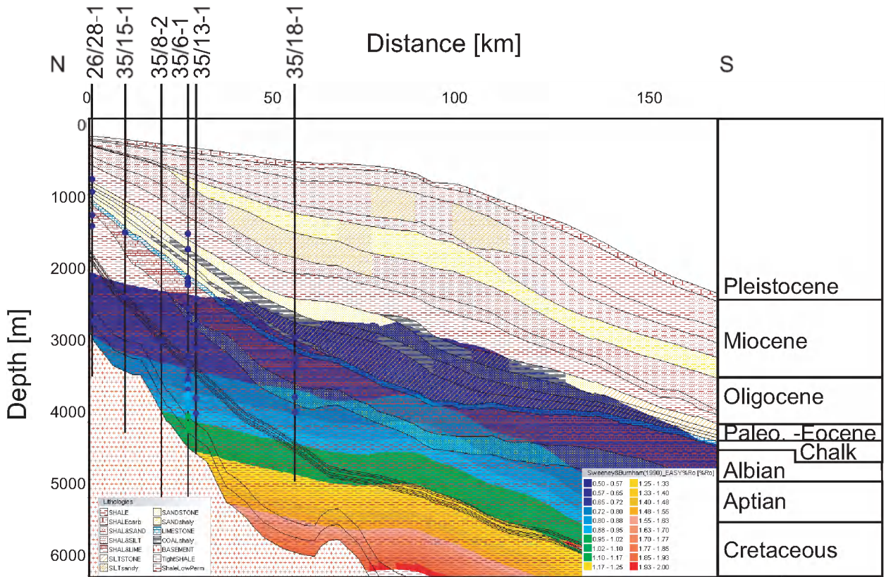
Fig.3. Line RE94 with calibration wells and calculated vitrinite reflectance (Easy R_o ) (Sweeney and Burnham, 1990) overlay; the coloured area shows the maturity distribution between 0.5 and 2% R_o . The coloured dots on the wells represent the measured vitrinite reflectance.
