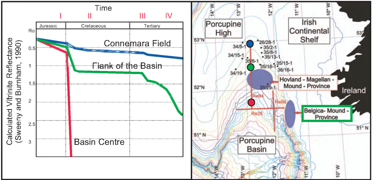
Fig. 10. Evolution of the maturity of a postulated Upper Jurassic source rock at three locations in the basin (blue: Connemara field; green: flank of the basin; red: basin centre).
