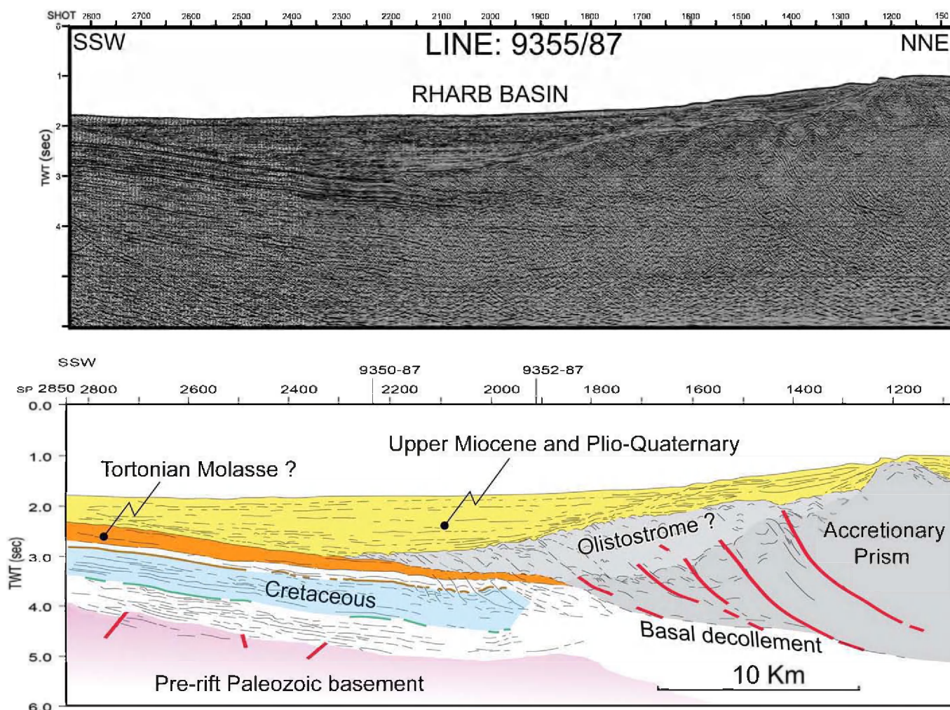
Fig. 7. Multi-channel seismic line ONAREP 9355-87. Mcs Line encompassing the Gulf of Cadiz accretionary wedge at the Rharrb Valley, in the Moroccan offshore (modified after Camurri, 2004). Location in Fig. 3.
