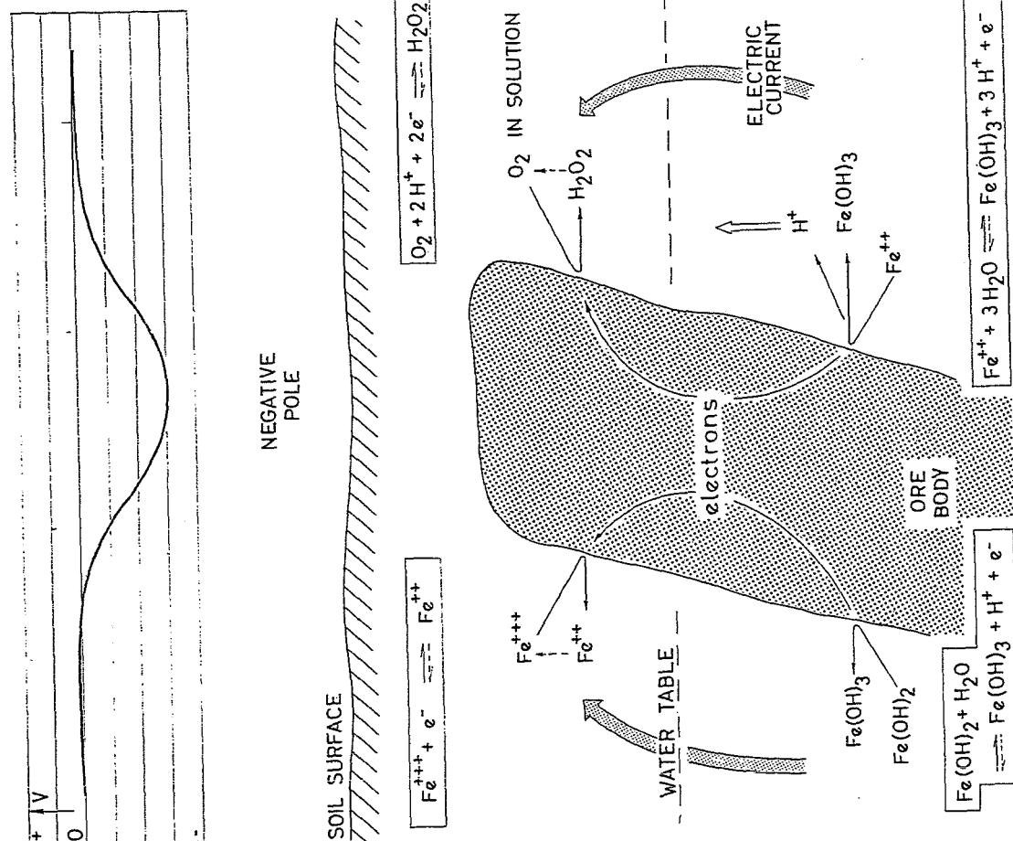
Fig. 6. Electrochemical S.P. mechanism, after SATO and MOONEY (1960).
