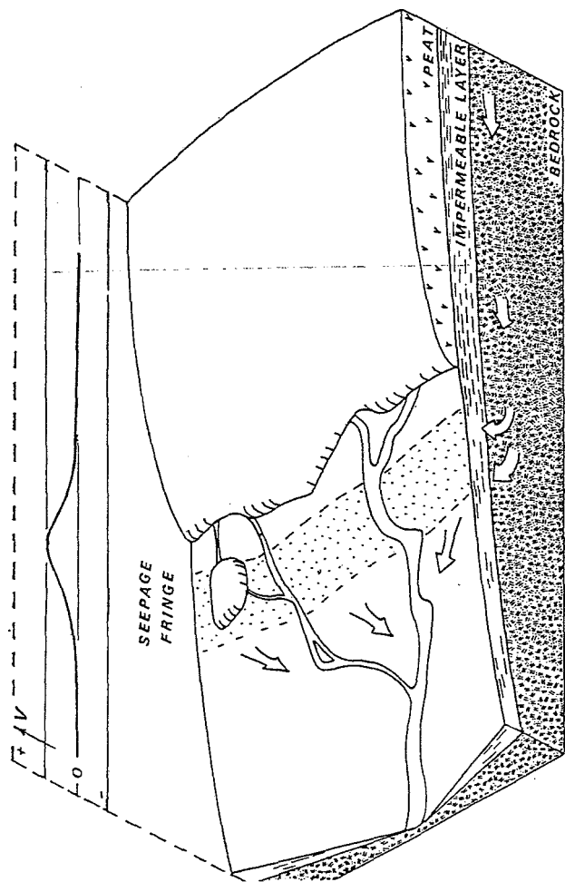
Fig. 8. Scheme illustrating the electrofiltration hypothesis for the generation of positive S.P. anomalies downstream the raised bog of Champfa-Grandpassage.
