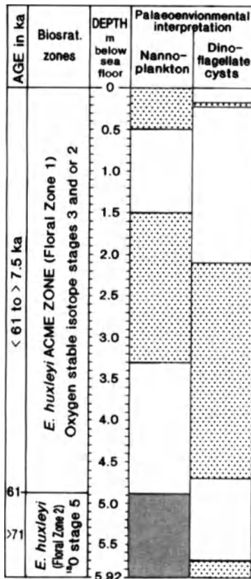
Fig 5. Detailed late Quaternary-Holocene stratigraphy of cores 46 and 37 from the Faroe-Shetland Channel.
