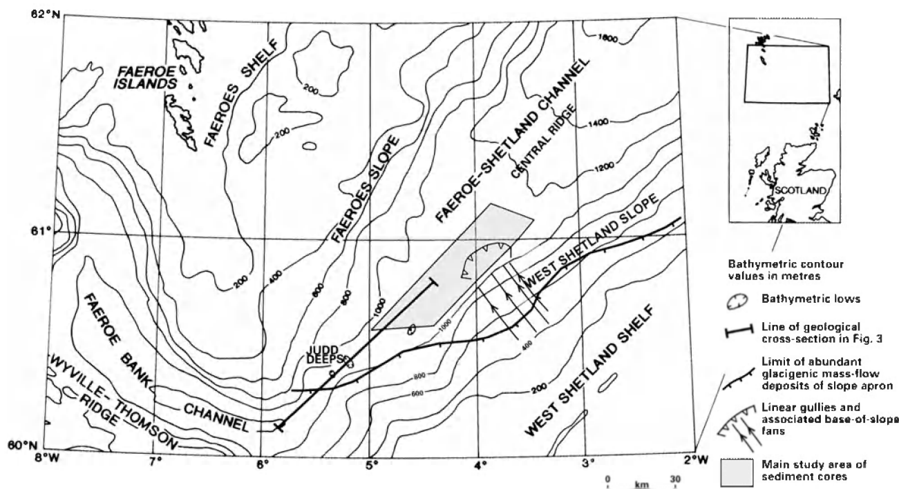
Fig 1. Location map and bathymetry of the SW Faroe–Shetland Channel region, showing the main area of study of the sediment cores. The limit of glacialic mass-flow slope-apron deposits is taken from Stoker (1999), and the linear gullies and associated fans is adapted from Stoker et al. (1993) Masson (2001) and Bulat & Long (in press). Note that debris flows interbedded with the basinal section occur within the channel (e.g. see Fig. 7).
