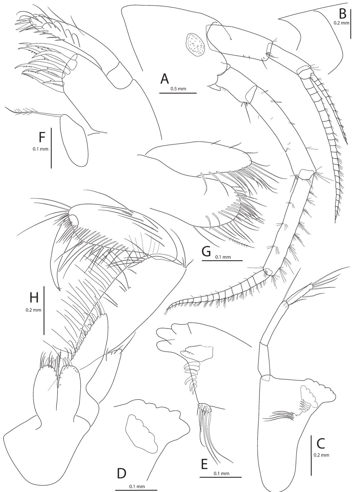
Fig. 35. — Liljeborgia nesiotica D'UDEKEM D'ACQZ, 2008, Bouvetøya, BENDEX, sta. 028-I. A, adult ♂; B-F, ovigerous ♀. A, head and antennae; B, rostrum; C, left Md; D, tip of left Md; E, tip of right Md; F, left Mx1; G, right Mx2; H, Mx3.
