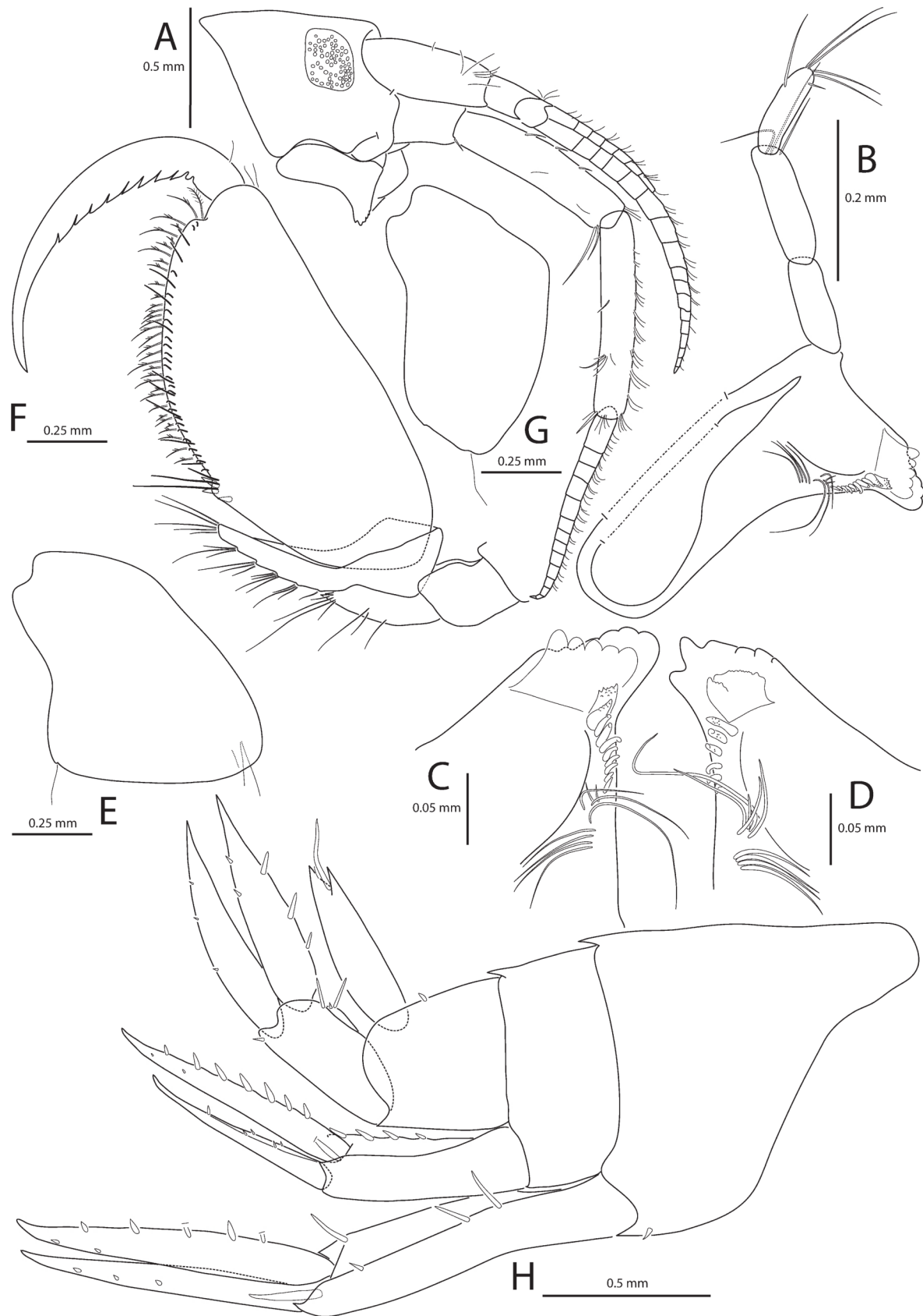
Fig. 22. — Liljeborgia cryptothrix D'UDEKEM D'ACQZ, 2008, nearly mature ♀, Macquarie Isl., R/V Eltanin, cruise 27, sta. 1974. A, head with antennae; B, left Md; C, tip of left Md; D, tip of right Md; E, right coxa 1; F, left Gn2; G, right coxa 2; H, urosome.
