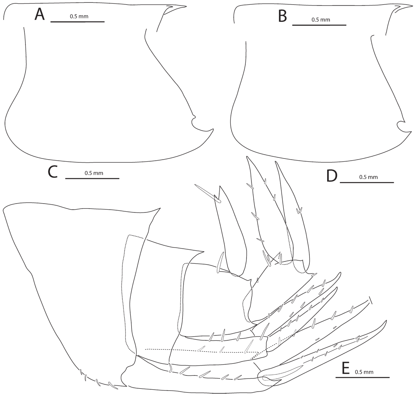
Fig. 41. – Liljeborgia nesiatica D'UDEKEM D'ACOZ, 2008, King George Isl. A, B, C, E, ovigerous ♀, ARC93, sta. CA 105; D, presumably ♀, Arc93, sta. F11. A, dorsal border of pleonite 1; B, dorsal border of pleonite 2; C, D, Ep3; E, urosome.
