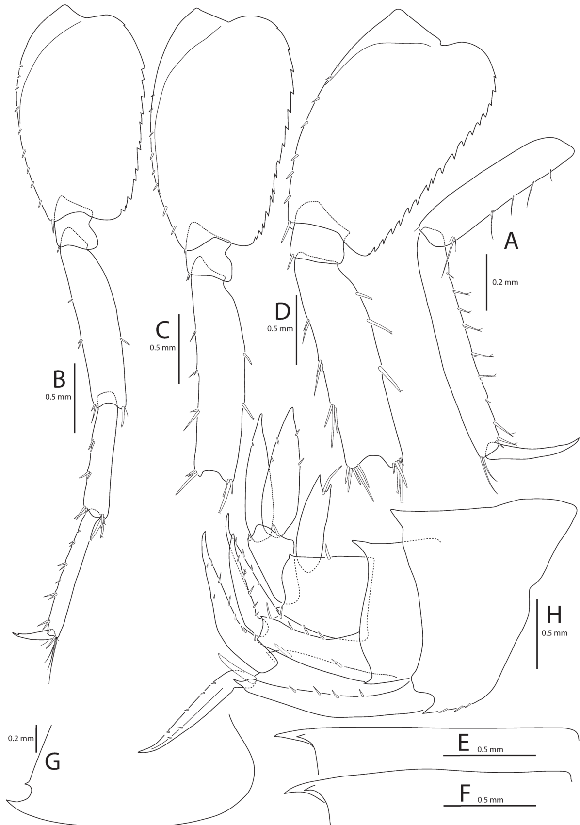
Fig. 42. – Liljeborgia nesiatica D'UDEKEM D'ACÓZ, 2008, ovigerous ♀, Ross Sea, R/V Eltanin, sta. 2120. A, tip of left P4; B, left P5; C, left P6 (tip missing); D, left P7 (tip missing); E, dorsal part of pleonite 1; F, dorsal part of pleonite 2; G, Ep3; H, urosome.
