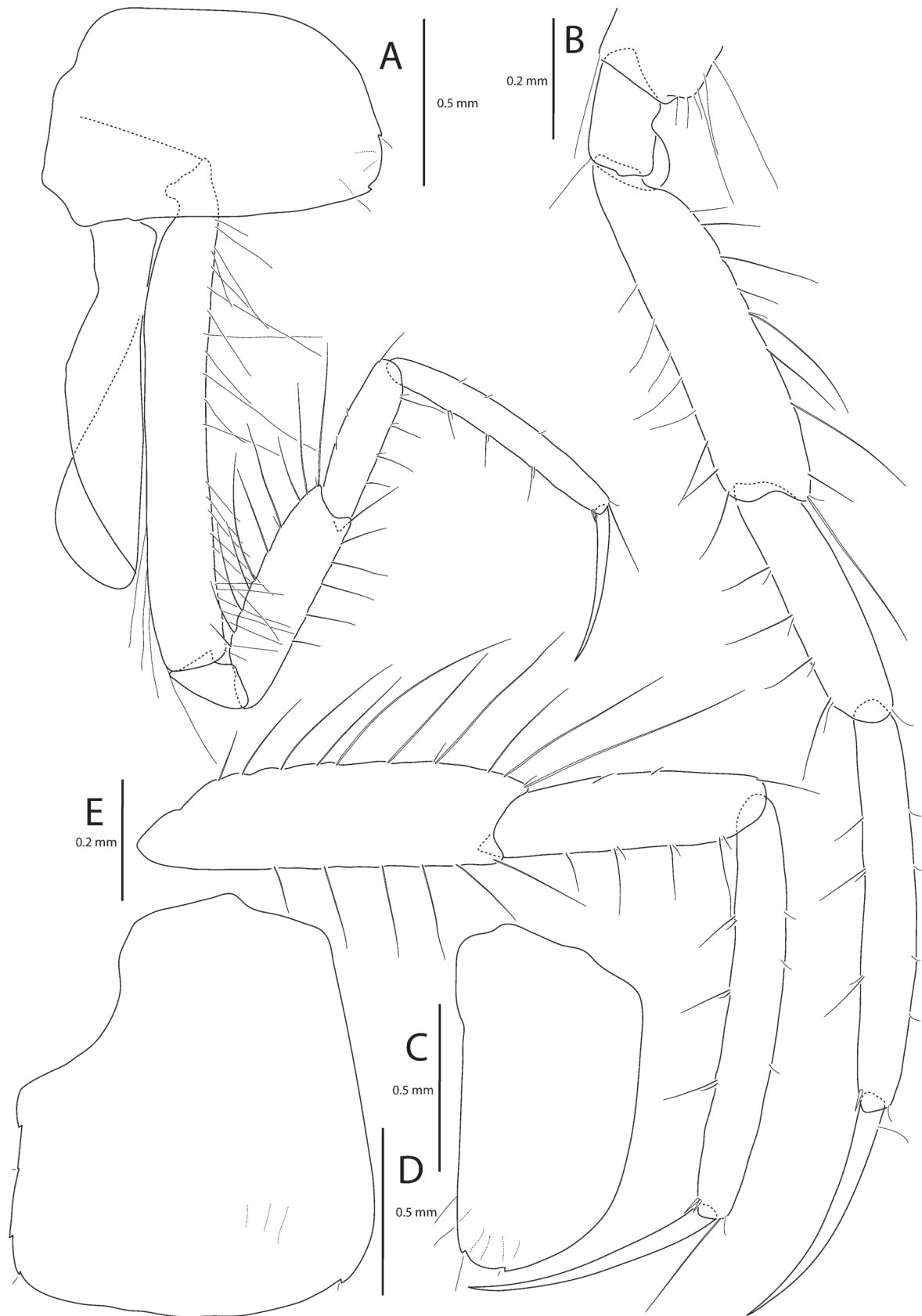
Fig. 10. — Liljeborgia barhami HURLEY, 1954, Stewart Isl.; A-B, D-E, adult ♂; C, mature ♀. A, right P3; B, tip of right P4; C, coxa 3; D, coxa 4; E, tip of right P3. Note the difference in width between the coxa 3 of the ♂ and that of the ♀.
