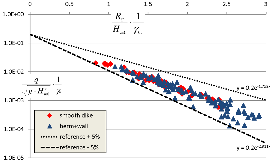
Figure 17. Good description of the situation berm+wall when reduction factor \gamma_{bw} is implemented in the reference formula
