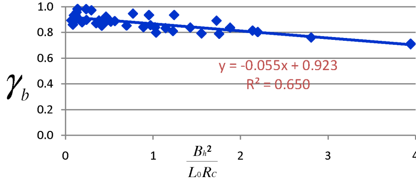
Figure 10. Reduction factor \gamma_b as a function of the dimensionless berm length
