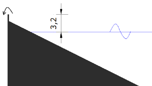
Figure 20. Due to \gamma_v the overtopping is 17.3l/s/m in stead of 42.3l/s/m
