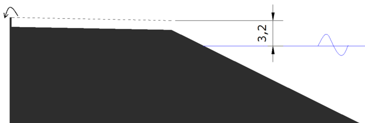
Figure 21. Dike with berm and storm wall. q = 4.3\text{l/s/m}
