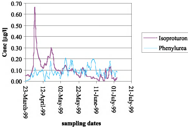
Concentrations of phenylurea herbicides and isoproturon measured by immunoassay (in \mu\text{g/l} )
