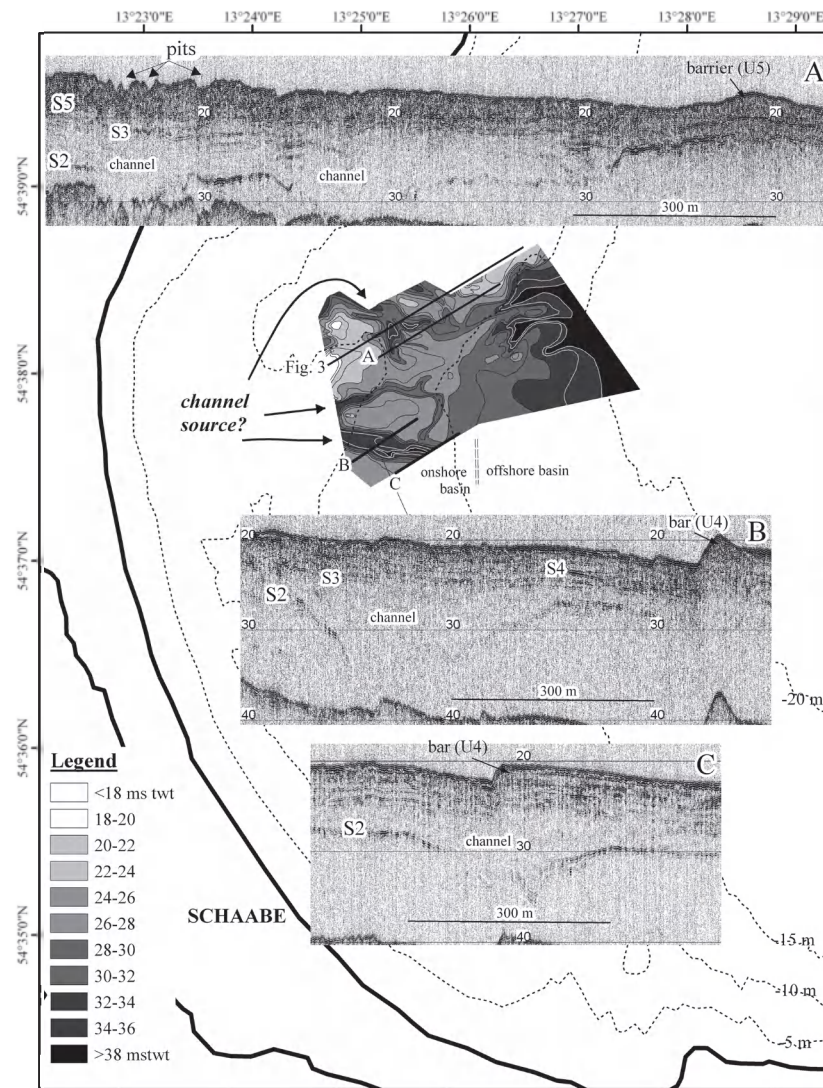
Figure 5. Isochrons of surface S2 and details of the seismic profiles.
