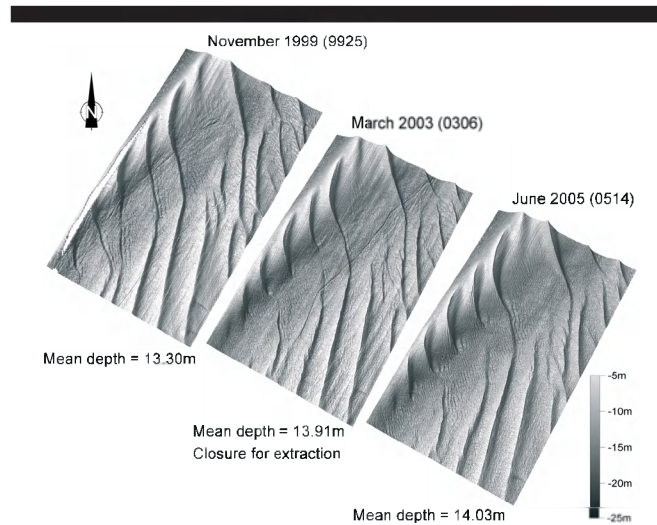
Figure 6. Successive terrain models of the KBMA monitoring area (depth in negative values and referenced to MLLWS). Notice the trailer-dredged furrow marks within the depression, in November 1999 and March 2003.
