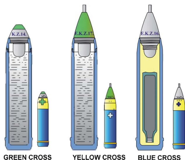
Figure 5.2 German toxic munition from WWI. Green cross shells contain (di)phosgene or chloropicrin, yellow cross shells contain mustard gas, blue cross shells contain Clark. The latter differ from the other toxic shells in the fact that the toxic agent is stored in a glass bottle.
