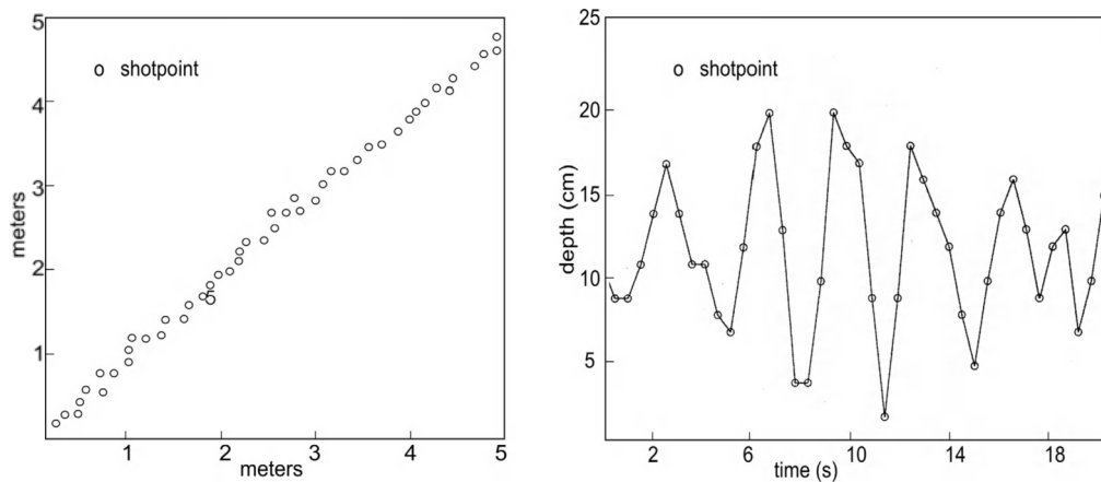
Figure 2.12 Source-mounted antenna movement at sea. Left: lateral movement. Right: vertical movement.
