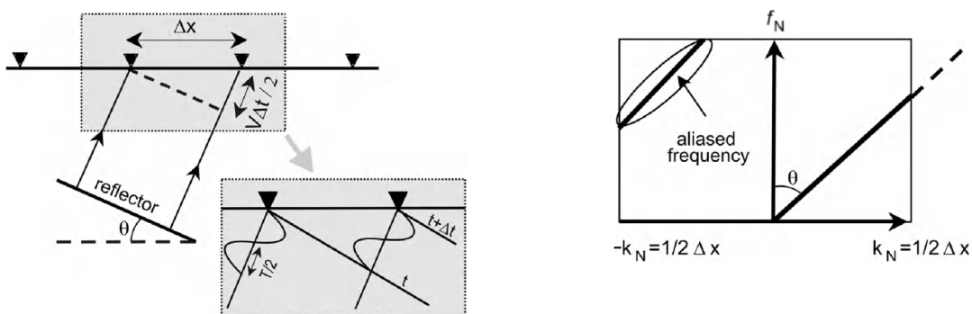
Figure 2.17 Spatial aliasing aspect in the time domain (left) and wavenumber domain (right).
