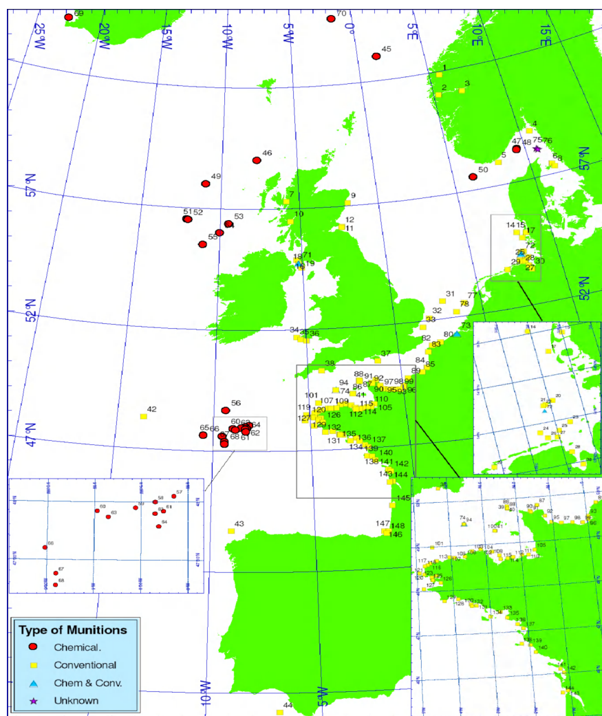
Figure 4.2 Location of conventional and chemical munition dumpsites in the North Sea and NE Atlantic (after OSPAR 2005). Chemical munition dumpsites are marked in red. Conventional munition dumpsites are marked in yellow.
