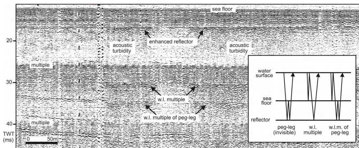
Figure 8.7 Seismic profile showing different types of multiples related to a gas horizon (w.l. = water layer). The vertical disturbances observed on the left are most likely due to acoustic noise.
