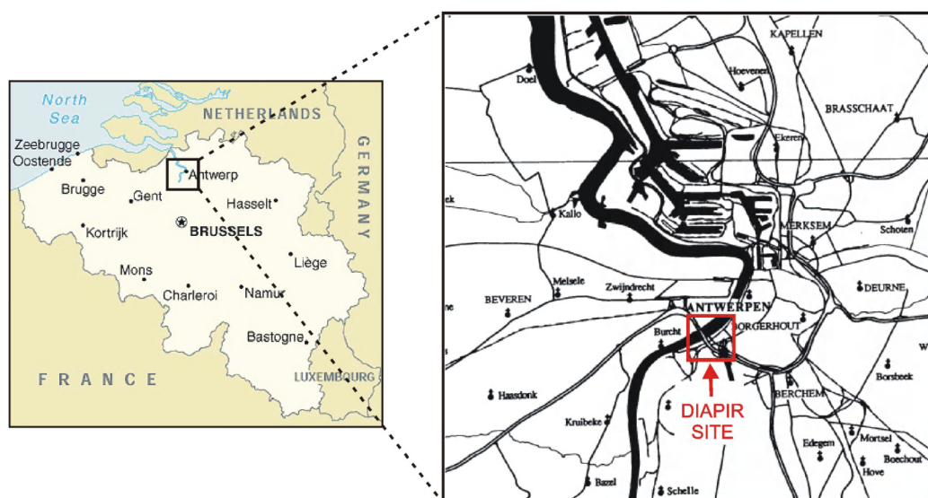
Figure 3.1 Location of the diapir in the Boom Clay under the Schelde river near Antwerpen.
