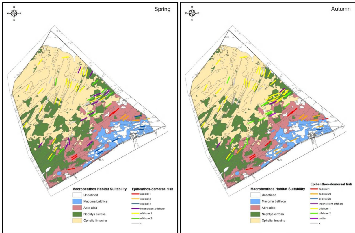
Figure 2: Overlay of demersal fish and epibenthos communities per sampling station on the macrobenthos habitat suitability map (from Degraer et al. 2009) of the BPNS for spring (left) and autumn (right).
