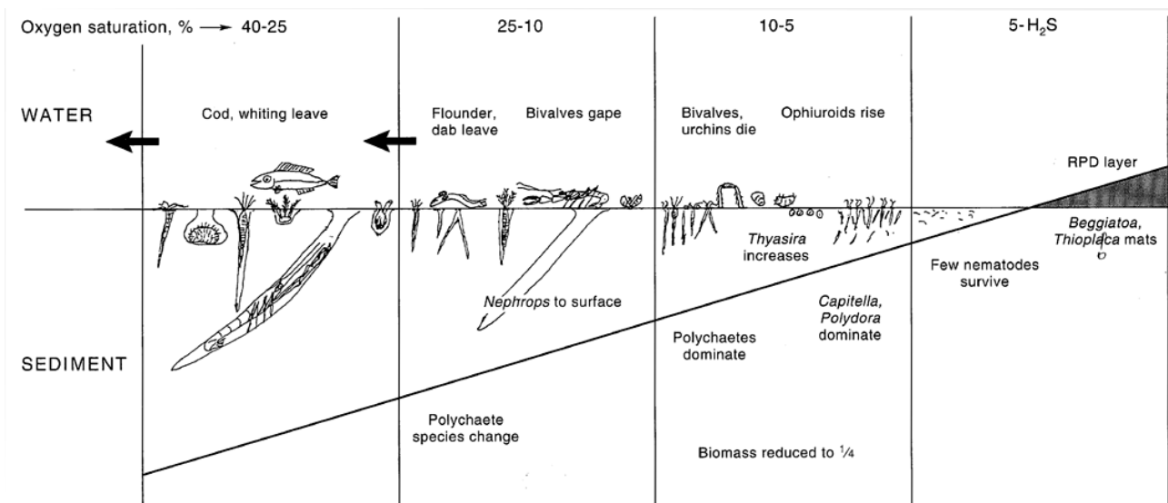
FIG. 7. – General model of benthic epifauna and infauna distribution and behavioural response to a gradient in oxygen saturation. The general change of redox potential discontinuity (RPD) along this gradient is also indicated (from Gray 1992).
