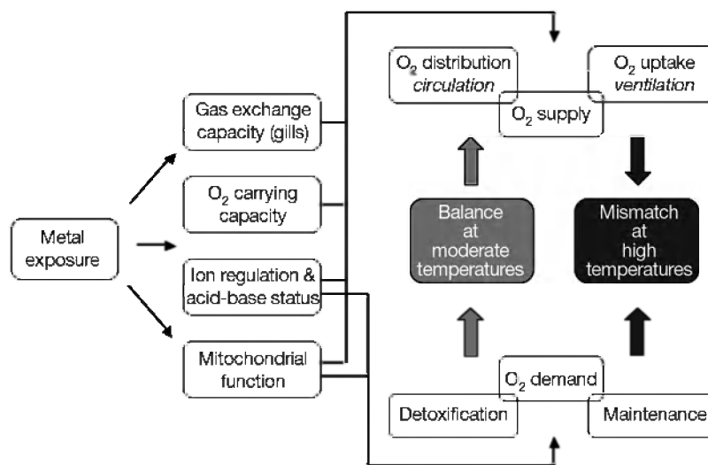
Fig. 4. Generalized physiological model of interactive effects of temperature and trace metals on aquatic ectotherms. Metal exposure interferes with several physiological and biochemical processes that affect aerobic metabolic capacities. At moderate temperatures, the metal-induced rise in oxygen demand can be balanced by a corresponding rise in oxygen supply. At elevated temperatures these effects become detrimental, resulting in a mismatch between oxygen demand and supply mainly due to impaired ventilatory performance (see Sections 3.2 and 4 for details). This model does not cover cases of metabolic rate depression, where acclimation/adaptation to metal exposure occurs by decreasing the rates of metabolic processes and entering a metabolically depressed or dormant state with a concomitant decrease in energy demand and supply. According to the available literature, such situations are rare in metal- and temperature-stressed ectotherms
