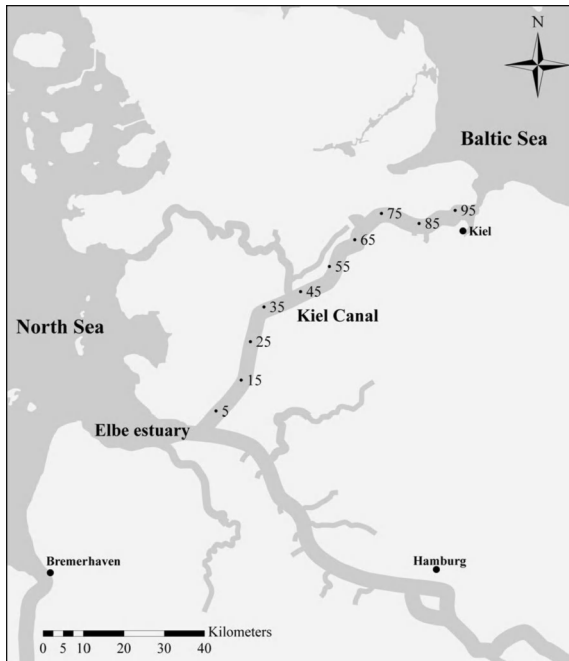
Figure 1. Geographic location of the Kiel Canal, Germany ( 54^{\circ}15'N , 9^{\circ}36'E ). Numbers indicate the canal kilometres.
