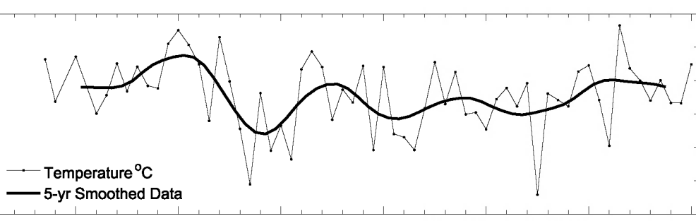
Figure 33. Area 3 – Icelandic waters. Temperature (upper panel) and salinity (lower panel) at 50–150 m at Siglunes Stations 2–4 in North Icelandic waters.
