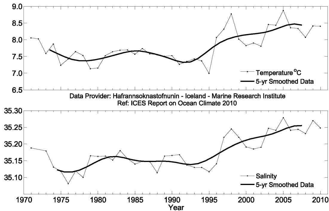
Figure 34. Area 3 – Icelandic waters. Temperature (upper panel) and salinity (lower panel) at 0–200 m at Selvogsbanki Station 5 in South Icelandic waters.
