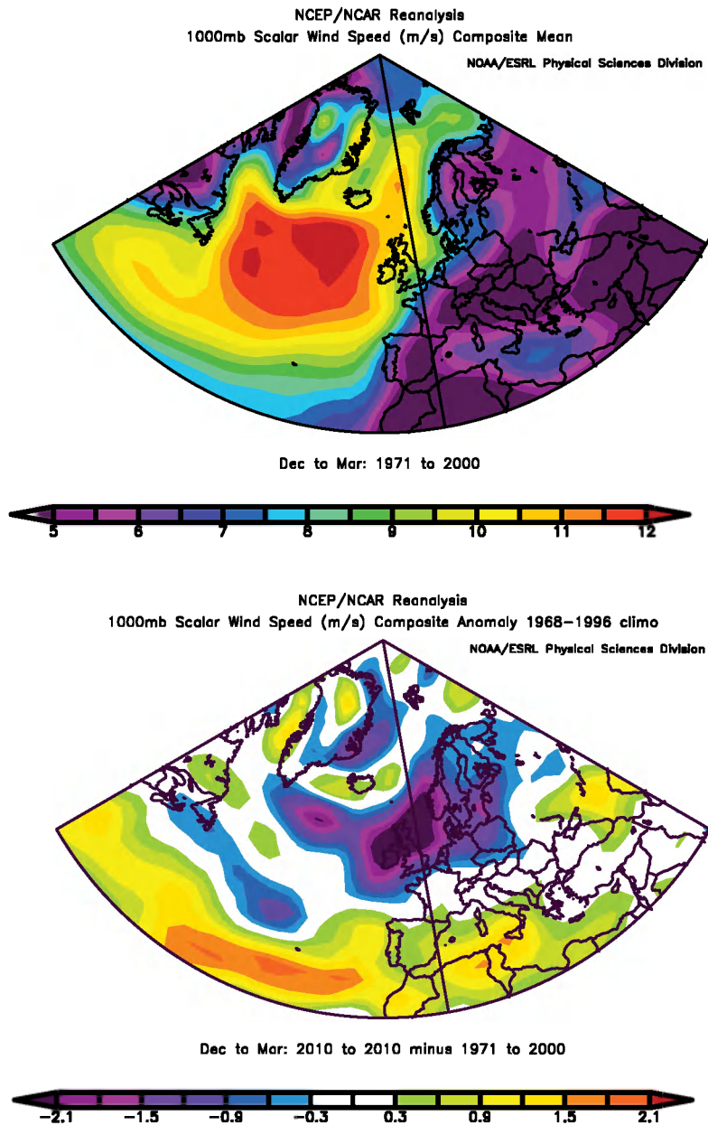
Figure 11. Winter (DJFM) surface windspeed. Upper panel: surface windspeed averaged over 30 years (1971–2000). Lower panel: winter 2010 anomaly in surface windspeed. Images provided by the NOAA/ESRL Physical Sciences Division, Boulder, CO (available online at http://www.cdc.noaa.gov/ ).
