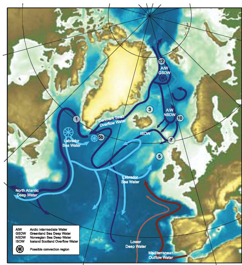
Figure 73. Schematic circulation of the intermediate to deep waters in the Nordic seas and North Atlantic.
