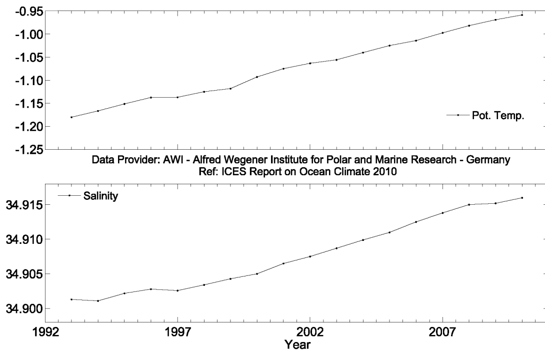
Figure 75. Area 12 – Greenland Sea and Fram Strait. Temperature (upper panel) and salinity (lower panel) at 3000 m in the Greenland Sea Section at 75°N.
