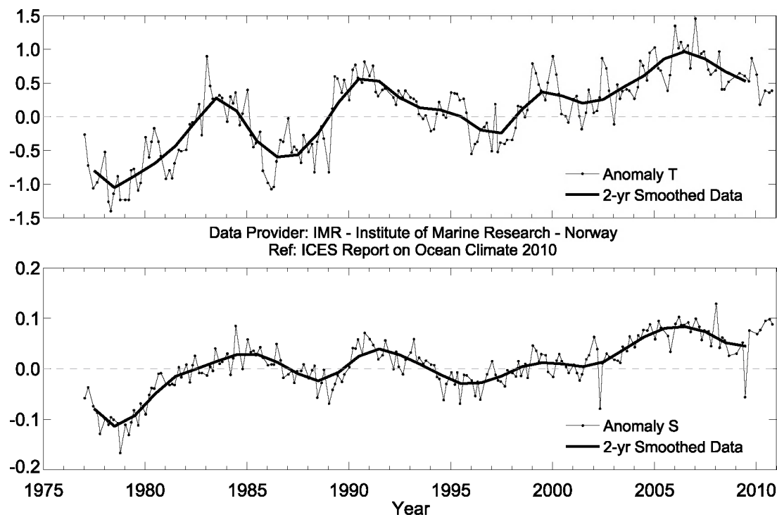
Figure 68. Area 11 – Barents Sea. Temperature anomaly (upper panel) and salinity anomaly (lower panel) in the Fugloya–Bear Island Section.
