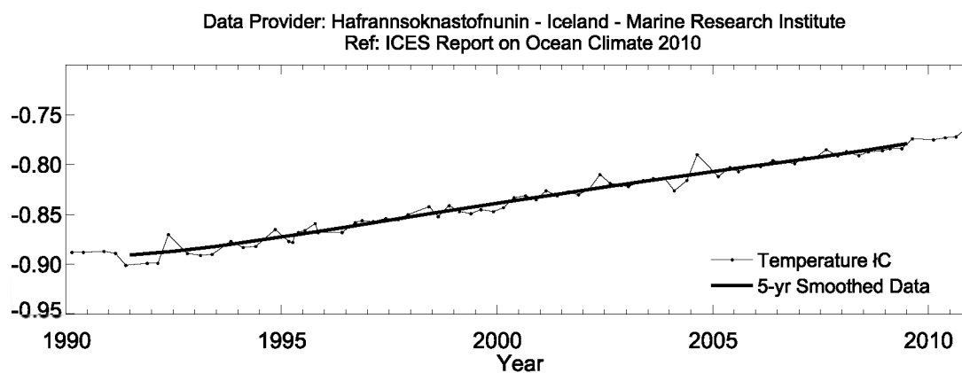
Figure 76. Area 3 – Icelandic waters. Temperature at 1500–1800 m in the Iceland Sea (68°N 12.67°W).
