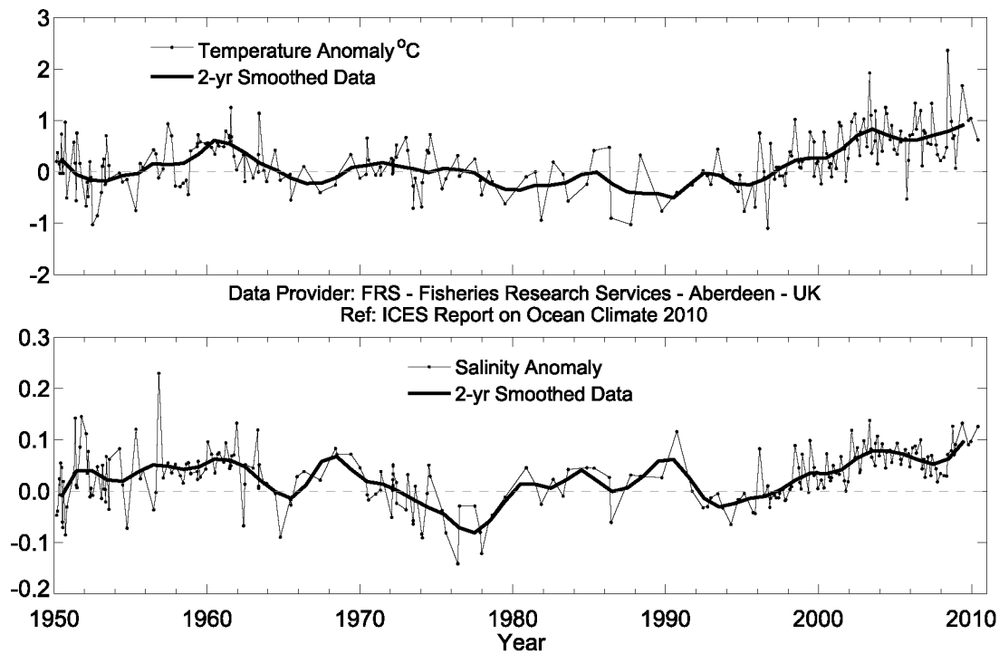
Figure 52. Areas 6 and 7 – Faroe–Shetland Channel. Temperature anomaly (upper panel) and salinity anomaly (lower panel) in the Modified North Atlantic Water entering the Faroe–Shetland Channel from the north after circulating around the Faroe Islands.
