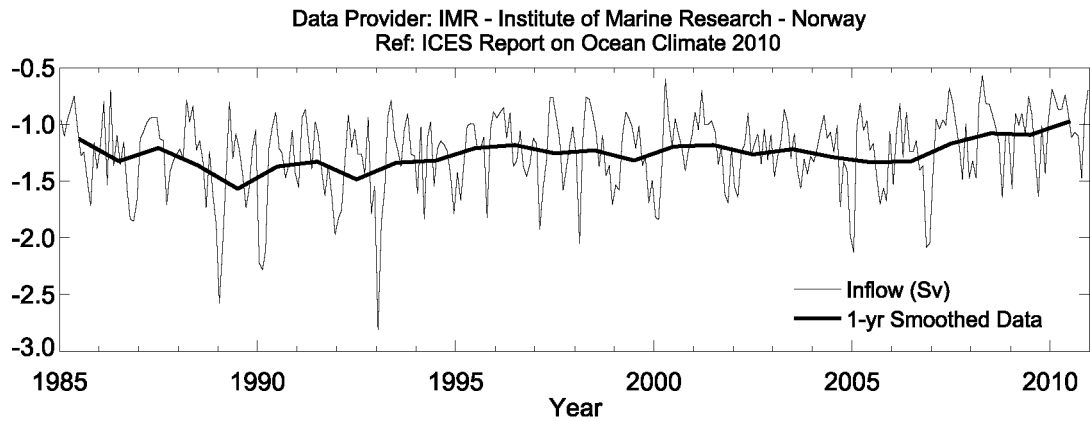
Figure 53. Area 8 – Northern North Sea. Modelled annual mean (bold) and monthly mean volume transport of Atlantic Water (AW) into the northern and central North Sea southwards between the Orkney Islands and Utsire, Norway (top panel). Temperature (middle panel) and salinity (bottom panel) near the seabed in the northwestern part of the North Sea (Location A) and in the core of AW at the western shelf edge of the Norwegian Trench (Location B) during summers 1970–2007.
