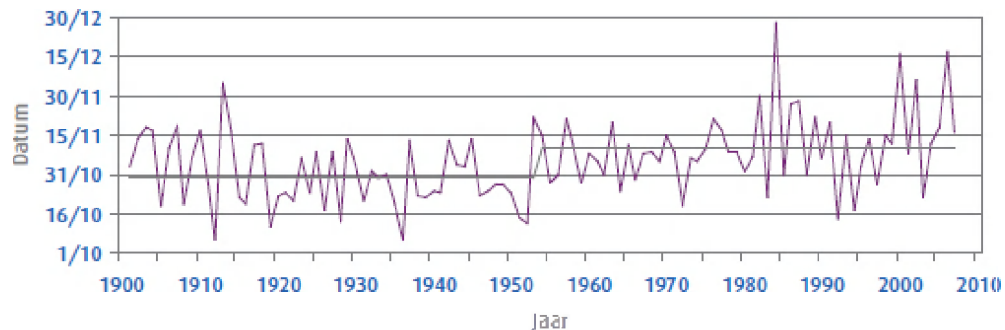
Figure 6 Date of first frost day (minimum temperature below 0 °C) at the beginning of winter in Uccle between 1901 and 2007 (KMI, 2009)
