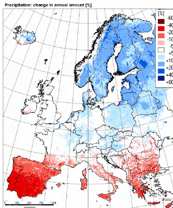
Figure 3 Change in mean annual precipitation by the end of this century (European Commission, 2007)
