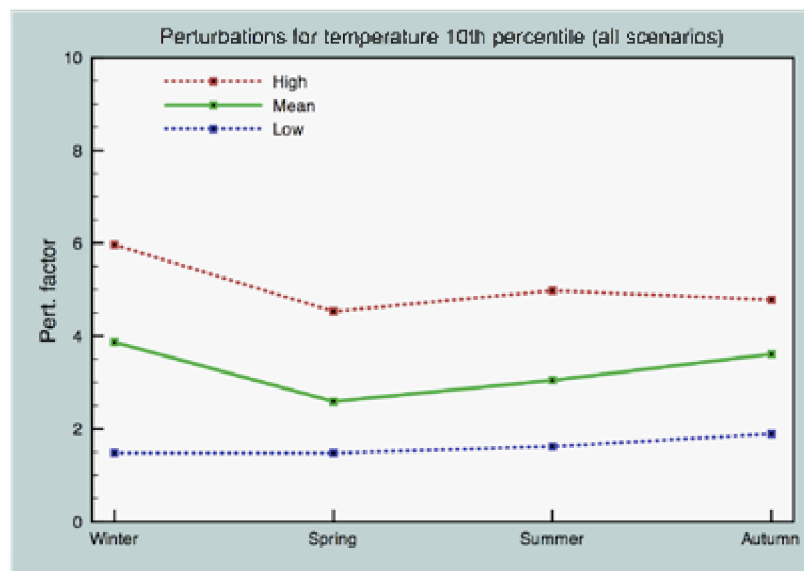
Figure 8 Increase in the 10% percentile of the monthly average temperature at Ukkel for CCI-HYDR climate scenarios, reference period from 1961-1990 and scenario period from 2071-2100 (Baguis et al., 2009)
