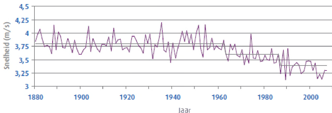
Figure 18 Annual average wind speed at Sint-Joost-ten-Node/Ukkel during the period 1880-2007 (in m/s) (KMI, 2009)
