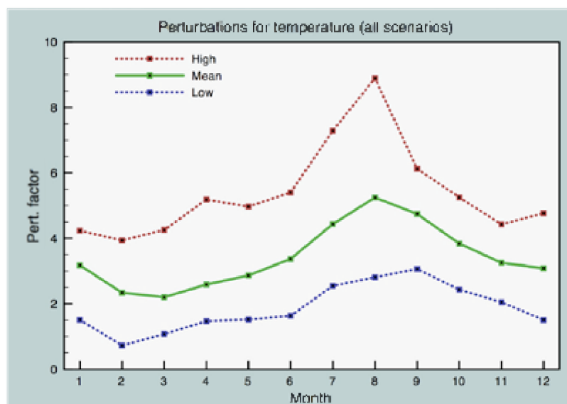
Figure 7 Increase in average monthly temperatures in Uccle for the CCI -HYDR climate scenarios, reference period 1961-1990 to the scenario period 2071-2100 (Baguis et al., 2009)
