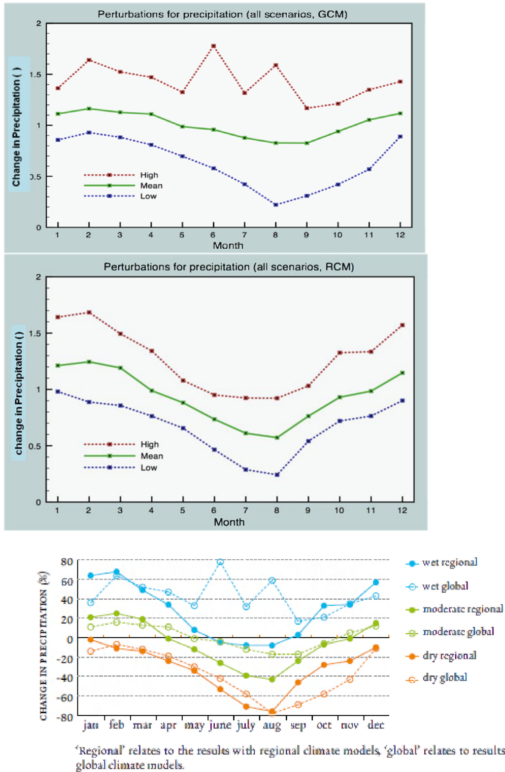
Figure 12 Relative change in monthly rainfall at Uccle for CCI-HYDR climate scenarios for GCM and RC, reference period 1961-1990 and scenario period 2071-2100 (2 top figures Baguis et al. 2009, last figure Brouwers et al. 2009)
