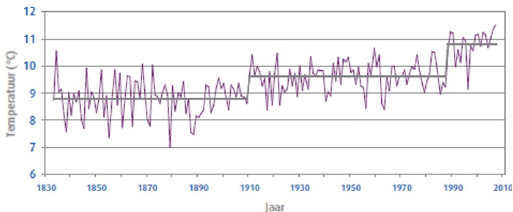
Figure 4 Average annual temperature (in ° C) at Ukkel from 1833-2007. The red curve shows the annual values and the black horizontal lines shows the different periods of relative stability for each period (KMI, 2009)
