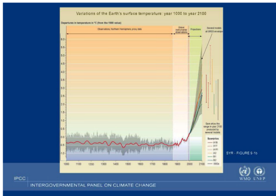
Figure 1 Evolution of the average world temperature between 1000 and 2100 (IPCC, 2001c)
