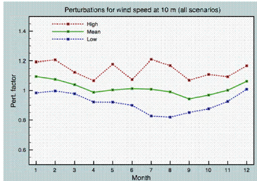
Figure 19 CCI-HYDR based climate scenarios for monthly average wind speed to Ukkel scenario in the period 2071-2100 (Baguis et al., 2009)
