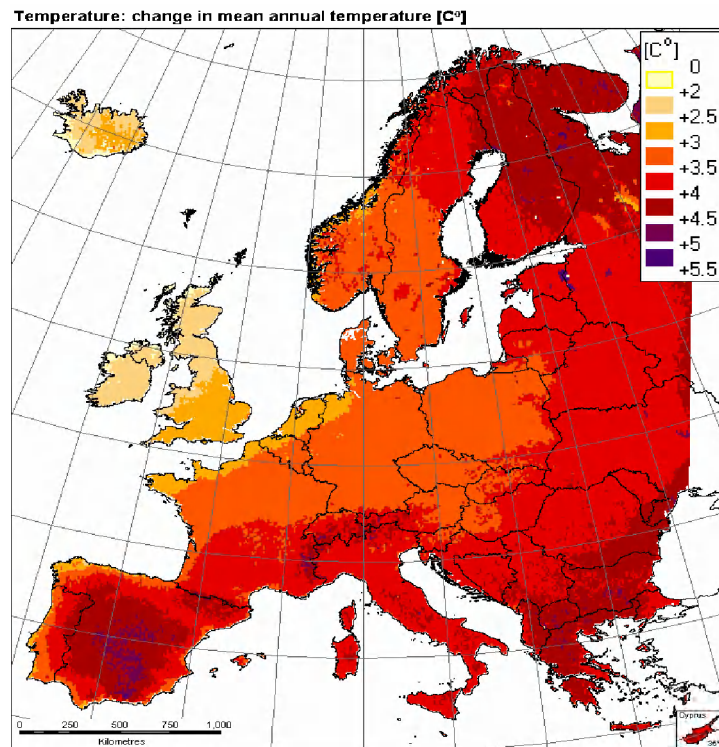
Figure 2 Change in mean annual temperature by the end of this century (European Commission, 2007)
