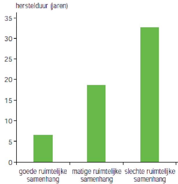
Figure 28 The link between connectivity (bad, moderate and good) and recovery time (in years) after a disturbance (Foppen et al, 1999).
