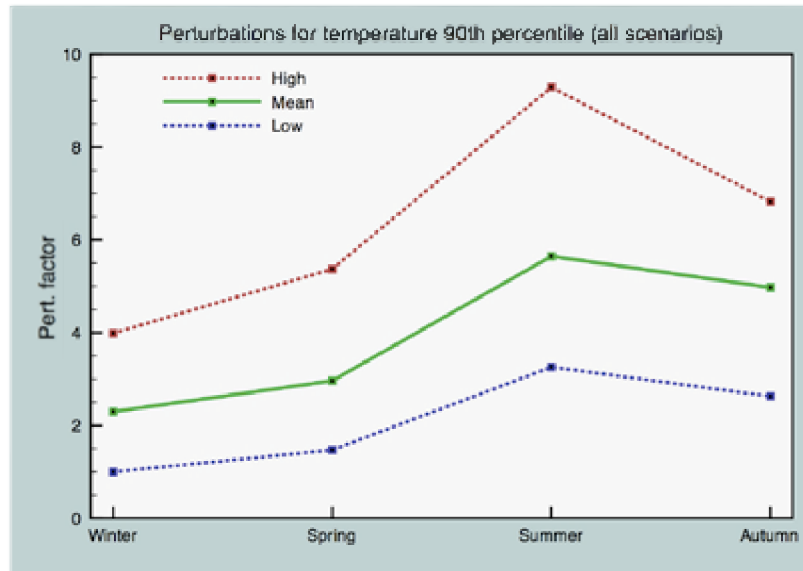
Figure 9 Increase in the 90% percentile of the monthly average temperature at Ussel for CCI-HYDR climate scenarios, reference period 1961-1990 and scenario period 2071-2100 (Baguis et al., 2009)
