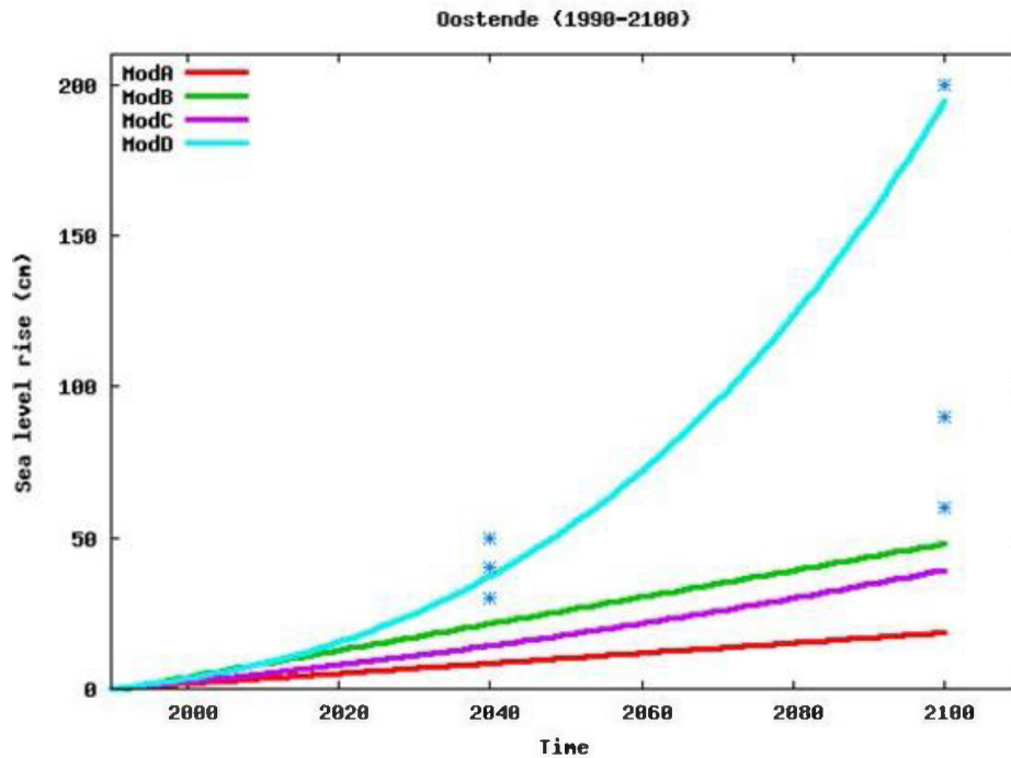
Figure 17 Extrapolation of rising sea levels based on different relationships to Oostende. Model A-Linear relationship, Model B – Stepwise linear, Model C – Second degree polynomial and Model D – third degree polynomial (Ozer et al., 2008)
