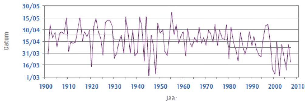
Figure 5 Date of last frost day (minimum temperature below 0 °C) at the end of winter in Uccle between 1901 and 2007(KMI, 2009)
