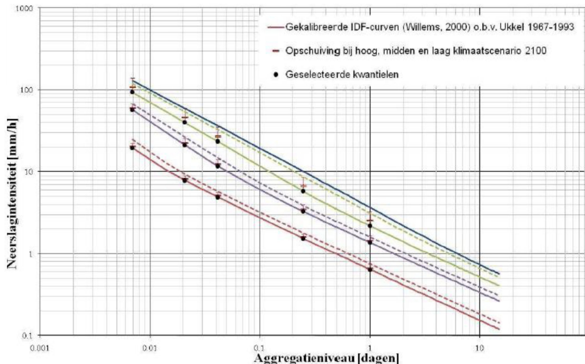
Figure 13 Influence of climate change on IDF curves (Brouwers et al. background document, 2009)
