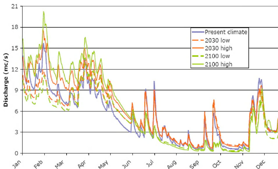
Figure 24 Comparison of the discharge predicted by the calibrated WetSpa model assuming different climate scenarios and the same land-use map
