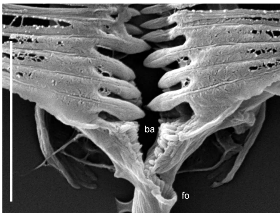
Fig. 4. Testudinella zhujiangensis sp. n., scanning electron microscope photograph of trophi. Detail of major teeth and proximal part of fulcrum, frontal view. Scale bar: 10 µm. ba: basal apophysis, fo: fulcrum opening
