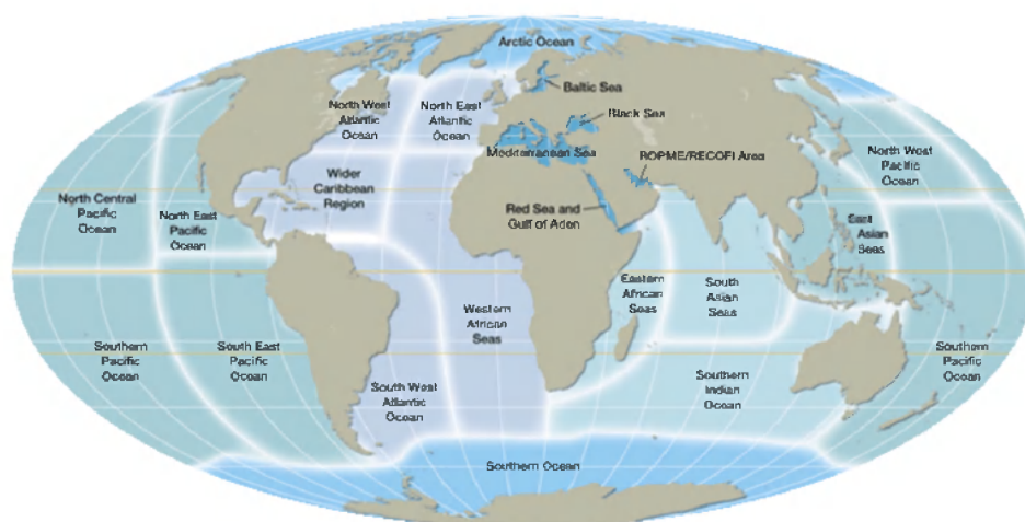
Fig. 2. Ocean regions considered in the Assessment of Assessments
