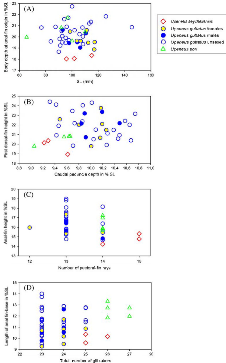
Figure 2. Body depth at anal-fin origin against SL (A), first dorsal-fin height against caudal-peduncle depth (B), anal-fin height against number of pectoral-fin rays (C), and length of anal-fin base against total number of gill rakers (D), in the three Western Indian Ocean species of the japonicus group (morphometric variables expressed in % SL).
