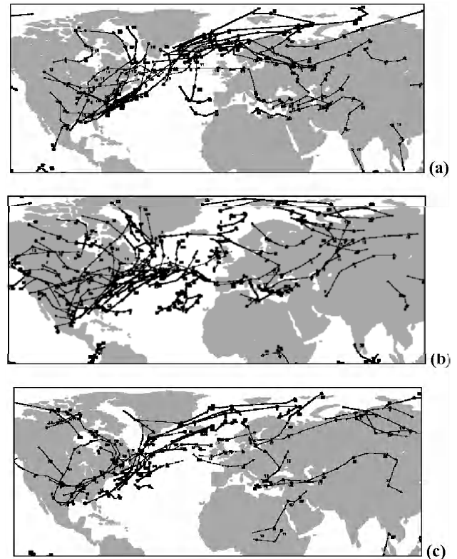
Figure 4. Typical January storm tracks for the “+1” year of the each type of El Niño on the example of the pair of events: (a) spring type – 1977, 1995; (b) summer-autumn long type – 1969, 1987; (c) summer-autumn short type – 1983, 1998.
