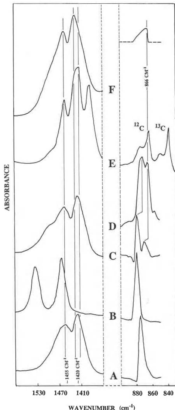
Fig. 4. FTIR spectra of \text{CO}_3^{2-} vibrational bands in carbonate-fluorapatite samples. (A) type B carbonate hydroxylapatite; (B) type A carbonate hydroxylapatite; (C) hydroxylapatite without the usual type A location band at 1540 \text{cm}^{-1} but with an 878- \text{cm}^{-1} band; (D) a fluoridation experiment showing the \nu_2 \text{CO}_3^{2-} vibrational band shift; (E) synthetic apatite from the present study; (F) marine carbonate-fluorapatite from the present study. See text for a complete description. Data for curves A–D are from Rey et al. (1989).
