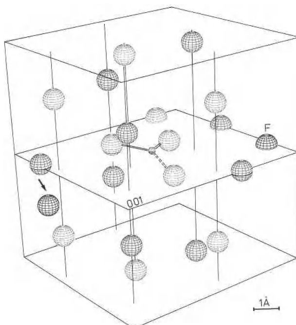
Fig. 9. Apatite molecular cluster after the replacement of \text{PO}_4^{3-} by \text{CO}_3\text{F}^{3-} (crystal orientation as indicated in Fig. 8). O = open spheres, Ca = shaded spheres, F is represented by the letter F, and the C atom = the small sphere. Note the interstitial position for F (thick arrow).
