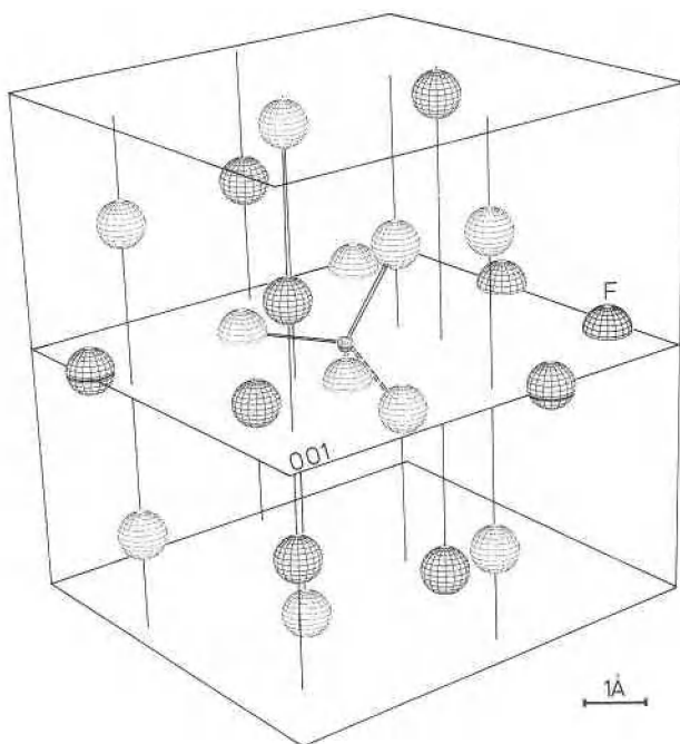
Fig. 8. Apatite molecular cluster centered around a fully optimized \text{PO}_4^{3-} ion. The nonphosphate atoms are generalized points of fractional charge, making up a net positive charge of +3 that balances the negative charge of the \text{PO}_4^{3-} ion. The vertical lines are parallel to the screw axis of the mineral and perpendicular to the (001) plane. O = open spheres, Ca = shaded spheres, F is represented by the letter F, and the P atom = the small sphere.
