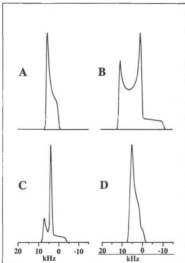
Fig. 7. (A) The simulated static-echo spectrum of a C atom in \text{CO}_3^{2-} in a planar equilateral triangle with no dipole interaction. (B) The simulated static-echo spectrum of a C atom in \text{CO}_3^{2-} , with F at a distance of 1.38 Å. Both the chemical-shift anisotropy of a pure carbonate and the dipolar interaction between C and F are considered. The F is assumed to lie on a line that runs through the C atom in a carbonate group and is perpendicular to the plane of the \text{CO}_3^{2-} ion. (C) The simulated spectrum with the distance of 2.00 Å between C and F. (D) The simulated spectrum with the distance of 3.00 Å between C and F. A Gaussian line broadening of 500 Hz was applied to each spectrum.
