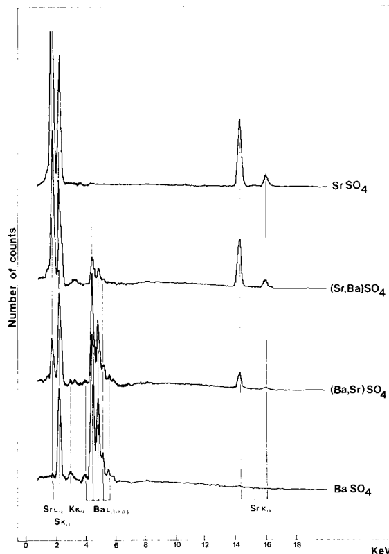
Fig. 4. Energy-dispersive spectra of barite, celestite and intermediate solid solutions, as observed in oceanic suspended matter samples. Vertical scales are arithmetic, but are normalized for the \text{Sr-K}_{\alpha} peak which represents 58,000 counts. Horizontal scale: energies of the X-rays in keV.
