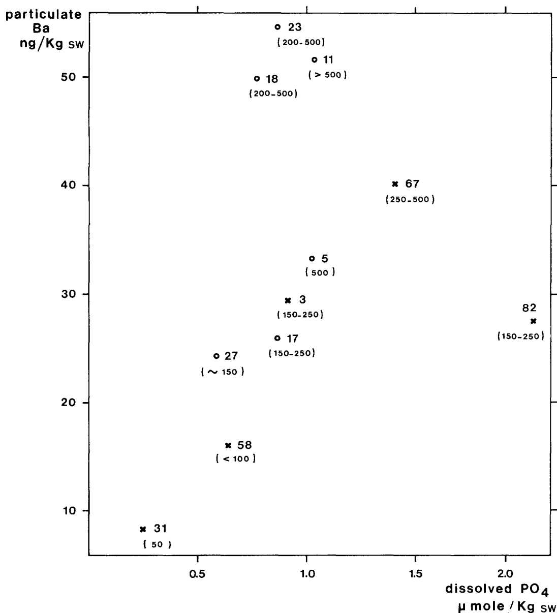
Fig. 10. Total Ba_p versus dissolved PO_4 . The geometric mean Ba_p value (in ng/kg sw), observed between 150 and 1000 m is plotted against the geometric mean dissolved PO_4 value (in \mu mole/kg sw; GEOSECS ship-board data) for the same depth interval. Crosses refer to Ba_p measurements performed by INAA at the Centre des Faibles Radioactivités; open circles refer to measurements performed by INAA at the Woods Hole Oceanographical Institution by P. Brewer (GEOSECS shore-based data). Numbers refer to GEOSECS station numbers. Between brackets: values of organic carbon production rates (in mg C/m 2 day) from Koblentz-Mishke [44]; value for station 31 from Steeman-Nielsen [41].
