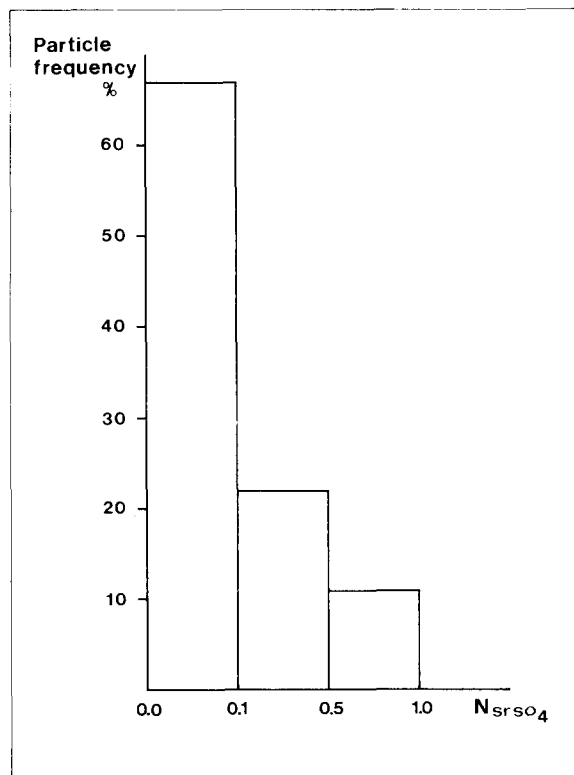
Fig. 3. Frequency histograms of (\text{Ba}, \text{Sr})\text{SO}_4 and (\text{Sr}, \text{Ba})\text{SO}_4 particles as a function of their \text{SrSO}_4 fraction ( N_{\text{SrSO}_4} ), for the sample from 200 m, GEOSECS station 58. We take N_{\text{SrSO}_4} + N_{\text{BaSO}_4} = 1 . Data obtained by P. Buat-Menard and C. Jehanno at the Centre des Faibles Radioactivités, Gif-sur-Yvette.
