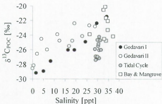
Figure 15 : Carbon isotope composition of suspended organic matter along the Gautami Godavari salinity gradient (both transects considered separately) and in the mangrove creeks and Kakinada Bay (note that no data are available for most of the Bay stations, see Table 3).
