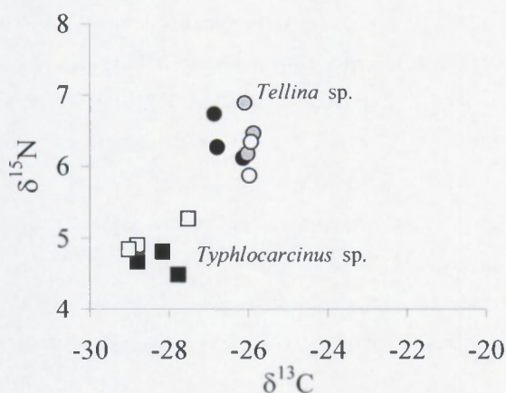
Figure 9 : Carbon and nitrogen isotopic composition of individual Tellina sp. (circles) and Typhlocarcinus sp. (squares) from the three mangrove creek locations. Black symbols : CO, grey symbols : GA, open symbols : LH.
