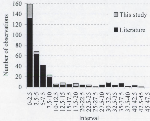
Figure 4 : Distribution of data on the organic carbon content (% on dry weight basis) of intertidal mangrove sediments from published literature (black bars) and this study (grey bars). Total number of data is 358. Literature sources, in alphabetical order : Alongi (1996), Alongi et al. (1993, 1999, 2000a, b, 2001), Chen & Twilley (1999), Dittmar & Lara (2001), Gillikin (2001), Hemminga et al. (1994), Jennerjahn & Ittekkot (1997, 2002), Kazungu (1996), Kristensen et al. (1988, 1992, 2000), Lacerda et al. (1995), Lallier-Verges et al. (1998), Matsui (1998), McKee et al. (2002), Middelburg et al. (1996), Mfilinge et al. (2002), E. Olafsson & M. Skov (unpublished data), Perrussel et al. (1999), Twilley et al. (1997), Holmer et al. (2001), Woodroffe (1985).
