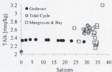
Figure 4: Variations in Total Alkalinity along the Gautami Godavari salinity gradient and in the mangrove creeks and Kakinada Bay during the pre-monsoon period of 2001.
