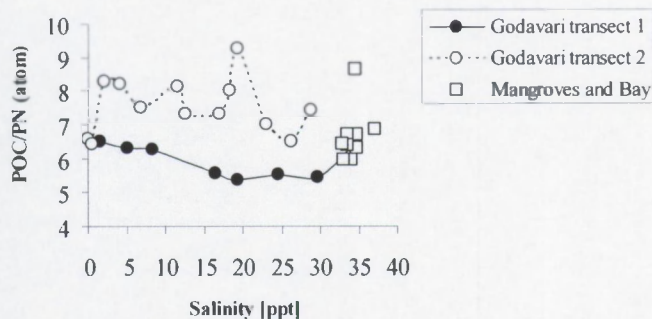
Figure 13 : Elemental composition (POC/PN) of suspended organic matter along the Gautami Godavari salinity gradient and in the mangrove creeks and Kakinada Bay (note that not data are available for most of the Bay stations nor for the diurnal cycle, see Table 3 and 4).
