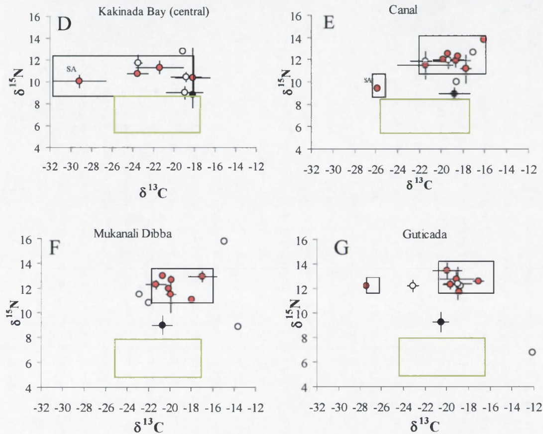
Figure 1 (continued): \delta^{13}\text{C} - \delta^{15}\text{N} plot of fish species collected at various locations in the Coringa Wildlife Sanctuary and adjacent Kakinada Bay during post-monsoon of 1999 (see Chapter 6 for location of sites). Black symbols : lower trophic level benthic invertebrates sampled during the same period at the specified site (data from Chapter 6), red symbols : benthic invertebrate feeding fish, and open symbols : fish with other or unknown feeding habits. The green square represents the stable isotope signature for most intertidal invertebrates (see Chapter 8). SA : Scatophagus argus . Error bars = 1 s.d.
