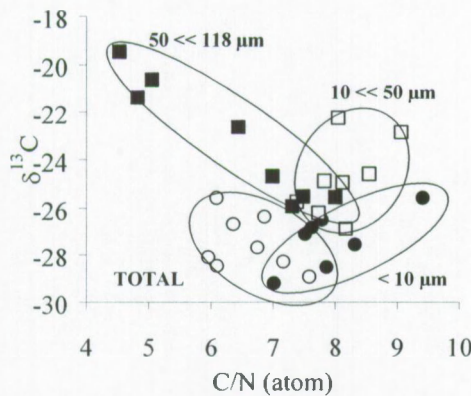
Figure 4 : Elemental composition (C/N, atom) versus \delta^{13}\text{C} of total and size-fractionated suspended organic matter. Open circles : total SPOM, open squares : 10 << 50 \mu\text{m} , black circles : < 10 \mu\text{m} , and black squares : 50 << 118 \mu\text{m} . Note that the ellipses merely serve to group data of the same size class.
