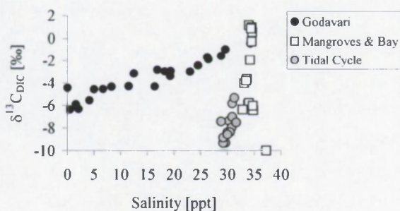
Figure 8 : Variations in the carbon isotope composition of the DIC pool along the Gautami Godavari salinity gradient and in the mangrove creeks and Kakinada Bay during the pre-monsoon period of 2001.
