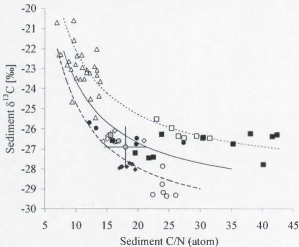
Figure 1 B : \delta^{13}\text{C} (in ‰) of sediment organic carbon versus C/N (atom) ratios of sediments from various mangrove ecosystems. Symbols as in Fig 1A. Error bars : 1 s.d. Different curves correspond to different assumptions for \delta^{13}\text{C} , organic carbon content, and C/N ratios for the two end-members (see text for details).
