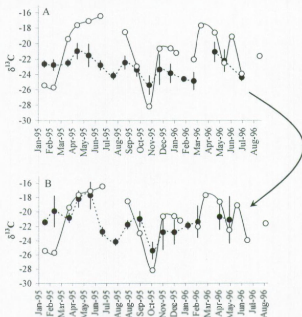
Figure 9 : (A) \delta^{13}\text{C} of POC (full circles) in Kakinada Bay and zooplankton (open circles) at station K 2 , and (B) \delta^{13}\text{C} of zooplankton at station K 2 (open circles) and estimated \delta^{13}\text{C} of phytoplankton in Kakinada Bay (full circles). Error bars indicate \pm 1 s.d.
