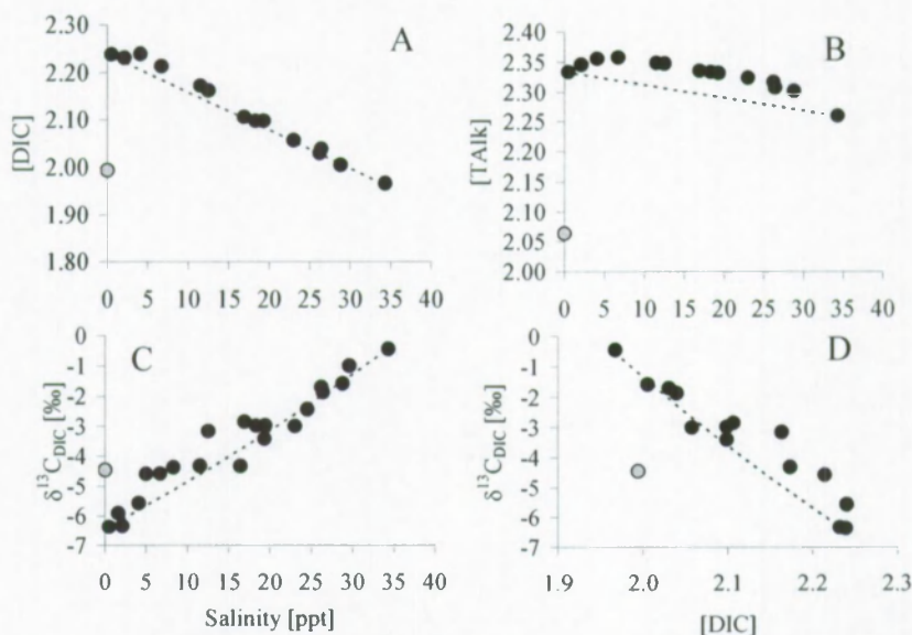
Figure 20 : Plot of (A) DIC concentrations versus salinity, (B) TAlk versus salinity, (C) \delta^{13}\text{C} of the DIC pool versus salinity, and (D) \delta^{13}\text{C}_{\text{DIC}} versus DIC concentrations for the Godavari samples (black symbols) and the sample from zero salinity at Dowleswaram Dam (grey symbol). Dotted curve represents conservative mixing.
