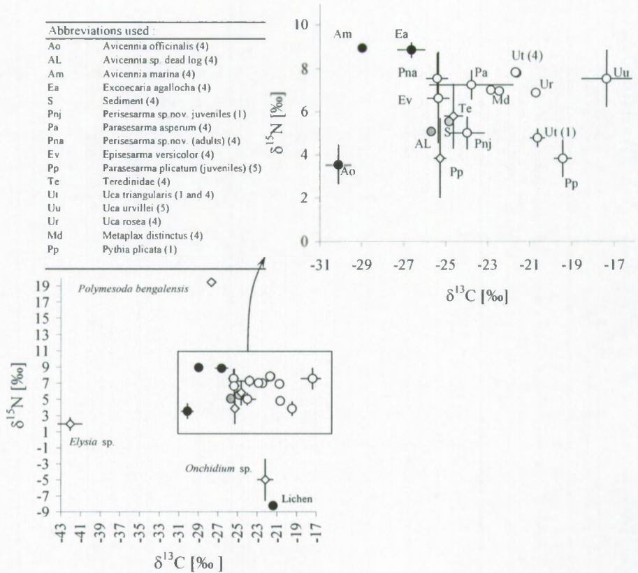
Figure 3 : Plot of \delta^{15}\text{N} versus \delta^{13}\text{C} for different primary producers, sediments, crustaceans and gastropods collected at different sites the intertidal mangrove forest of the Coringa Wildlife Sanctuary in May-June 2001. Abbreviations as in legend. Numbers between brackets refer to sampling sites, see Figure 1.
