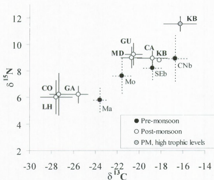
Figure 8 : Plot of \delta^{13}\text{C} and \delta^{15}\text{N} data for benthic invertebrates collected during post-monsoon period (open symbols : lower trophic levels, grey symbol : higher trophic level species), and a comparison with pre-monsoon data (only data for lower trophic level species are shown, black symbols). Abbreviations as in Figures 1 and 3. Error bars = 1 s.d.
