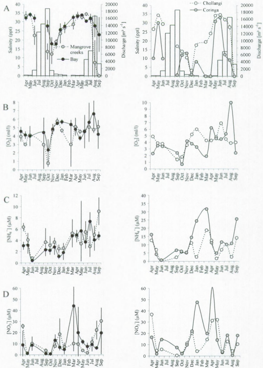
Figure 7 : Some physico-chemical parameters from mangrove creek locations (GA, Gc III, and LH), Bay locations (MD, GU, KB, KBN, and BB), and for two other creeks, Chollangi and Coringa between april 2000 and September 2001. See Chapter 4 for location of sampling stations. White bars on panel A (right-hand Y-axis) represent discharge rate of the Godavari at Dowleswaram Dam. Note the difference in Y-axis for panel B and C.
