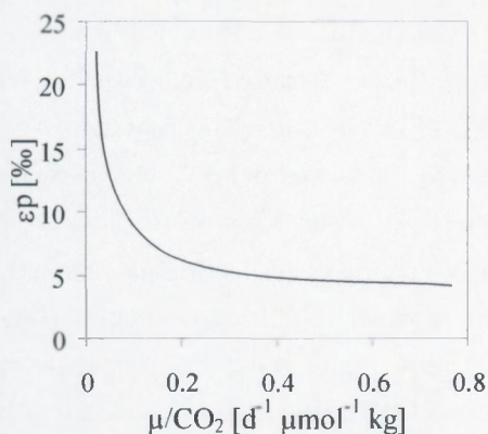
Figure 2 : Fitted curve through a compilation of field and laboratory data of stable isotope fractionation ( \epsilon_p ), phytoplankton growth rates ( \mu ) and \text{CO}_2 concentrations. Redrawn from Tortell et al (2000).
