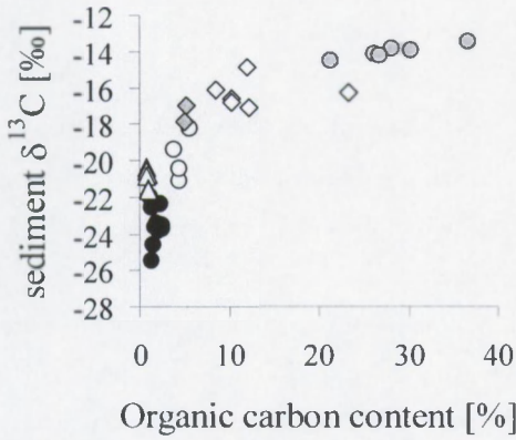
Figure 2 : \delta^{13}\text{C} (in ‰) of organic carbon versus organic carbon content (% dry weight) of surface sediments from various salt marsh ecosystems. Adapted from Middelburg et al. (1997).
