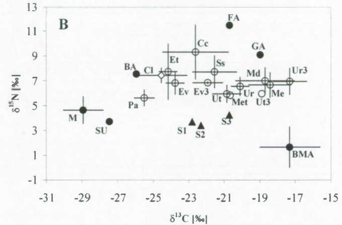
Figure 2 B : Plot of \delta^{15}\text{N} versus \delta^{13}\text{C} for different primary producers, sediments, and crustaceans collected in the intertidal mangrove forest of the Coringa Wildlife Sanctuary in Nov-Dec 1999. Error bars indicate 1 s.d.. BA : brown macroalgae (1), BMA : benthic microalgae (5), Cc : Cardisoma carnifex (8), Cl : Clibanarius longitarsis (6), Et : Episesarma tetragonum (6), Ev : E. versicolor (5 at site 1, 3 at site 3), FA : filamentous algae (1), GA : green macroalgae (1), M : mangrove leaves (17), Md : Metaplex distinctus (9), Me : M. elegans (12), Met : Metopograpsus messor (1), S : Sediment, Pa : Parasesarma asperum (5), Ss : Scylla serrata (7), Su : Suaeda sp. (1), Ur : Uca rosea (3 at each site), Ut : U. triangularis bengali (7 at site 1, 1 at site 3). (n) : number of individuals/samples; numbers on figure refer to sampling sites, if not from site 1 or 2.
