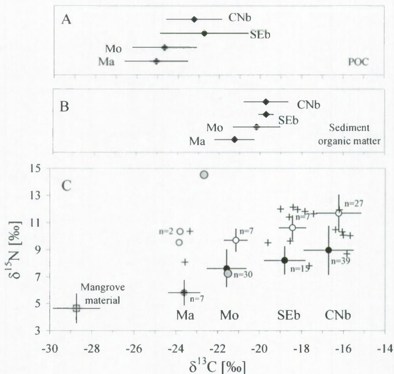
Figure 7 : Average \delta^{13}\text{C} of (A) suspended particulate organic carbon (POC, data from Bouillon et al. 2000 and Dehairs et al. 2000) and (B) sediment organic matter, and (C) \delta^{13}\text{C} - \delta^{15}\text{N} plot for mangrove litter and benthic invertebrates collected in the mangrove creeks (Ma), mangrove outlets (Mo), South-east Bay (SEb), and Central and North Bay (CNb). Closed symbols refer to species presumed to occupy a low trophic level, open symbols refer to species of higher trophic levels, and '+' indicate species of unknown trophic level from all zones. Two penaeid prawns collected in the North Bay with distinctly low \delta^{13}\text{C} values (see discussion) are shown as grey circles. Error bars indicate 1 s.d.
