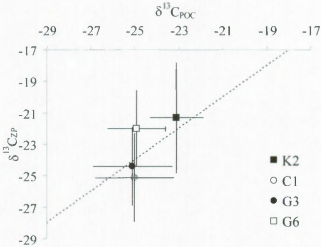
Figure 5 : Average zooplankton \delta^{13}\text{C} (in ‰) versus average POC \delta^{13}\text{C} (in ‰) for different locations. Note that only concurrently collected samples were used to construct this figure. Error bars indicate the standard deviation. The dotted line represents the \delta^{13}\text{C} for the zooplankton food source assuming a trophic fractionation factor of 1 ‰.
