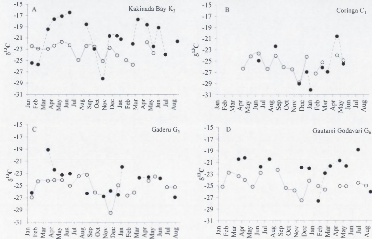
Figure 6 : Seasonal variation of zooplankton \delta^{13}\text{C} (full circles) and POC \delta^{13}\text{C} (open circles) at (a) Kakinada Bay K 2 , (b) Coringa mouth C 1 , (c) central Gaderu G 3 , and (d) mouth of the Gautami Godavari G 6 .
