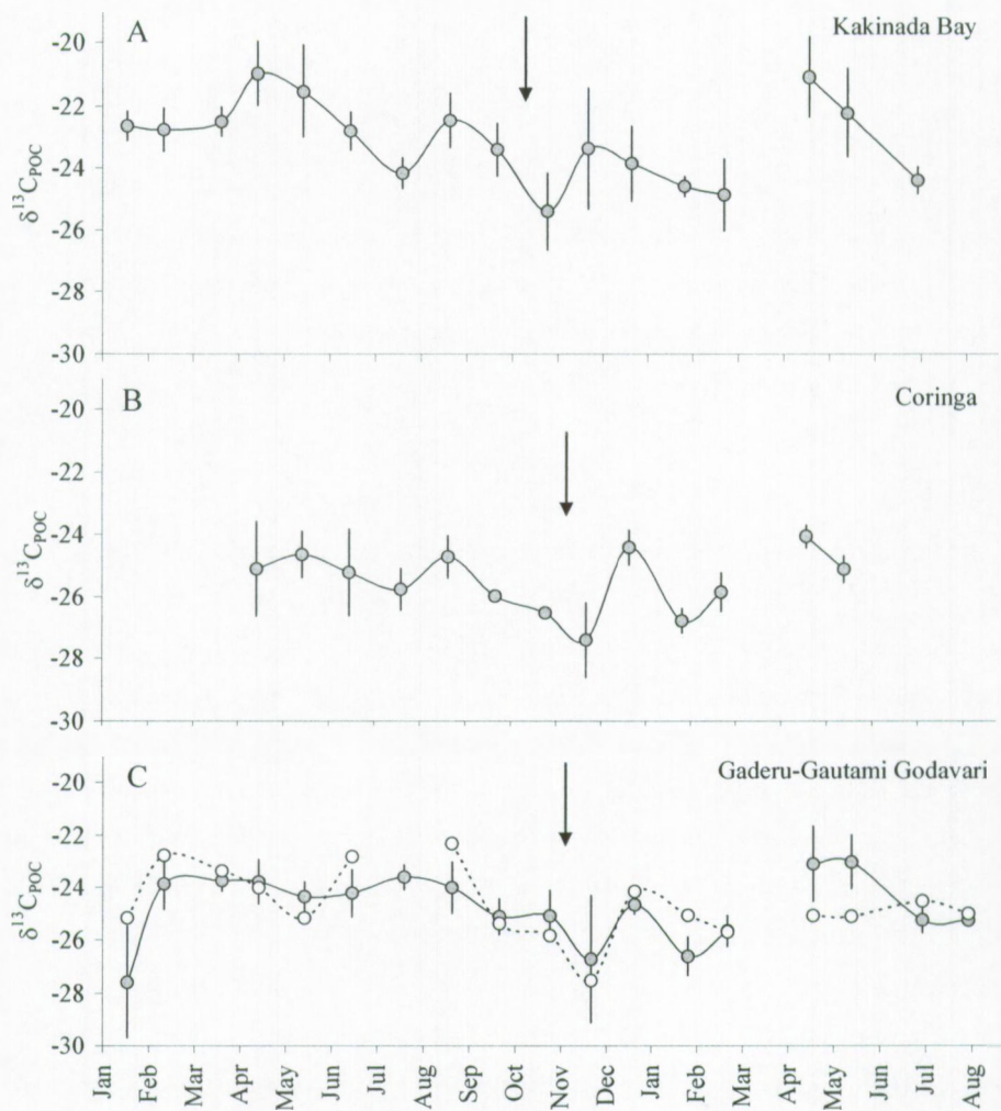
Figure 2 : Seasonal variations of \delta^{13}\text{C} of POC, averaged over different stations in (A) Kakinada Bay, (B) Coringa, and (C) Gaderu (grey circles) and the mouth of Gautami Godavari (open circles). Error bars indicate \pm 1 s.d. Arrow indicates a period in which a general depletion is noted, see text for details.
