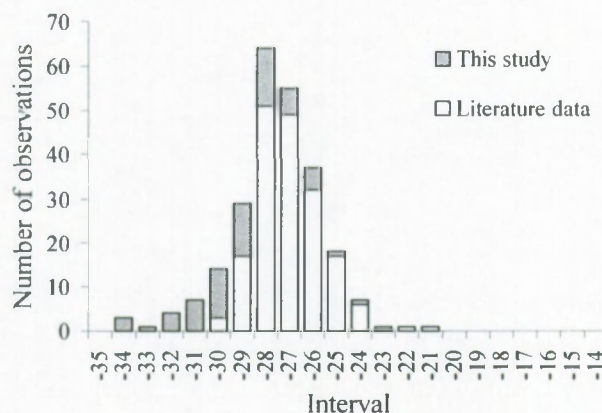
Figure 1 : Distribution of \delta^{13}\text{C} data of mangrove leaf tissue (literature data and this study). The \delta^{13}\text{C} value indicates the upper (i.e. least negative) value of the interval. Note that data from studies explicitly investigating the effect of environmental conditions or nutrient availability are not included.
