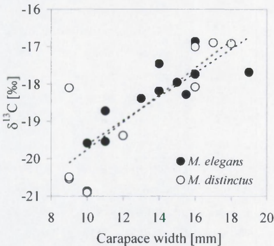
Figure 5 : Relationship between the carbon stable isotopic composition ( \delta^{13}\text{C} , expressed in ‰) and carapax width (mm) for Metaplex distinctus (open circles, R^2 = 0.70 , p < 0.01 ) and M. elegans (black circles, R^2 = 0.66 , p < 0.01 ).
