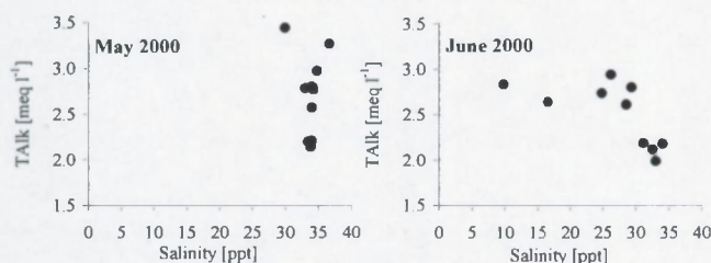
Figure 25 : Examples of the non-conservative behaviour of TALK in the mangrove creeks and Kakinada Bay area. Data for May and June 2000 are shown.
