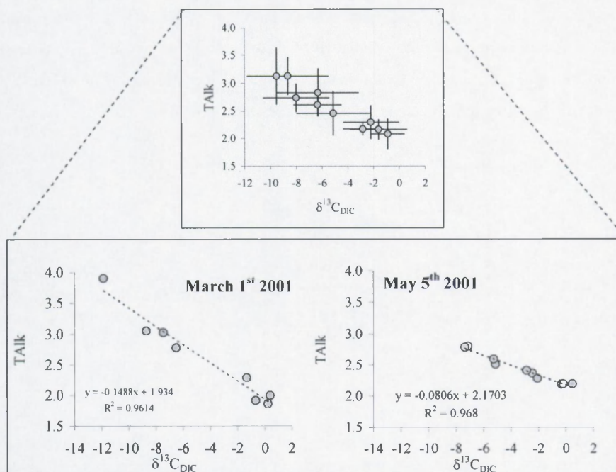
Figure 24 : TALK- \delta^{13}\text{C}_{\text{DIC}} relationship for the 10 sampling stations (see Figure 1) averaged over the entire sampling period (top panel, error bars indicate 1 s.d.) and for March 2001 (steep gradient) and early May 2001 (gradient less steep).
