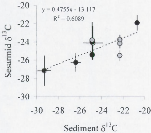
Figure 4 : Relationship between \delta^{13}\text{C} values of sediment organic matter and those of different species of sesamid crabs ( R^2 = 0.61 , p < 0.05 ). Black symbols : this study, grey symbols : data from Rodelli et al. (1984). Sediment data for Galle (Sri Lanka) were taken from Bouillon et al. (in review, i.e. Chapter 7). Error bars indicate 1 s.d.
