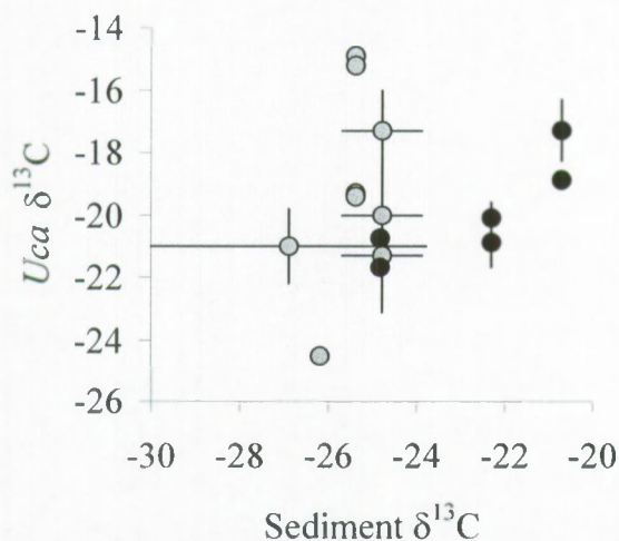
Figure 6 : Relationship between \delta^{13}\text{C} values of sediment organic matter and those of different species of fiddler crabs, Uca spp. Black symbols : this study, grey symbols : data from literature sources (Fry 1984, Rodelli et al. 1984, France 1998, Hsieh et al. 2002). Error bars indicate 1 s.d.
