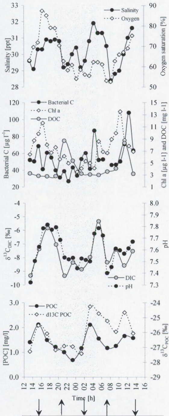
Figure 16 : Diurnal variations (at hourly or two-hourly resolution) of the stable carbon isotope composition of the DIC pool, pH, salinity, oxygen saturation state, bacterial C stock, Chlorophyll a concentration, DOC concentration, POC concentration, and stable carbon isotope composition of the POC pool at Gaderu creek (see Figure 1B for location). Grey-shaded area represents night time. Arrows pointing upward represent approximate high tide, arrows pointing downward represent approximate low tide.
