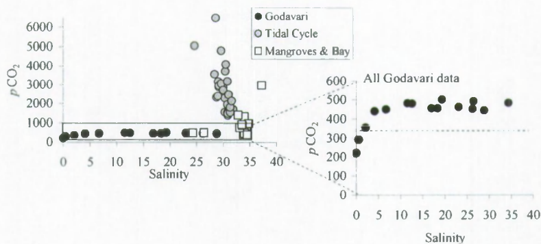
Figure 6 : Variations in the partial pressure of \text{CO}_2 (expressed in ppm) along the Gautami Godavari salinity gradient (enlarged section) and in the mangrove creeks and Kakinada Bay during the pre-monsoon period of 2001. Dotted line in insert represents equilibrium with the atmosphere.
