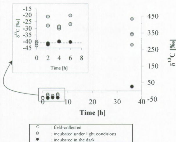
Figure 1 : \delta^{13}\text{C} values of field-collected Elysia coringaensis sp. nov. (June 2001), and evolution of \delta^{13}\text{C} during incubation under light or dark conditions in the presence of ^{13}\text{C} -labeled \text{NaHCO}_3 .
