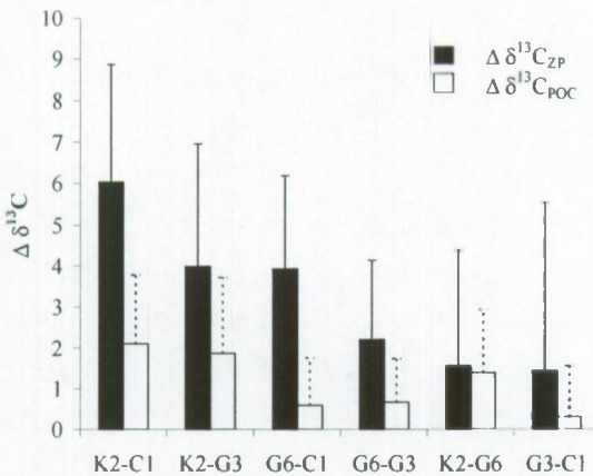
Figure 7 : Average difference in zooplankton \delta^{13}\text{C} (black bars) and average difference in POC \delta^{13}\text{C} (white bars) for different pairs of locations. Error bars = 1 s.d.
