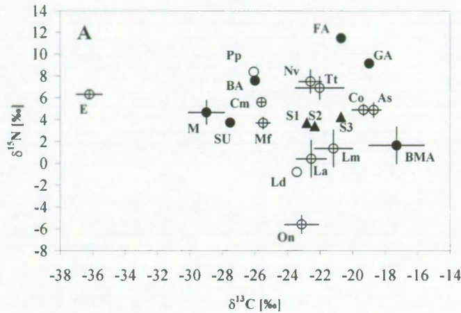
Figure 2 A : Plot of \delta^{15}\text{N} versus \delta^{13}\text{C} for different primary producers, sediments, and gastropods collected in the intertidal mangrove forest of the Coringa Wildlife Sanctuary in Nov-Dec 1999. Error bars indicate 1 s.d.. As: Assiminea sp. (6), BA: brown macroalgae (1), BMA: benthic microalgae (5), Cm: Cassidula mustelina (2), Co: Cerithidea obtusa (6), E: Elysia coringaensis sp. nov. (10), FA: filamentous algae (1), GA: green macroalgae (1), La: Littoraria articulata (5), Ld: Littoraria delicatula (2), Lm: Littoraria melanostoma (6), M: mangrove leaves (17), Mf: Melampus fasciatus (6), Nv: Neritina violacea (6), On: Onchidium sp. (7), Pp: Pythia plicata (2), S: Sediment, SU: Suaeda sp. (1), Tt: Telescopium telescopium . (n) : number of individuals/samples; numbers on figure refer to sampling sites, if not from site 1 or 2.
