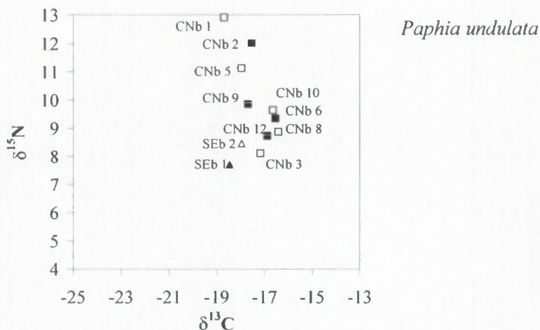
Figure 10 (see also previous page): \delta^{13}\text{C} - \delta^{15}\text{N} plot for (A) Typhlocarcinus sp., (B) Tellina spp., and (C) Paphia undulata sampled at different locations throughout the study area (see Fig 1 for location of stations).
