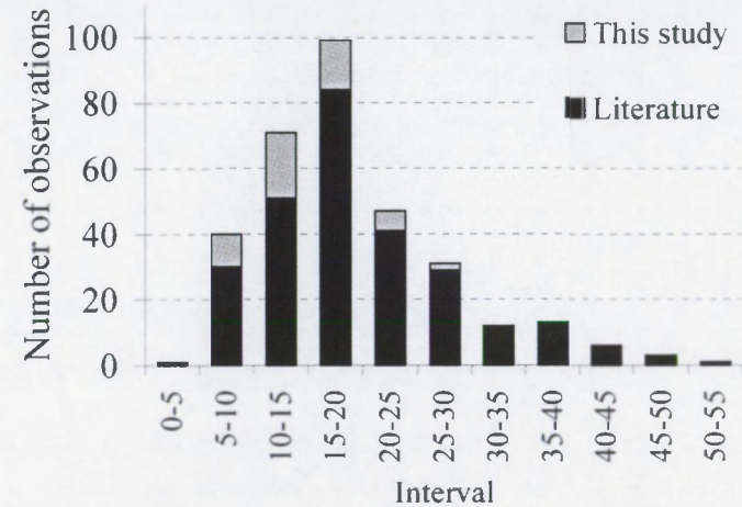
Figure 5 : Distribution of data on the elemental composition (C/N, atom) of organic matter in intertidal mangrove sediments from published literature (black bars) and this study (grey bars). Total number of data is 324. Literature sources, in alphabetical order : Alongi (1996), Alongi et al. (1993, 1999, 2000a, b), Chen & Twilley (1999), Dittmar & Lara (2001), Gillikin (2001), Jennerjahn & Ittekkot (1997, 2002), Kazungu (1996), Kristensen et al. (1988, 1992, 2000), Lacerda et al. (1995), Lallier-Verges et al. (1998), McKee et al. (2002), Middelburg et al. (1996), Mfilinge et al. (2002), E. Olafsson & M. Skov (unpublished data), Perrussel et al. (1999), Twilley et al. (1997), Holmer et al. (2001), Woodroffe (1985).
