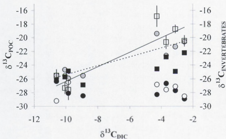
Figure 11 : \delta^{13}\text{C} of different SPOM size fractions (left Y-axis) and of benthic invertebrates (open squares, right Y-axis) versus \delta^{13}\text{C} of dissolved inorganic carbon. Black circles : total SPOM, open circles : < 10 \mu\text{m} , grey circles : 10 << 50 \mu\text{m} , black squares : 50 << 118 \mu\text{m} . Error bar = 1 s.d.
