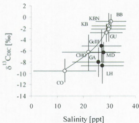
Figure 26 : Average \delta^{13}\text{C}_{\text{DIC}} values for each of the seasonal sampling locations versus the average salinity at these locations. Error bars indicate 1 s.d. Abbreviations of sampling locations as in legend of Figure 1.
