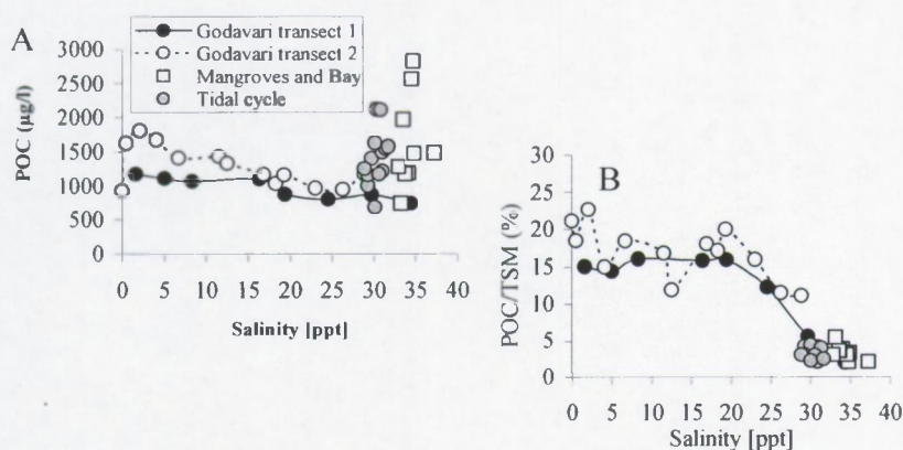
Figure 10 : (A) Concentrations of particulate organic carbon along the salinity gradient of the Gautami Godavari and in the mangrove creeks and Kakinada Bay (note that some data from Kakinada Bay are missing, see Table 3), and (B) contribution of organic carbon to the total suspended matter (TSM) pool. Legend as in panel A. Note that two high values from Coringa were not included as they were well out of the range of other data ( \text{POC} > 7000 \text{ } \mu\text{g l}^{-1} , see Table 3 for details).
