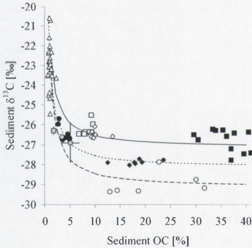
Figure 1 A : \delta^{13}\text{C} (in ‰) of organic carbon versus organic carbon content (% dry weight) of surface sediments from various mangrove ecosystems. Open triangles represent data from the Coringa Wildlife Sanctuary, full circles : Excoecaria agallocha zone (Galle), open circles : Rhizophora spp. zone (Galle), open diamonds : Avicennia spp. zone (Pambala), full diamonds : Rhizophora spp. zone (Pambala), open squares : data from Kazungu (1996), grey square : data from Dittmar & Lara (2001), and black squares : data from Lallier-Verges et al. (1998), grey-filled circles : data from Jennerjahn & Ittekkot (2002). Error bars : 1 s.d. Different curves correspond to different assumptions for \delta^{13}\text{C} and organic carbon content for the two end-members (see text for details).
