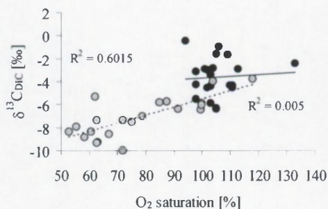
Figure 21 : Relationship between oxygen saturation levels and the carbon stable isotope composition of the DIC pool ( \delta^{13}\text{C}_{\text{DIC}} ) for the Godavari data (black symbols) and the data from mangrove creeks but excluding Kakinada Bay data (grey symbols).
