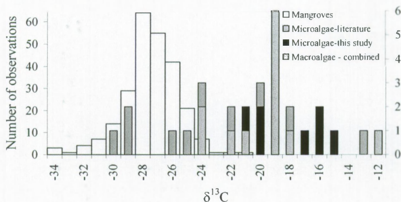
Figure 7 : Frequency distribution of \delta^{13}\text{C} values of mangrove leaves (both literature data and data gathered in this study, left-hand Y-axis) and \delta^{13}\text{C} values of micro- and macroalgae (right-hand Y-axis). See legend for details. Data sources for algae : M. Skov (unpublished data), Rodelli et al. (1984), Ambler et al. (1994), Newell et al. (1995), Primavera (1996), Dittel et al. (1997), Lee (2000), Machiwa (2000), Sheaves & Molony (2000).
