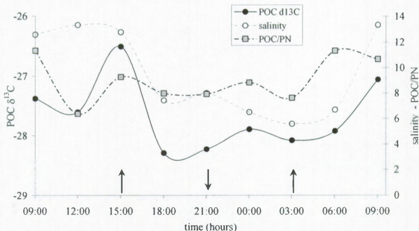
Figure 4: Salinity (open circles), elemental composition (grey squares) and stable carbon isotopic composition (full circles) of suspended particulate organic matter collected during a 24 hour period at the central Gaderu station ( G_3 ) on 16-17 November 1995. Arrows pointing upward indicate high tides, the arrow pointing downward indicated the time of low tide.
