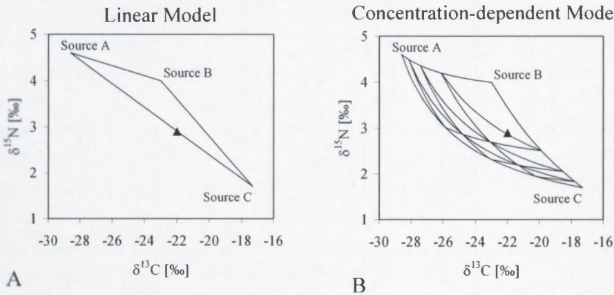
Figure 4. Contribution of 3 different sources (A, B, and C) to the diet of an organism (represented by the triangle) according to (A) a linear 3-source mixing model (Phillips & Gregg 2001), and (B) a concentration-dependent 3-source mixing model (Phillips & Koch 2001). Note that the \delta^{13}\text{C} and \delta^{15}\text{N} values of the food sources have been corrected for trophic enrichment.
