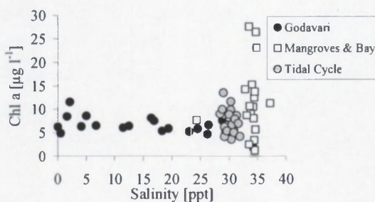
Figure 14 : Chlorophyll a concentrations ( \mu\text{g l}^{-1} ) along the salinity gradient of the Gautami Godavari and in the mangrove creeks and Kakinada Bay during the pre-monsoon period of 2001.
