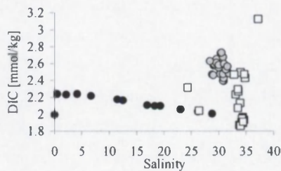
Figure 5: Variations in dissolved inorganic carbon concentration along the Gautami Godavari salinity gradient and in the mangrove creeks and Kakinada Bay during the pre-monsoon period of 2001.
