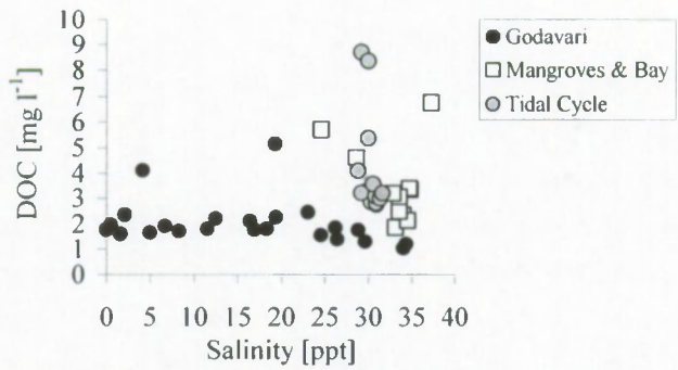
Figure 11 : Variations in the concentration of dissolved organic carbon (DOC) along the salinity gradient of the Gautami Godavari (black symbols), in the mangrove creeks and Kakinada Bay (open symbols + grey symbols taken during the diurnal cycle).
