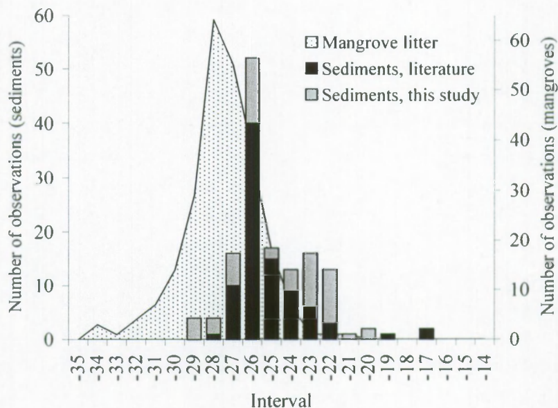
Figure 3 : Distribution of \delta^{13}\text{C} data of mangrove leaves (right axis, updated from Bouillon et al. 2002b i.e. Chapter 8) and intertidal mangrove sediments (left axis) from published literature sources (black bars) and this study (grey bars). Indicated \delta^{13}\text{C} value on X-axis corresponds to the upper level of the interval. Total number of sediment \delta^{13}\text{C} data is 141. Literature sources for sediment \delta^{13}\text{C} data : Fry (1984), Rodelli et al. (1984), Lacerda et al. (1986), Ambler et al. (1994), Hemminga et al. (1994), Kazungu (1996), Dittel et al. (1997), Loneragan et al. (1997), France (1998), Lallier-Verges et al. (1998), Machiwa (2000), McKee et al. (2002), Dittmar & Lara (2001c), Hsieh et al. (2002), Jennerahn & Ittekkot (2002), E. Olafsson & M. Skov (unpublished data).
