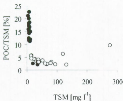
Figure 17 : Relationship between the contribution of particulate organic carbon (POC) to the total suspended matter (TSM) pool and the TSM concentration itself for the Gautami Godavari salinity gradient (black symbols) and the mangrove creeks of the Coringa Wildlife Sanctuary and Kakinada Bay.
