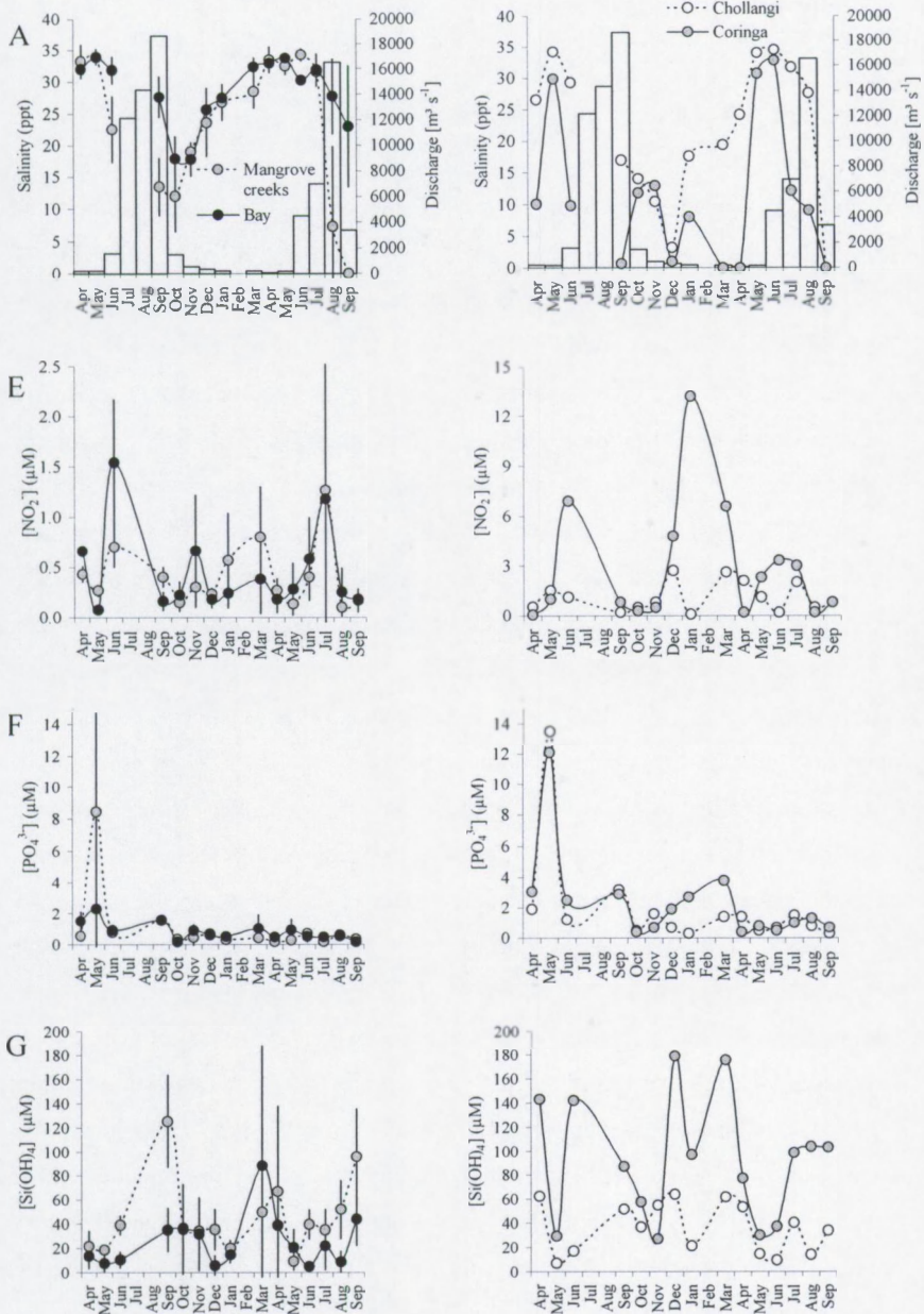
Figure 7 (continued) : Some physico-chemical parameters from mangrove creek locations (GA, Gc III, and LH), Bay locations (MD, GU, KB, KBN, and BB), and for two other creeks, Chollangi and Coringa between april 2000 and September 2001. See Chapter 4 for location of sampling stations. White bars on panel A (right-hand Y-axis) represent discharge rate of the Godavari at Dowleswaram Dam. Note the difference in Y-axis for panel B.
