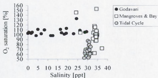
Figure 3 : Variations in the oxygen saturation state along the Gautami Godavari salinity gradient and in the mangrove creeks and Kakinada Bay during the pre-monsoon period of 2001.
