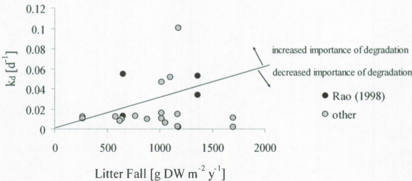
Figure 3 : Decay constant ( k_d ) versus litter fall for the Coringa Wildlife Sanctuary ( Avicennia officinalis and Excoecaria agallocha ) and other studies (Woodroffe 1985, Flores-Verdugo et al. 1987, Twilley et al. 1997, Wafar et al. 1997, Woitchik et al. 1997, Tam et al. 1998, Ashton et al. 1999, McKee & Faulkner 2000). Note that the data by Rao (1998) represent total annual litter fall rates, but decay constants for 2 different seasons per species.
