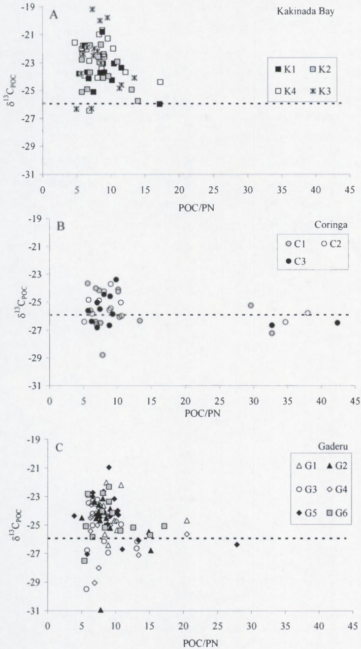
Figure 3 : Elemental (POC/PN) versus stable carbon isotope composition ( \delta^{13}\text{C} , in ‰) of suspended organic matter from the different sampling stations in (a) Kakinada Bay, (b) Coringa, and (c) Gaderu and Gautami Godavari. The horizontal dotted line represents average \delta^{13}\text{C}_{\text{POC}} (-25.9 ‰) for all samples with \text{POC/PN} > 12 .
