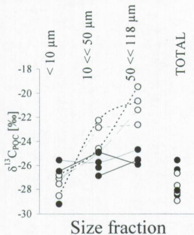
Figure 5 : \delta^{13}\text{C} differences between SPOM size classes. white symbols : bay locations (MD, GU, KB, and CA), black symbols : mangrove creek locations (LH, GA, CO, and GC).
