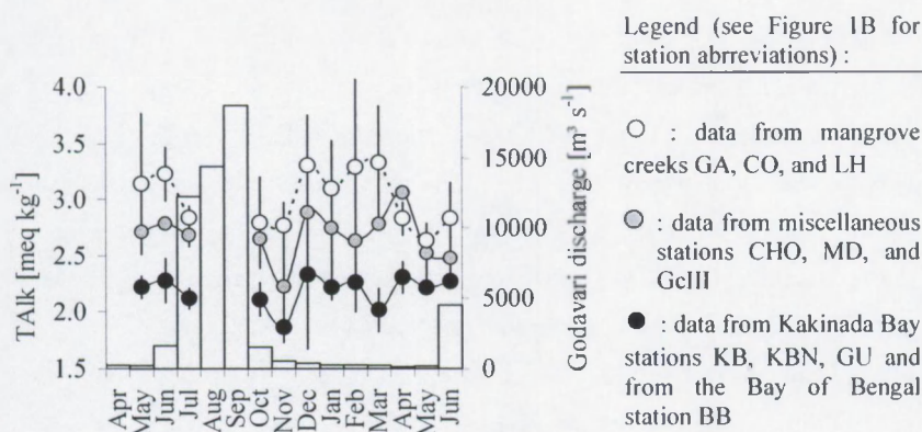
Figure 7 : Seasonality of Total Alkalinity at 10 sampling stations (see Figure 1B) in the mangrove creeks of the Coringa Wildlife Sanctuary and the adjacent Kakinada Bay. [Note : the choice of stations for which data were grouped in Fig 8 is the result of a paired t-test for data on \delta^{13}\text{C}_{\text{DIC}} , a similar approach for TAlk resulted in some additional significant differences -e.g. between GA on the one hand and LH and CO on the other hand- but for reasons of clarity these are not presented separately]. White bars indicate average monthly discharge for the Godavari at Dowleswaram Dam.
