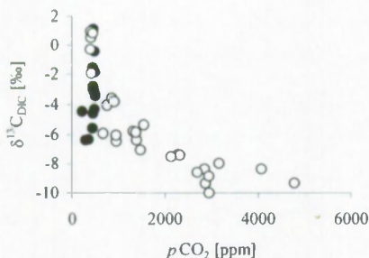
Figure 23 : Relationship between pH and the carbon stable isotope composition of the DIC pool for the Gautami Godavari (black symbols) and for the mangrove creeks and Kakinada Bay (open squares, grey circles are for the diurnal cycle) during the pre-monsoon of 2001.
