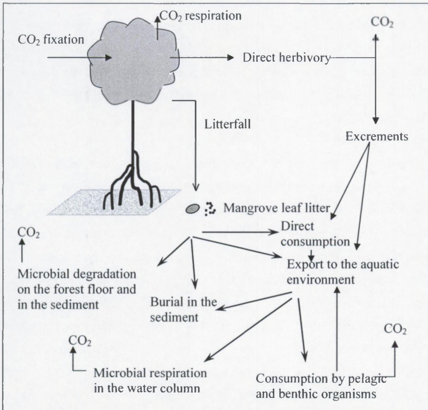
Figure 1 : Schematic representation of the potential fate of mangrove primary production.
