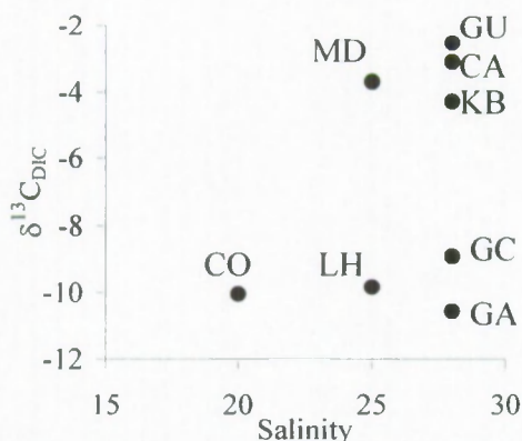
Figure 6 : Relationship between salinity (in ppt) and the carbon stable isotope composition of the dissolved inorganic carbon pool ( \delta^{13}\text{C}_{\text{DIC}} , in ‰). Sampling locations as in Figure 3.
