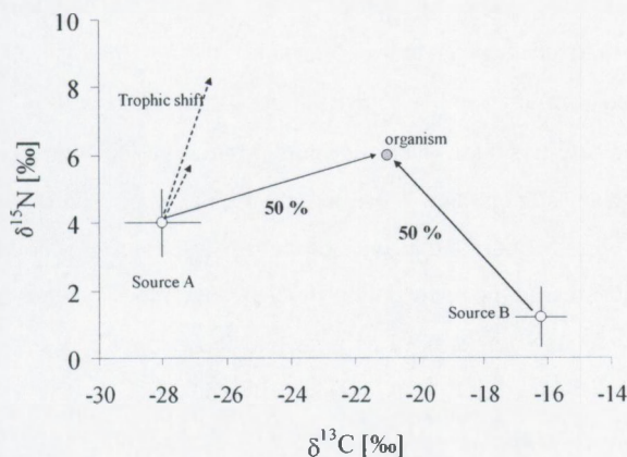
Figure 3 : Simplified graphical representation of the combined use of C and N stable isotopes to estimate the contribution of two food sources to an organisms diet : any organism deriving equal proportions of its diet from source A and B is expected to have an isotopic composition close to that shown in the figure.
