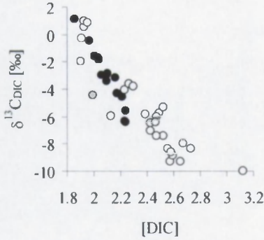
Figure 19 : Relationship between dissolved inorganic carbon concentration and its carbon isotope composition for data collected during the pre-monsoon period of 2001 along the Gautami Godavari (black symbols), and in the mangrove creeks and Kakinada Bay (open symbols). Grey symbol represents the sample from Dowleswaram Dam (see text for details).
