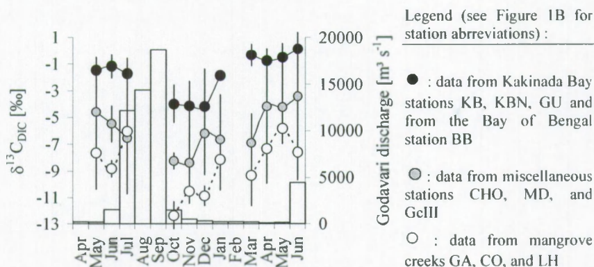
Figure 9 : Seasonality of \delta^{13}\text{C}_{\text{DIC}} at 10 sampling stations (see Figure 1B) in the mangrove creeks of the Coringa Wildlife Sanctuary and the adjacent Kakinada Bay. White bars indicate average monthly discharge for the Godavari at Dowleswaram Dam. [Note : the choice of stations for which data were grouped in Fig 11 is the result of a paired t-test for \delta^{13}\text{C}_{\text{DIC}} data].
