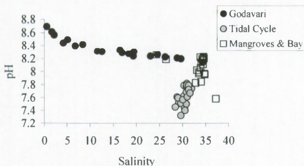
Figure 2 : pH variations along the Gautami Godavari salinity gradient and in the mangrove creeks and Kakinada Bay during the pre-monsoon period of 2001.
