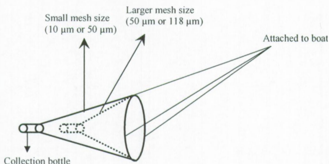
Figure 6 : Custom-made nets for the collection of different size-fractions of suspended matter.
