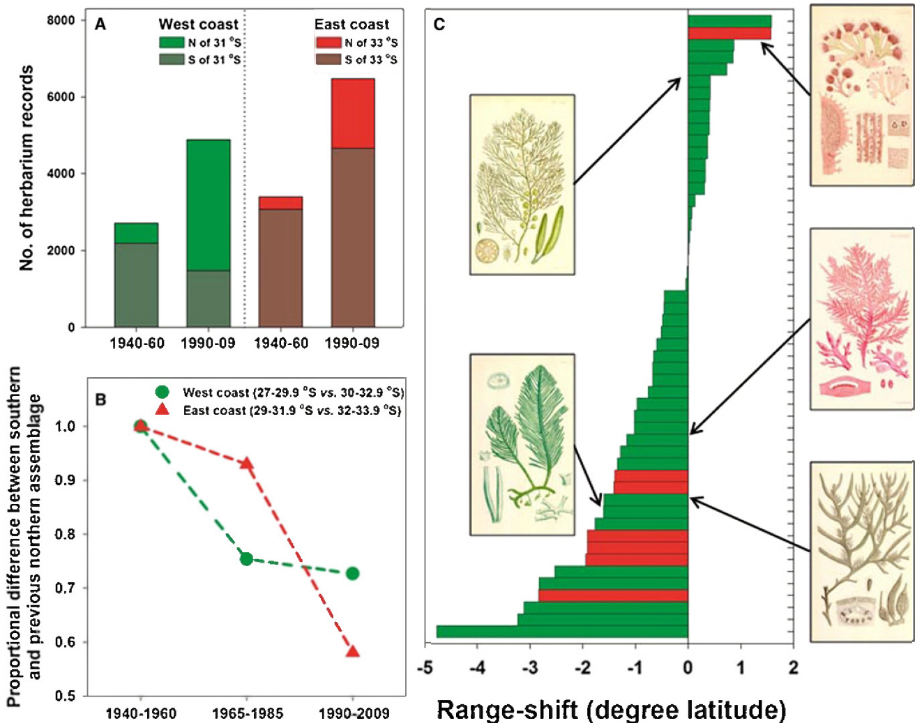
Figure 1. Poleward Shifts in Temperate Macroalgae in Australia Assessed from Herbarium Records (A) Sampling intensity (records from Australia’s Virtual Herbarium) on the west and east coasts of Australia during 1940–1960 and 1990–2009. (B) Multivariate dissimilarity in assemblage structure (proportional Sorensen dissimilarity) between past northern and subsequent southern floras. (C) Shift in northern range limits of temperate macroalgae in Australia from 1940–1960 and 1990–2009. Inserts: Color plates of selected algae from Henry Harvey’s Phycologia Australica (1858–1863); from top left, Caulocystis uvifera and Caulerpa flexilis and top right, Martensia fragilis , Pterocladia lucida , and Scytothalia doryocarpa (source: http://users.ugent.be/phycology/harvey ). A complete list of species can be found in Table S1 (see G and H).
