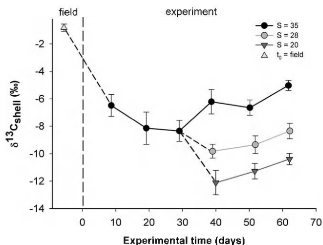
Fig. 5. Evolution of stable carbon isotope values ( \delta^{13}\text{C}_{\text{shell}} ) in R. philippinarum shells during the experiment for the three salinity conditions (20, 28 and 35). Values are expressed as means and error bars represent standard deviations, n=15 during the first 35 days; n=5 from day 35 to 64 for each point.
