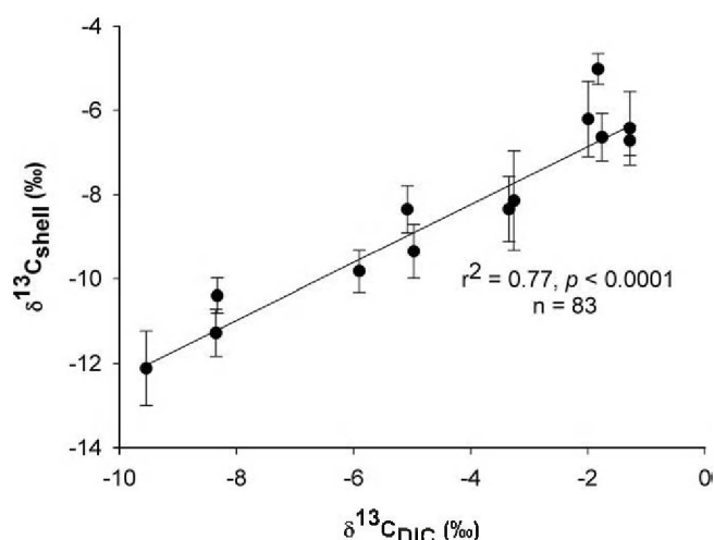
Fig. 6. \delta^{13}\text{C}_{\text{shell}} vs \delta^{13}\text{C}_{\text{DIC}} in clam tanks for samples taken over the experiment. Error bars represents standard deviations. The solid line shows the linear least squares regression calculated with all data obtained during this experiment ( r^2=0.77 , p<0.0001 , n=83 ).
