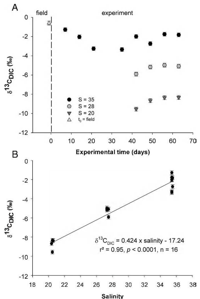
Fig. 3. A: DIC stable carbon isotope values ( \delta^{13}\text{C}_{\text{DIC}} ) during the experiment. Three salinity conditions (20, 28 and 35) were tested from days 35 to 64. B: \delta^{13}\text{C}_{\text{DIC}} as a function of salinity during the experiment. Error bars represent the analytical precision ( 1\sigma ).
