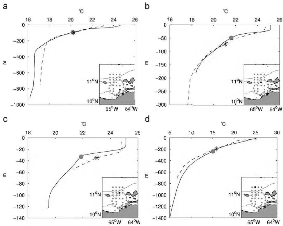
Fig. 5. Observed (dashed line) and modelled (solid line) profiles at four locations in the Cariaco basin domain (two inside the basin, one at the Tortuga channel, and one outside the basin). The asterisk and the grey circle show the thermocline depth for the observed and modelled profile respectively. Small inset maps show the position of the profiles with a black circle, and the 200 m isobath as a thin black line.
