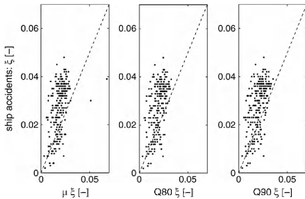
Fig. 16. Observed wave steepness (total sea) versus climate mean, 0.8-quantile, and 0.9-quantile wave steepness.
