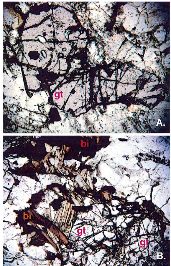
Fig. 7. Photomicrograph of garnet gneiss clasts in basement rocks at Site 1137 (Elan Bank). A: Poikiloblastic (gt) in a conglomerate clast. Field of view is 1.4 mm, plane-polarized light. B: Porphyroblastic garnet (gt) and biotite (bi) in a clast contained in a crystal-vitric tuff. Field of view is 2.75 mm, plane-polarized light.
