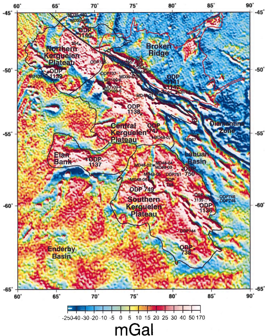
Fig. 1. Plate reconstruction of the Kerguelen Plateau and Broken Ridge free-air gravity field [67] at C18n.2n 0 (40.1 Ma) using rotation poles of [68] Kerguelen Plateau sector boundaries are outlined in black. Leg 183 drill sites (★), Leg 119/120 drill sites (circles) and dredge or piston core locations (squares) where igneous basement was recovered are in black; where only sediment was penetrated, the symbols are white.
