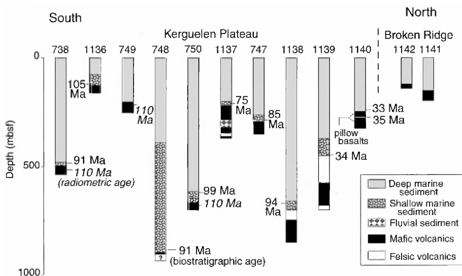
Fig. 3. Summary of ODP drill holes on the Kerguelen Plateau that recovered volcanic rocks. Data are shown for Leg 119 (Site 738), Leg 120 (Sites 747, 748, 749 and 750) and Leg 183 (Sites 1136, 1137, 1138, 1139, 1140, 1141 and 1142). Multichannel seismic reflection profiles indicate that the volcanic rocks at all sites except Site 748 were recovered from the uppermost basement of the plateau, which lies beneath younger sedimentary cover. Basalt at Site 748 was recovered ~200 m above the seismically defined basement and overlies a poorly recovered zone that contains smectitic clay and highly altered basalt. Radiometric ages for basalts [25–28] are shown in italics. Biostratigraphic ages of sediments overlying basement are also indicated. Data sources are as seen in EPSL Online Background Data Set 1 .
