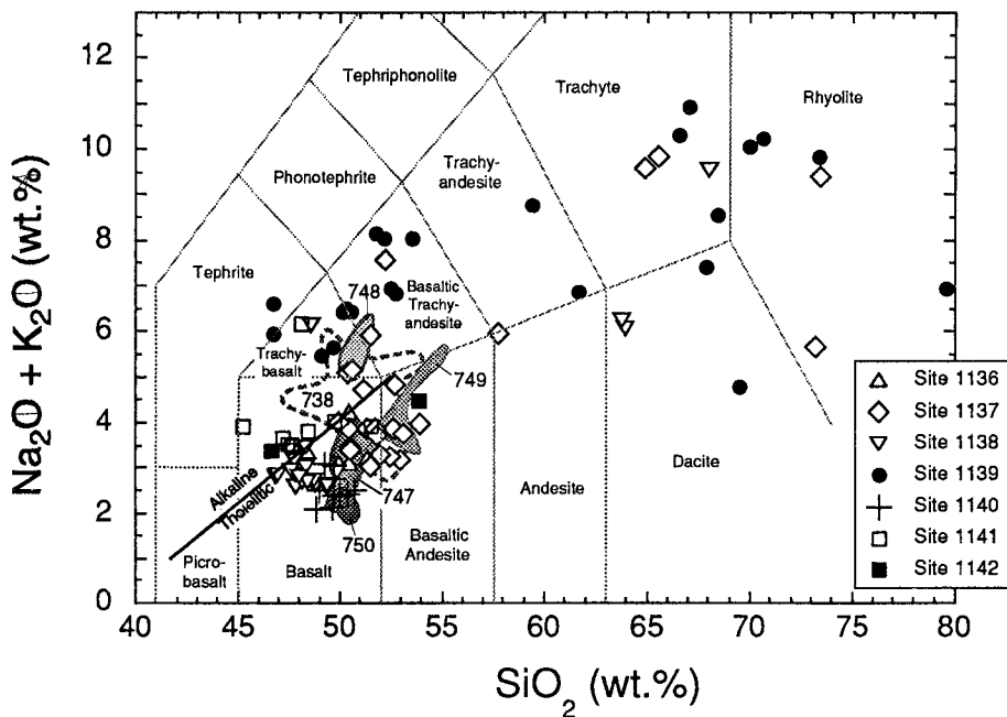
Fig. 4. Total alkalis ( \text{Na}_2\text{O}+\text{K}_2\text{O} ) versus \text{SiO}_2 classification plot for igneous rocks recovered by drilling on the Kerguelen Plateau and Broken Ridge. Although in detail this plot is affected by post-magmatic mobility of alkalis, the principal aspects of the data reflect magmatic characteristics. Important features are: (a) the dominance of basalt with subordinate trachyte, rhyolite and dacite at Sites 1137, 1138 and 1139; and (b) lavas at some sites are dominantly tholeiitic basalt (Sites 750 and 1140) whereas the low \text{SiO}_2 lavas at Site 1139 are alkalic (trachybasalt and basaltic trachyandesite). Data sources are in EPSL Online Background Data Set (see footnote 1).
