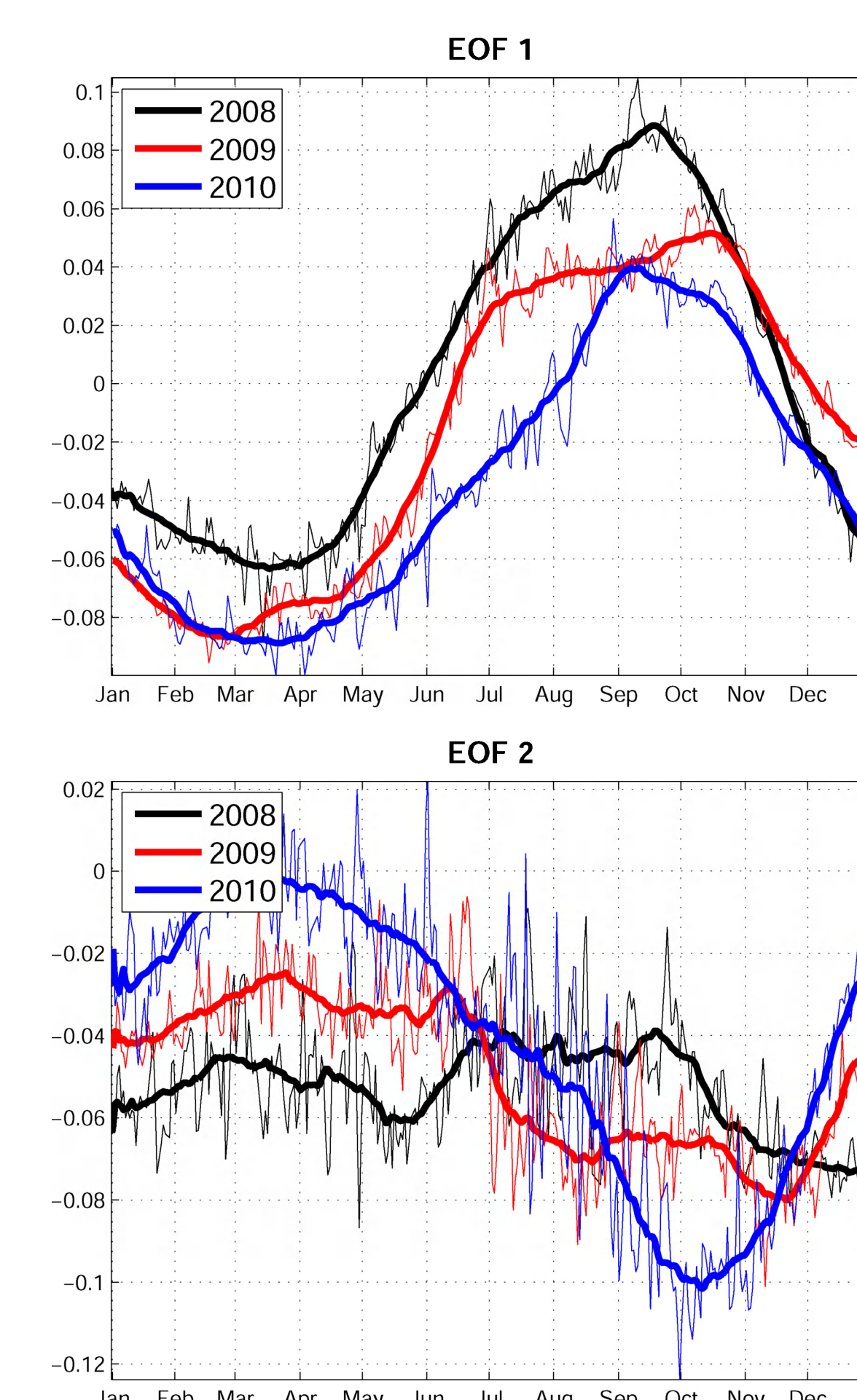
FIGURE 5: First two temporal EOFs. Thick curves indicate the 30-day running averages.
