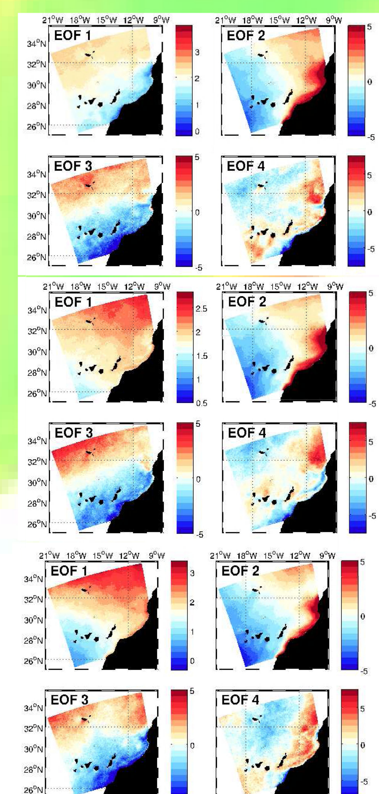
FIGURE 4: First four spatial modes for 2008, 2009 and 2010.
