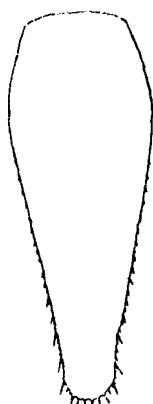
FIG. 3.— Outline of telson; the row of lateral subdistal impressions omitted.
