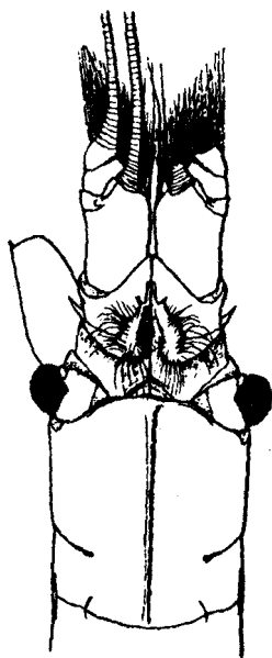
FIG. 20. — Front part of an adult male, from above.
