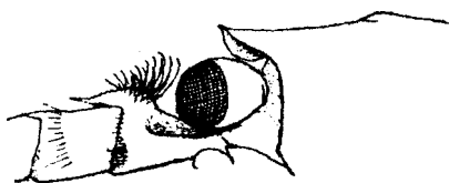
FIG. 13. — Front and of carapace, left eye and peduncle of antennula of T. distinguenda , from the side.
