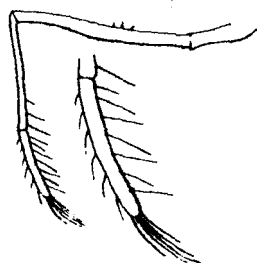
FIG. 23. — Left elongate leg (of first pair) of the same specimen.
