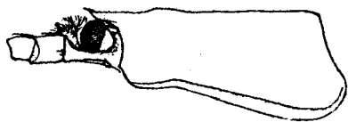
FIG. 14. — Carapace with left eye and antennular peduncle of a female T. lateralis .
