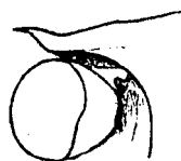
FIG. 15. — Outline of front end of carapace and eye of the same specimen, more highly magnified.
