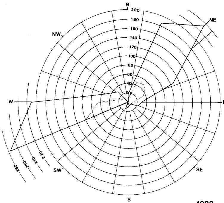
Fig. 6. a-b. Annual variations of wind direction and velocity at Yeong-il Bay.
