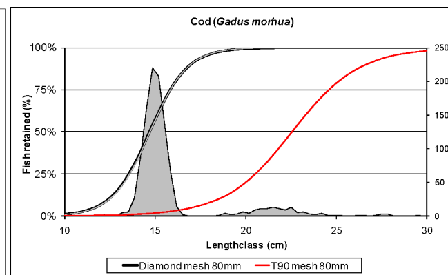
Fig. 15-3 – The selection ogives for a standard 80mm commercial cod-end and a 80mm T90 cod-end for five commercial and one non-commercial species. For each species the length frequency distribution for the total catch (cod-end + cover) is given.
