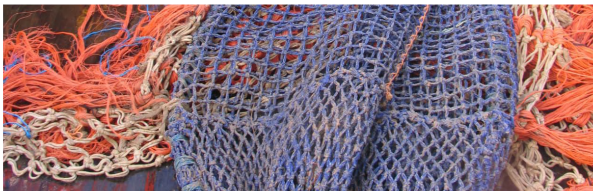
Figure 3-2 – Square mesh cod-end with a posterior sheet of diamond mesh
