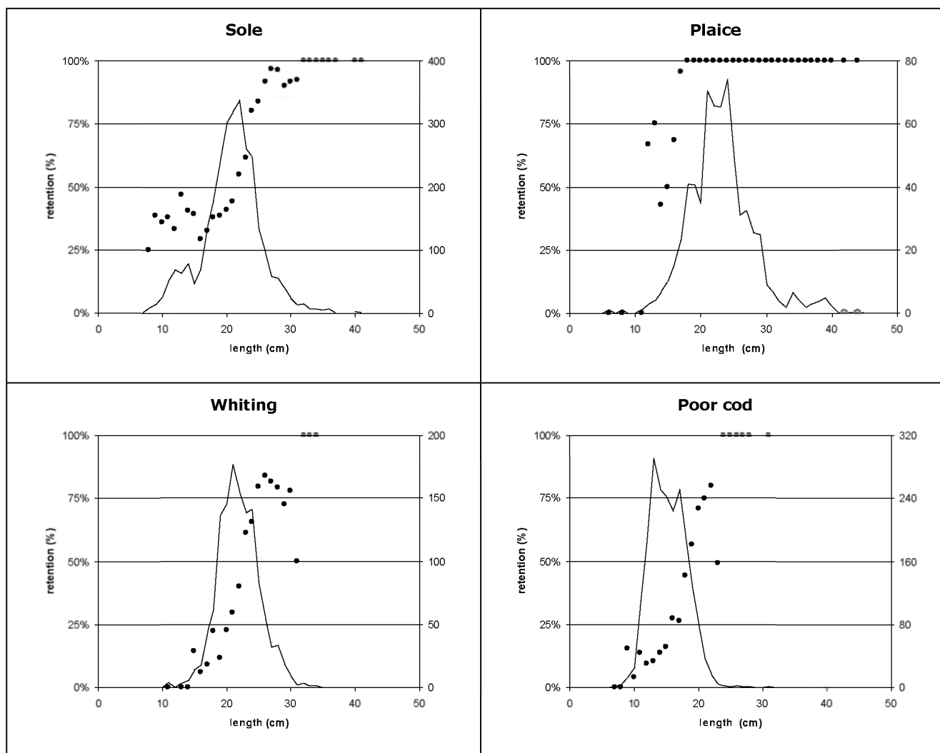
Figure 3-3 – Retention of fish in a square mesh cod-end (dotted line), total number of fish caught in both cod-end and cover (full line)
