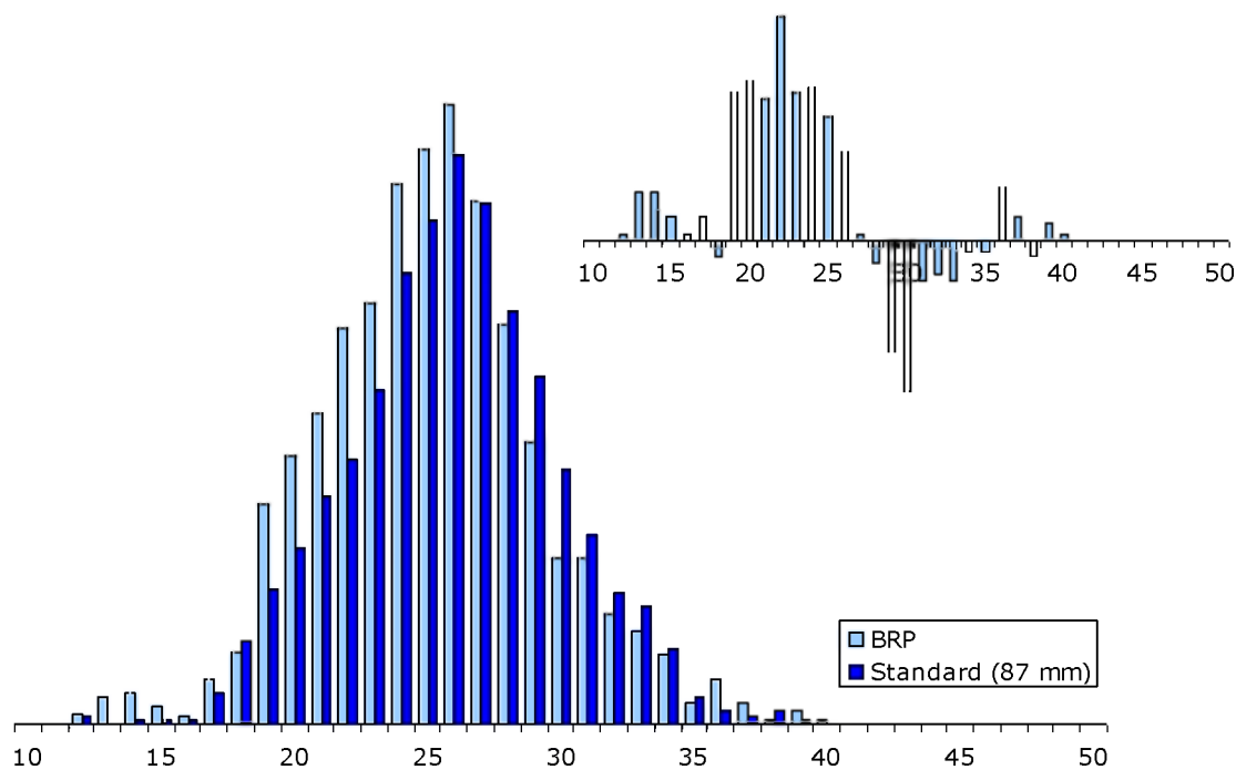
Fig. 17-10 - Length distribution of sole catch with experimental (BRP) and standard configuration (large mesh cod end) (Trip 3a); small graph shows catch difference (by number)
