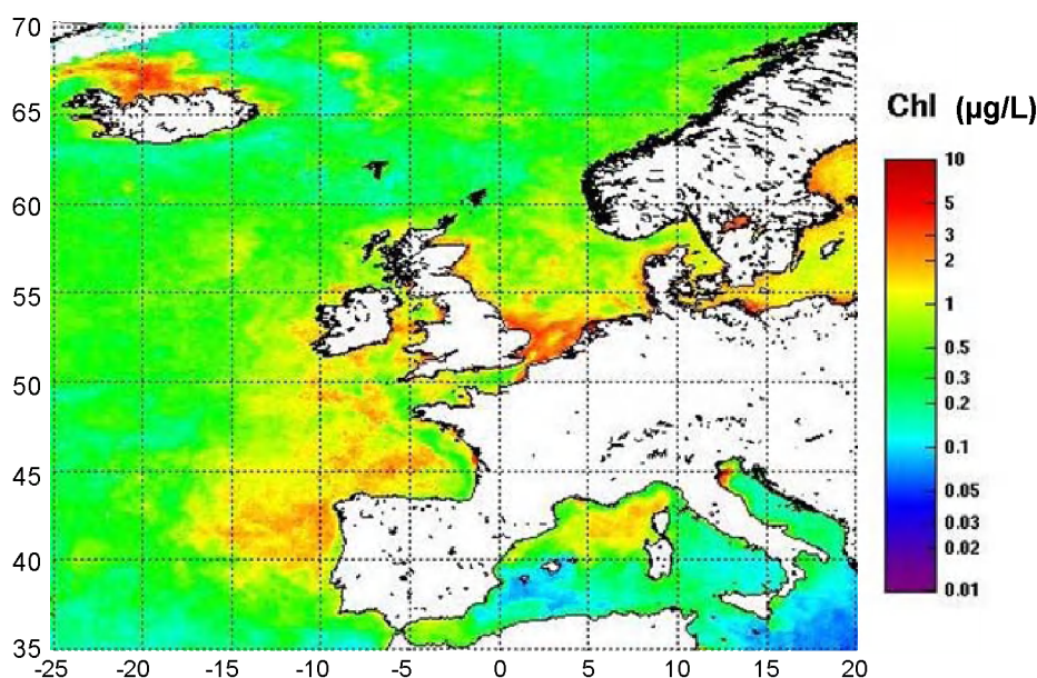
Figure 3.5 Chlorophyll a, April 2005 (Merged SeaWiifs-Modis-Meris image). Monthly means (µg/L) reflect only roughly chlorophyll distributions, relevant for assessments, but indicate regional gradients. Acknowledgement: ACRI & the GlobColour team. GlobColour is funded by ESA with data from ESA, NASA and GeoEye.
