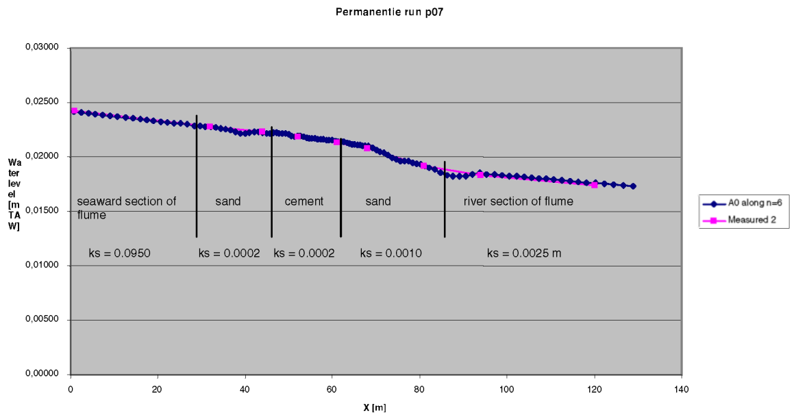
Figure 5.10: Calibration of numerical scale model and derived Nikuradse roughness.
