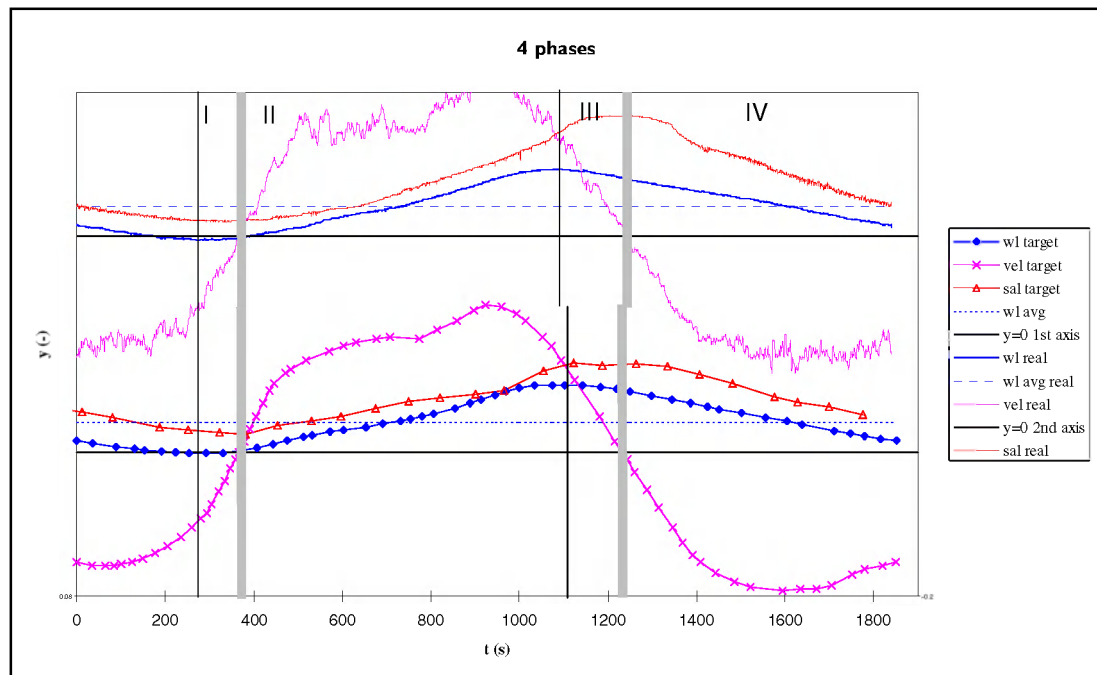
Figure 5.7: Comparison of phase differences of target water level, velocity and salinity. Top panel: realised curves (tide 23 15/05/2003); bottom panel: target curves.
