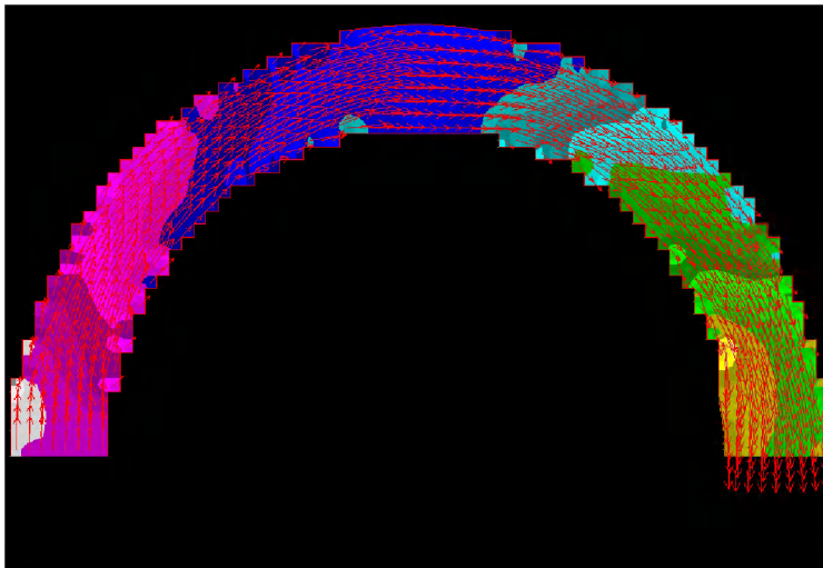
Figure 5.15b: Velocity distribution in river bend with rectangular grid without smooth boundary approximation
