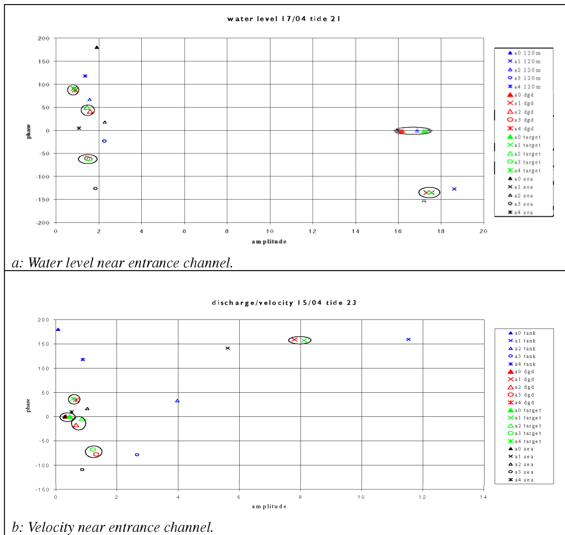
Figure 5.6: Amplitude-phase diagrams.
