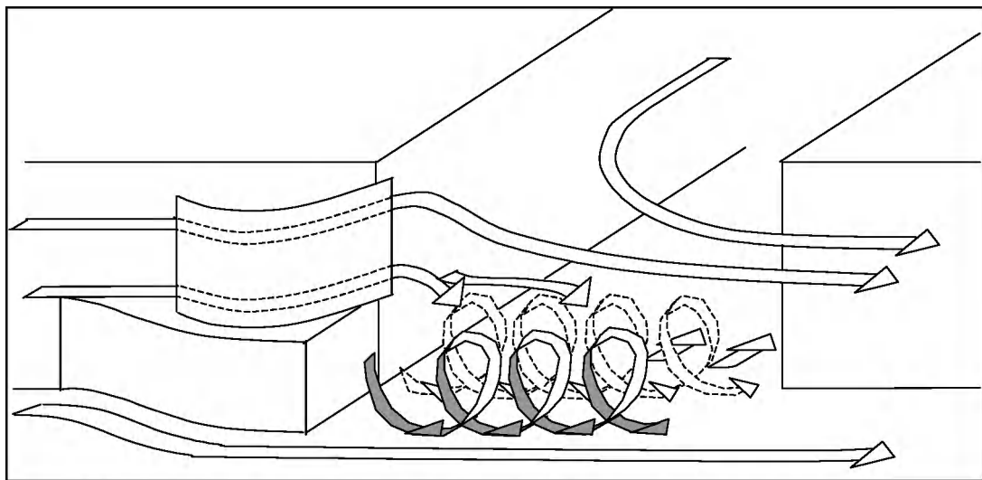
Figure 2.2. Schematic helical flow pattern in entrance during flood, with CDW present (non-homogeneous flow conditions).
