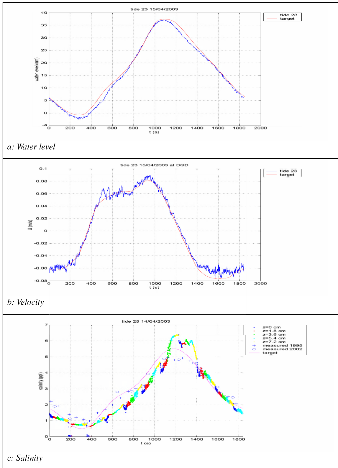
Figure 5.5: Calibration results for the physical scale model (van Kessel and Cornelisse, 2003).
