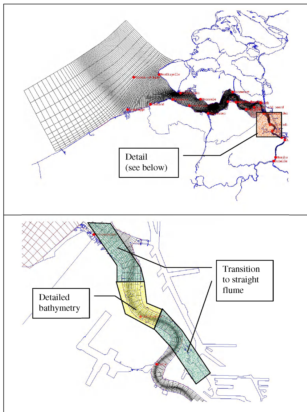
Figure 5.11: Overall Scheldt estuary model (upper) and detail for Beneden Zeeschelde with Tidal Flume.
