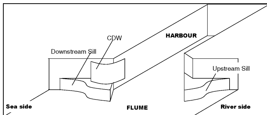
Figure 2.7: CDW-SILL system in the Delft Tidal Flume for non-homogeneous conditions (Hofland et al, 2001).
