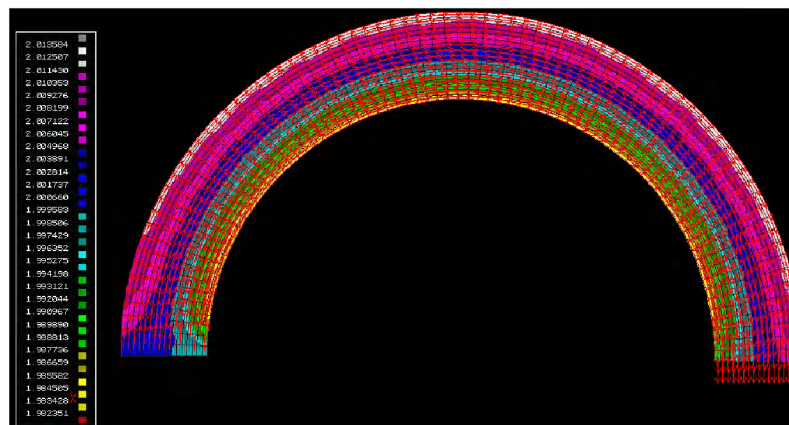
Figure 5.15a: Velocity distribution in river bend with ‘ideal’ circular grid
