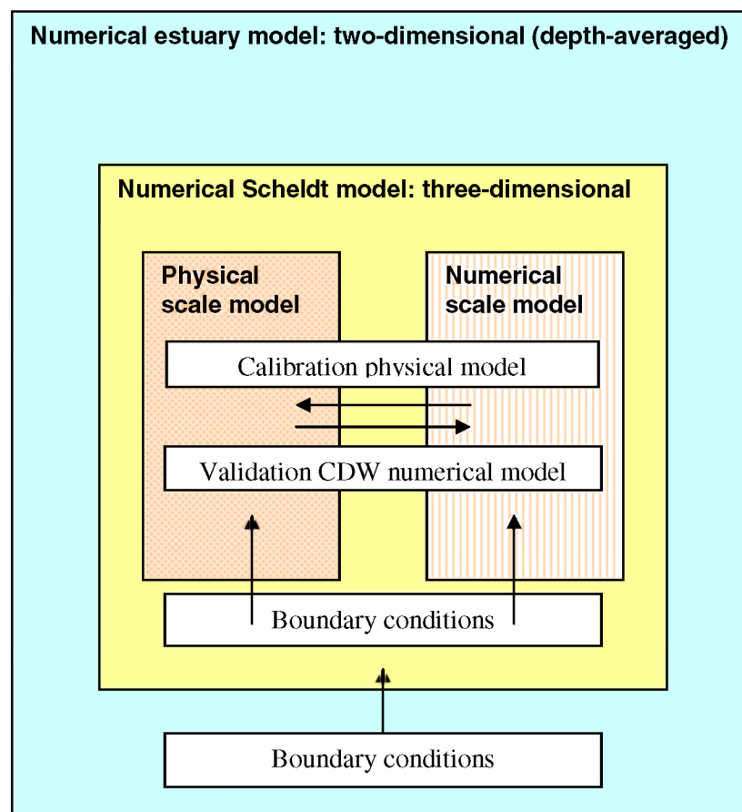
Figure 4.3: Schematic representation of modelling tools and their interactions.
