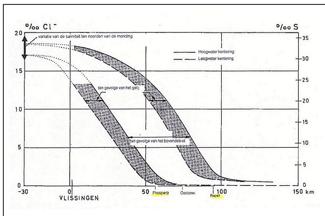
Figure 3.2: Salinity distribution in the Scheldt estuary (Peters and Sterling, 1976).
