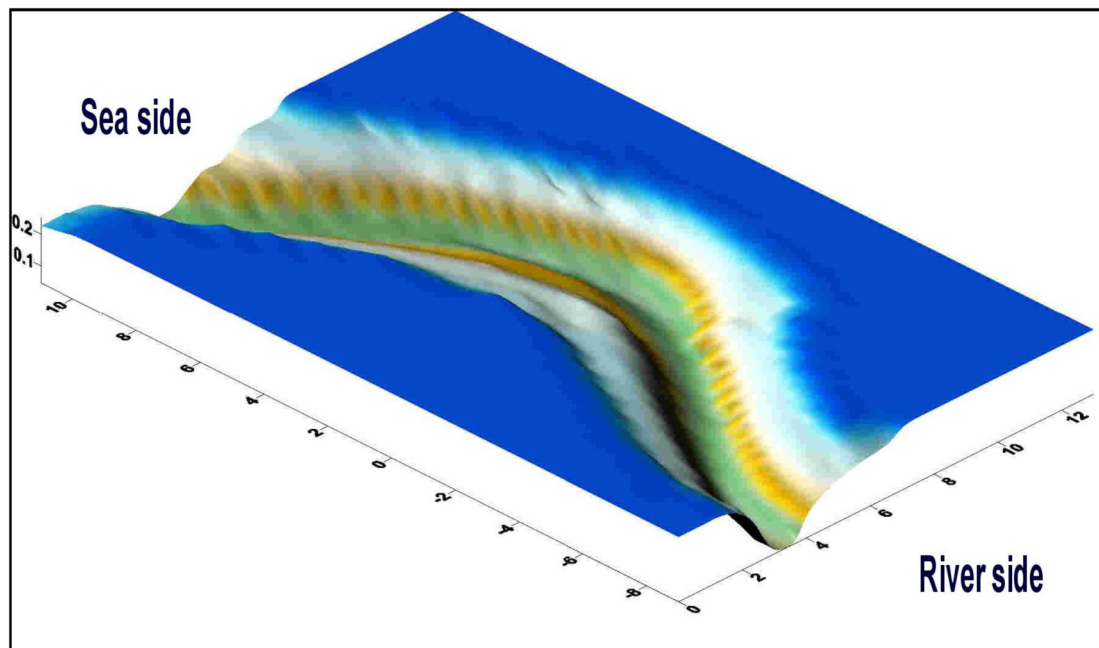
Figure 5.4: Bathymetry of the Beneden Zeeschelde between Kallo and Zandvliet in the physical scale model (figure is distorted).
