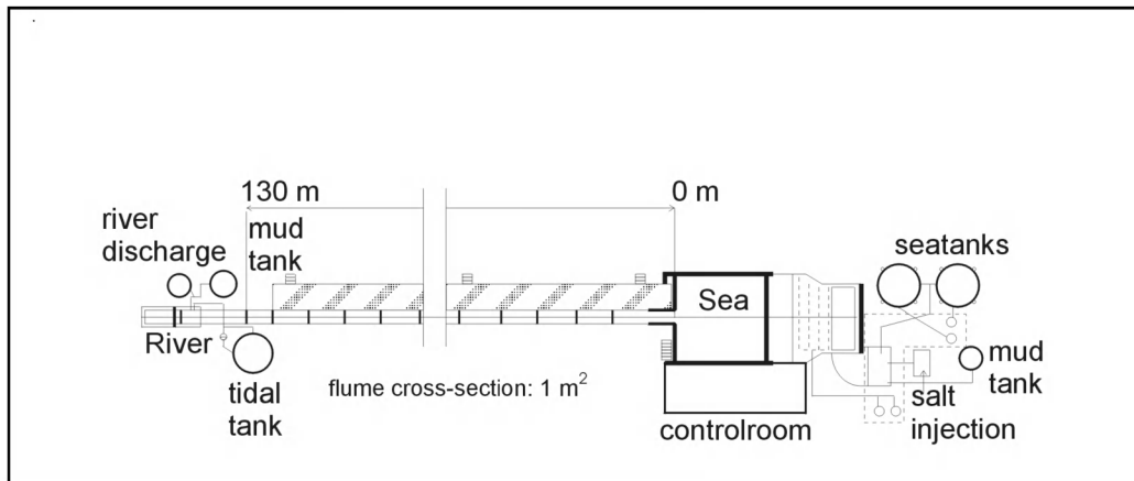
Figure 5.2: Delft Tidal Flume
