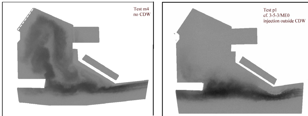
Figure 2.6: Dispersion of dye in the Parkhafen 700 s (model time) after start of dye injection upstream of the harbour entrance during flood. Left panel: without CDW; right panel: with CDW and dye injection at the outside of the CDW.
