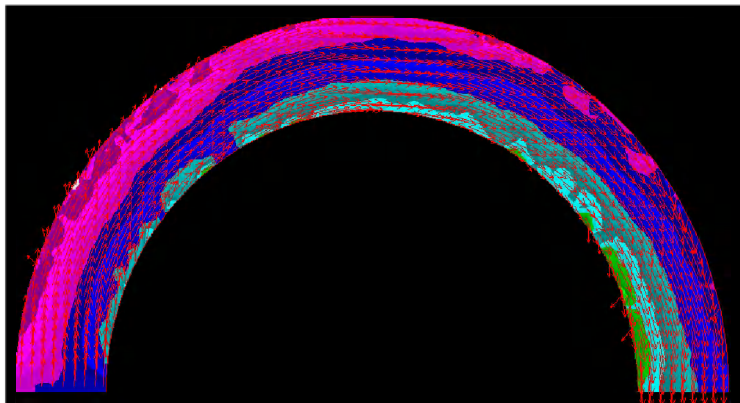
Figure 5.15c: Velocity distribution in river bend with rectangular grid with smooth boundary approximation
