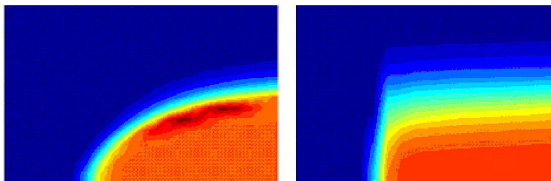
Figure 5.13: Characteristic salinity distribution (side view) of the front of a gravity current: non-hydrostatic model (left) and hydrostatic model (right) (Bijvelds, 2003).
