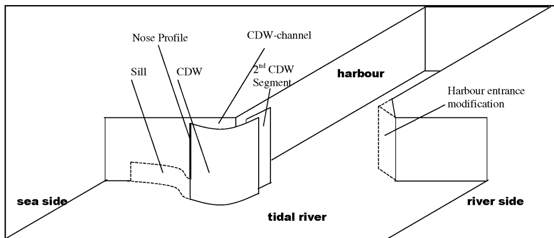
Figure 2.1: Sketch of Current Deflecting Wall for homogeneous flow conditions.
