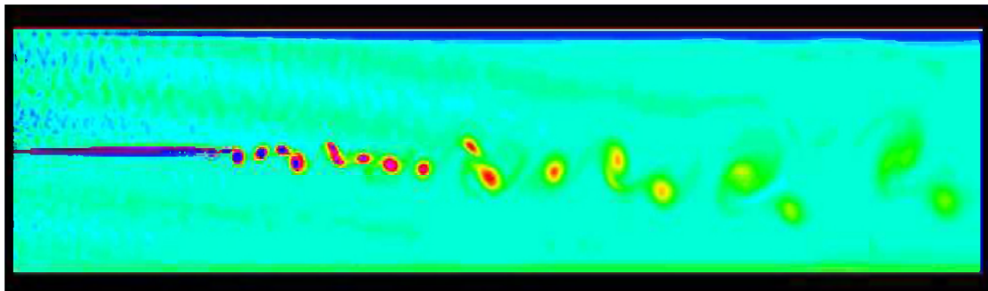
Figure 4.2: DELFT3D simulations: mixing layer due to velocity differences between upper and lower layer (figure is slightly distorted).
