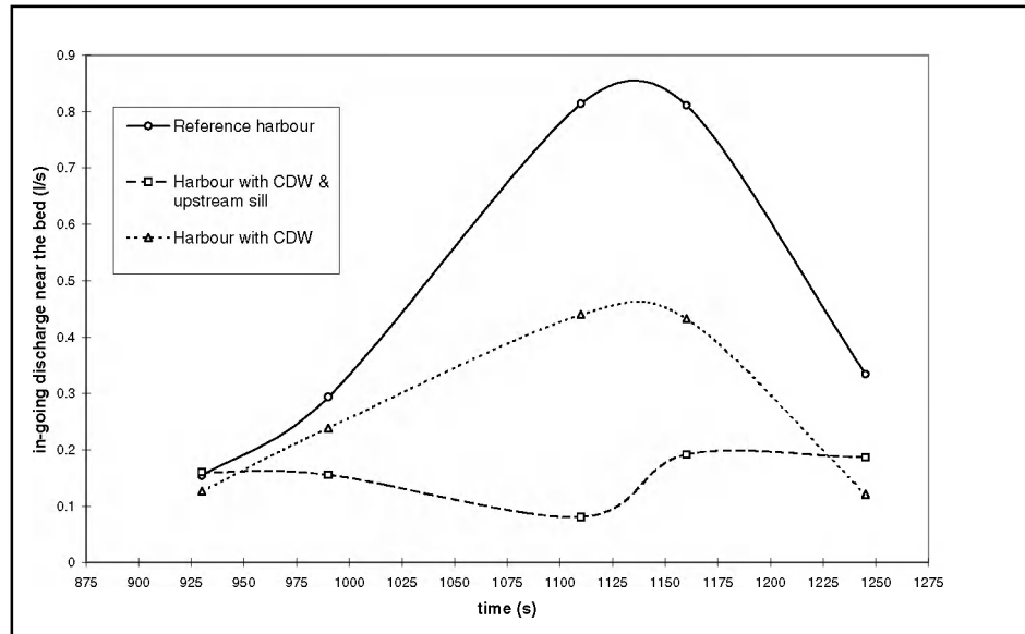
Figure 2.8: In-going discharge near the bed during periods from 925s to 250s in the next tidal cycle (Hofland et al, 2001).
