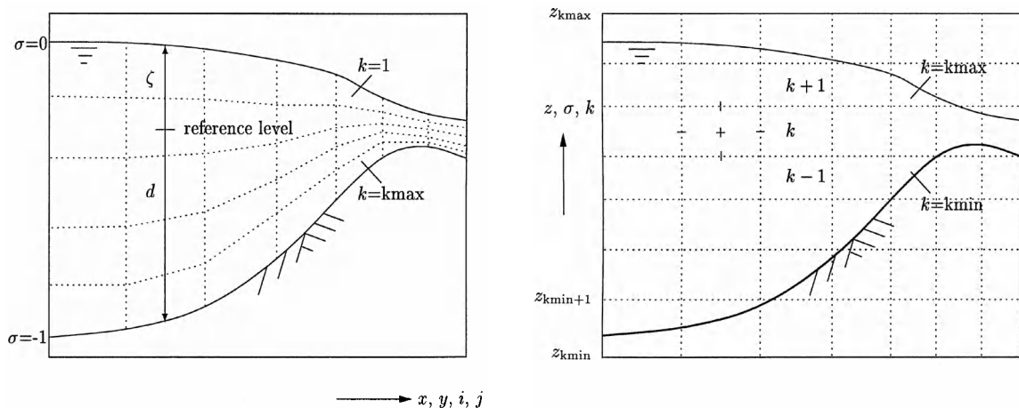
Figure 5.12: Vertical computational grid z -coordinate model (left) and the \sigma -model (right) (Van Kester et al, 2002).
