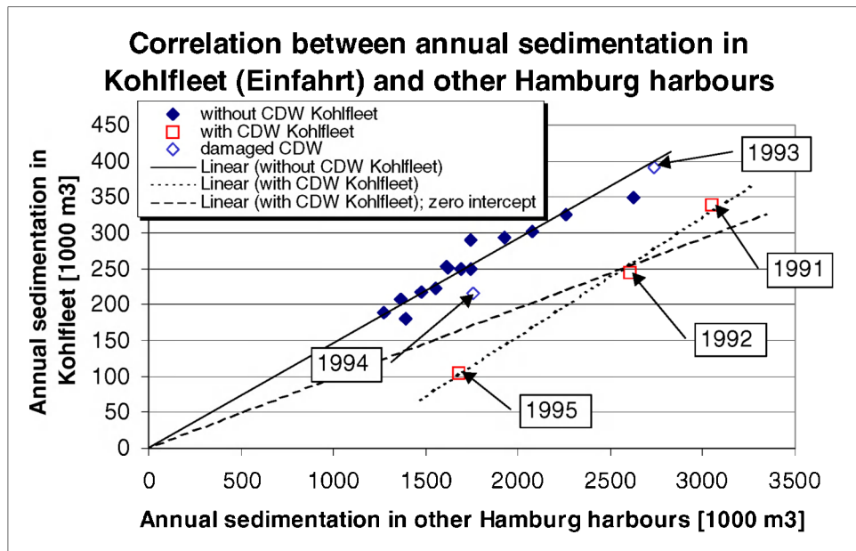
Figure 2.4: Annual siltation in the Köhlfleet harbour without and with CDW.
