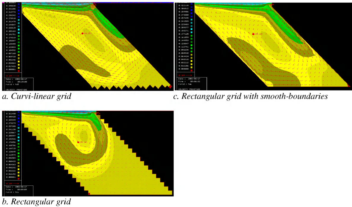
Figure 5.16: Effect of a stair-case boundary on the velocity distribution in a harbour basin.
