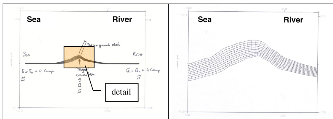
Figure 5.9: Grid schematisation of numerical scale model (coarse version).
