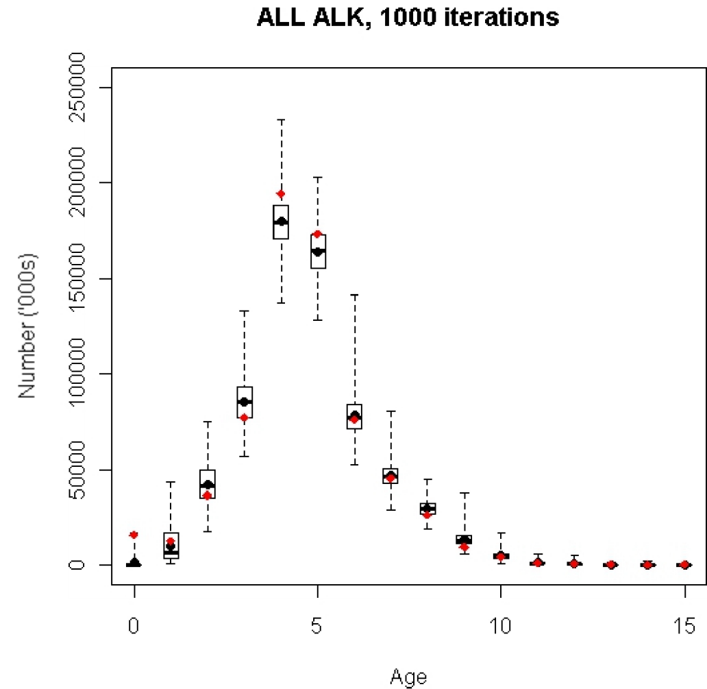
Figure 1: Bootstrap using all available ALKs. Box limits denote the interquartile range, whiskers extend to the most extreme outliers. Black dots show the mean, black bars the median and red dots the baseline result.
