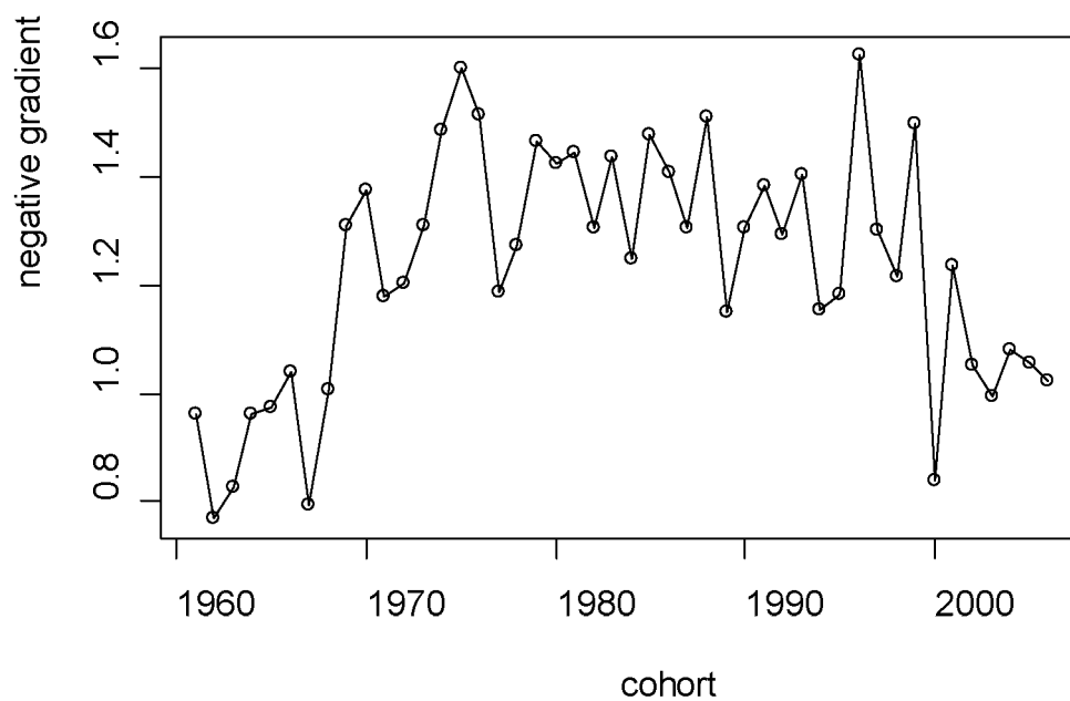
Figure 14.8 Cod in Subarea IV and Divisions IIIa (Skagerrak) and VIId. Log-catch cohort curves (top panel) and the associated negative gradients for each cohort across the reference fishing mortality of age 2-4.
