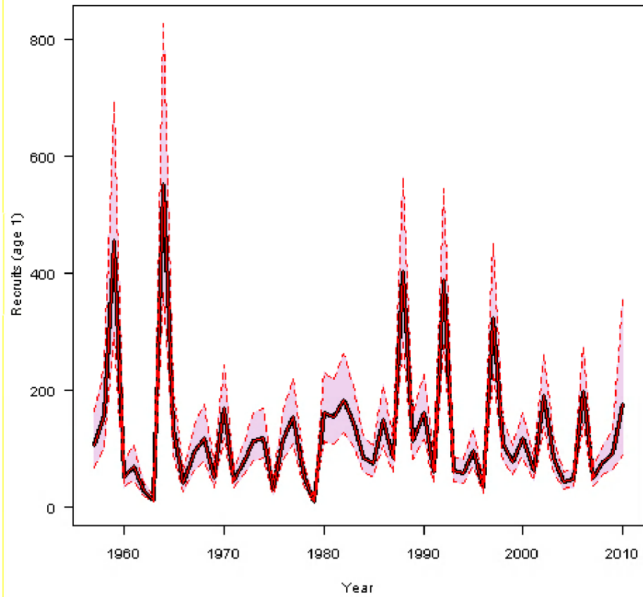
Figure 10.3.3c Sole in sub-area IV: Recruitment 1957–2010 output by SAM model.
