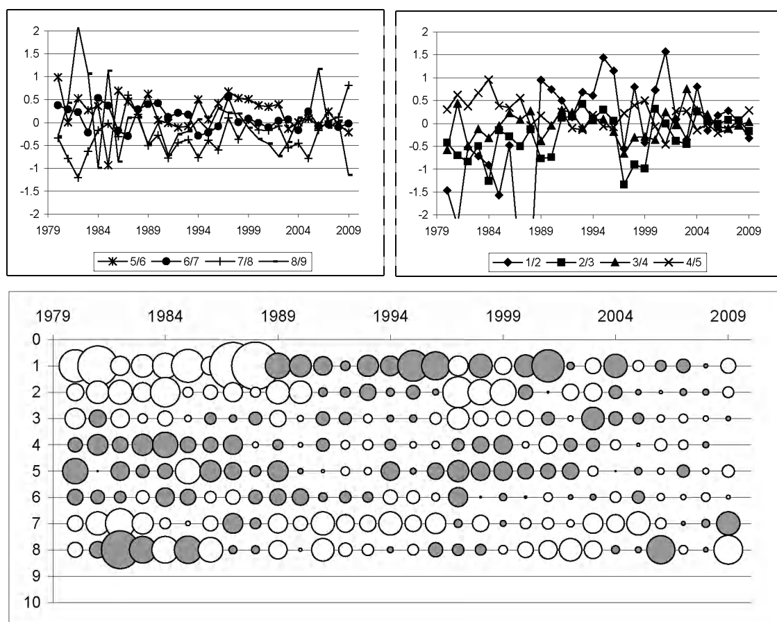
Figure 6.3.2.1 - Plaiice in VIId. Separable VPA
