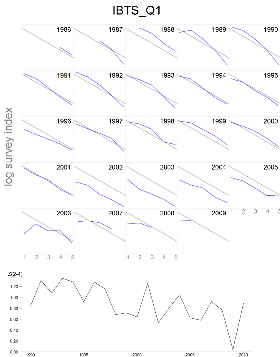
Figure 12.3.4 Whiting in IV and VII. Top panel: Log indices by cohort for the IBTS Quarter 1 survey (ages 1 to 5). The year specifies the year-class. A reference line with constant intercept and gradient representing a Z of 0.8 has been drawn in grey. Bottom panel: a raw estimate of annual mean Z averaged over ages 2 to 4, Z at age was estimated as \log \text{index}(y, a) - \log \text{index}(y+1, a+1) .
