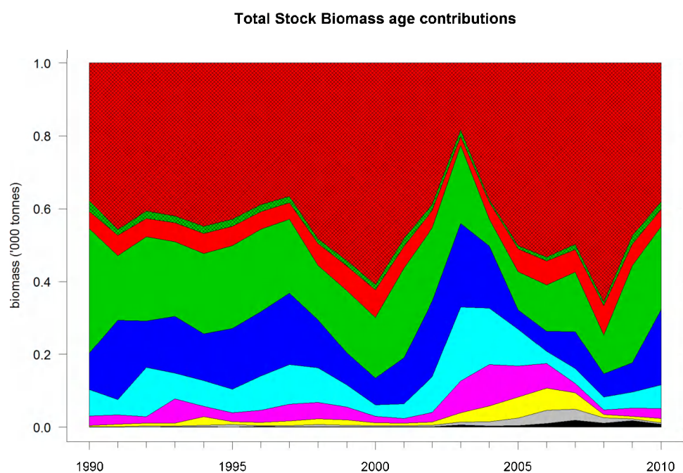
Figure 12.4.3 Whiting in IV and VIId. Age contributions to the SSB and TSB shown as proportions of the total stock biomass. Biomass not contributing to SSB is overlaid with hatched lines: immature age 1 lies over immature age 2, and the immature biomass lies over mature age 1, mature age 2 etc.
