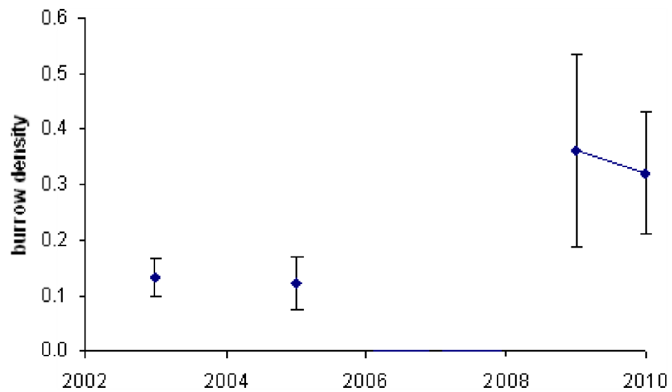
Figure 3.3.9.5. Nephrops , Devil's Hole (FU 34). Time series of TV survey density estimates, with 95 % confidence intervals, 2003, 2005, 2009-10.
