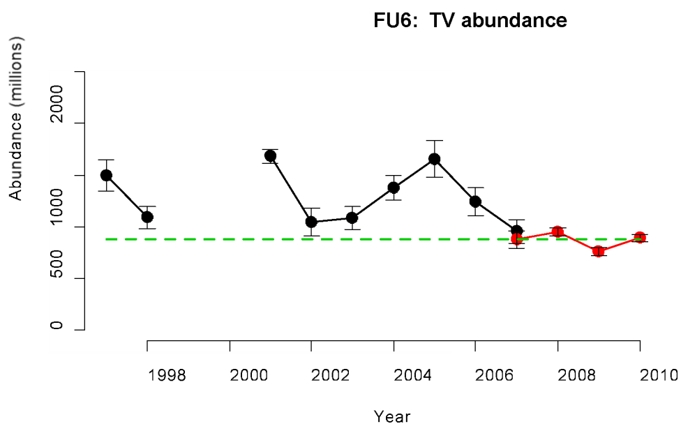
Figure 3.3.2.8 Nephrops in FU6: Time series of UWTV results. The dashed green line is the proxy for MSY B_{trigger} (879), the abundance estimate for 2007. The red line since 2007 gives the Geo-statistical abundance estimate using GPS measured distance. Prior to 2007 the estimate was raised using straight-line estimates of distance and stratified raising.
