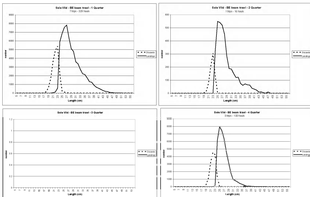
Figure 9.2.1e - Sole Vlied - BE Length distributions of discarded and retained fish from discard sampling studies of beam trawls in 2010
