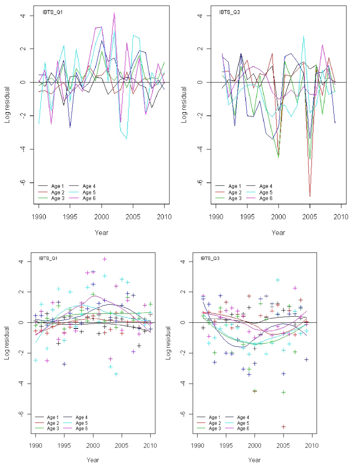
Figure 12.12.5 Whiting in Division IIIa. SURBAR analysis. Log residual estimates per age class for IBTS Q1 and IBTS Q3. Upper: line plots. Lower: point plots, with a loess smoother (span = 2) fitted through the points for each age class.
