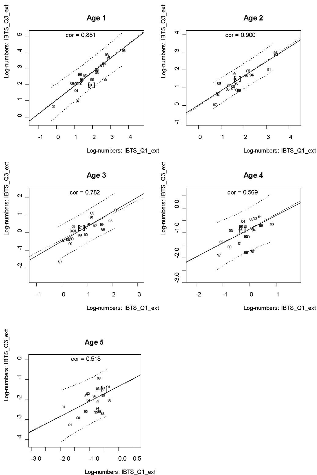
Figure 14.5c Cod in Subarea IV and Divisions IIIa (Skagerrak) and VIIId. Between-survey correlations for IBTSQ1 and Q3 surveys for the period 1991-2010. Individual points are given by cohort (year-class), the solid line is a standard linear regression line, and the broken line nearest to it a robust linear regression line. The pair of broken lines on either side of the solid line indicate prediction intervals. The most recent data appear in square brackets.
