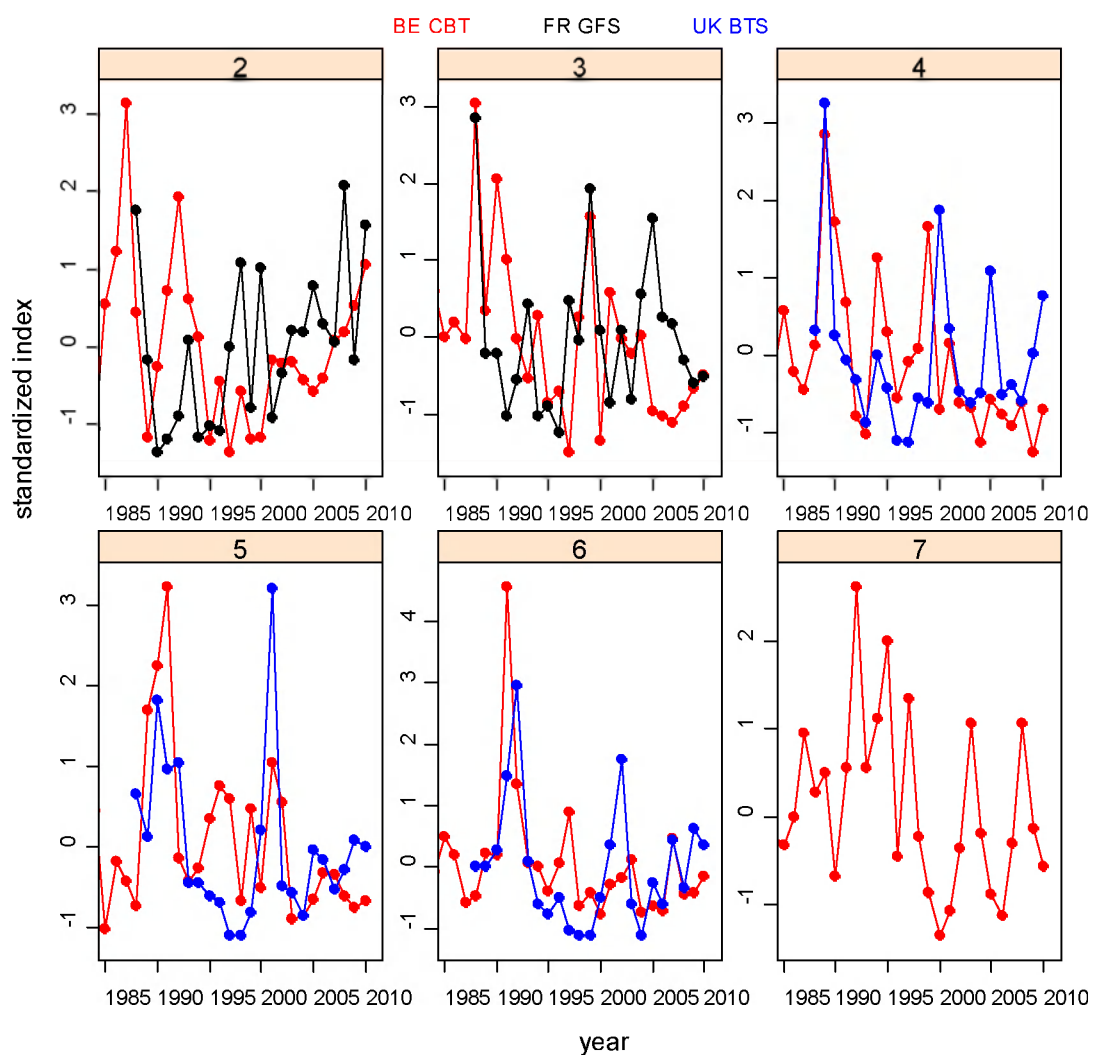
Figure 6.2.5.2. Plaiice in VIIId. Between survey consistency. Mean standardised indices by surveys for each age
