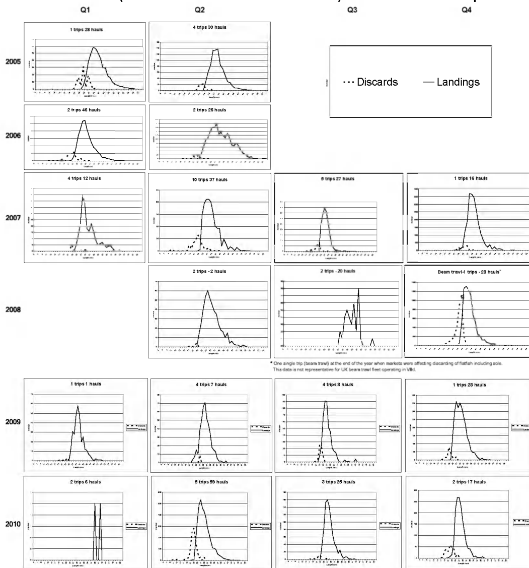
Figure 9.2.1a - Sole Vllid - UK Length distributions of discarded and retained fish from discard sampling studies for static gear (2005 - 2006 - 2007 - 2008 - 2009 - 2010) and one beam trawl trip in 2008
