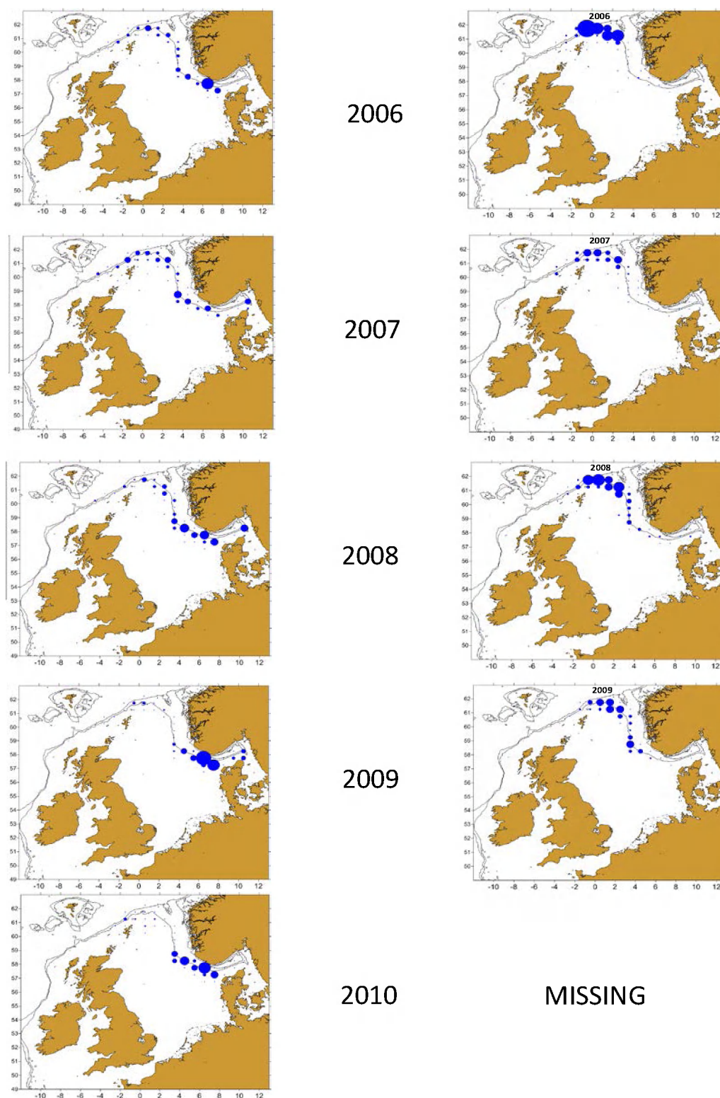
Figure 3. Spatial distribution of the catches for the GEROTR (left column) and NORTL (right column) indexes from 2006 to 2010.
