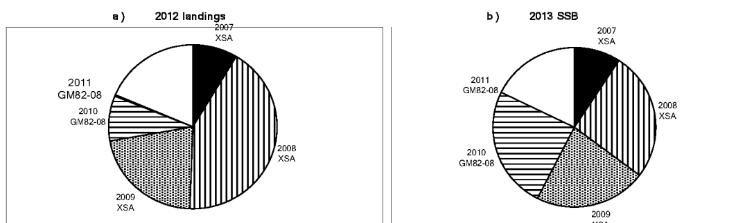
Sole Vld : Year-class % contribution to
