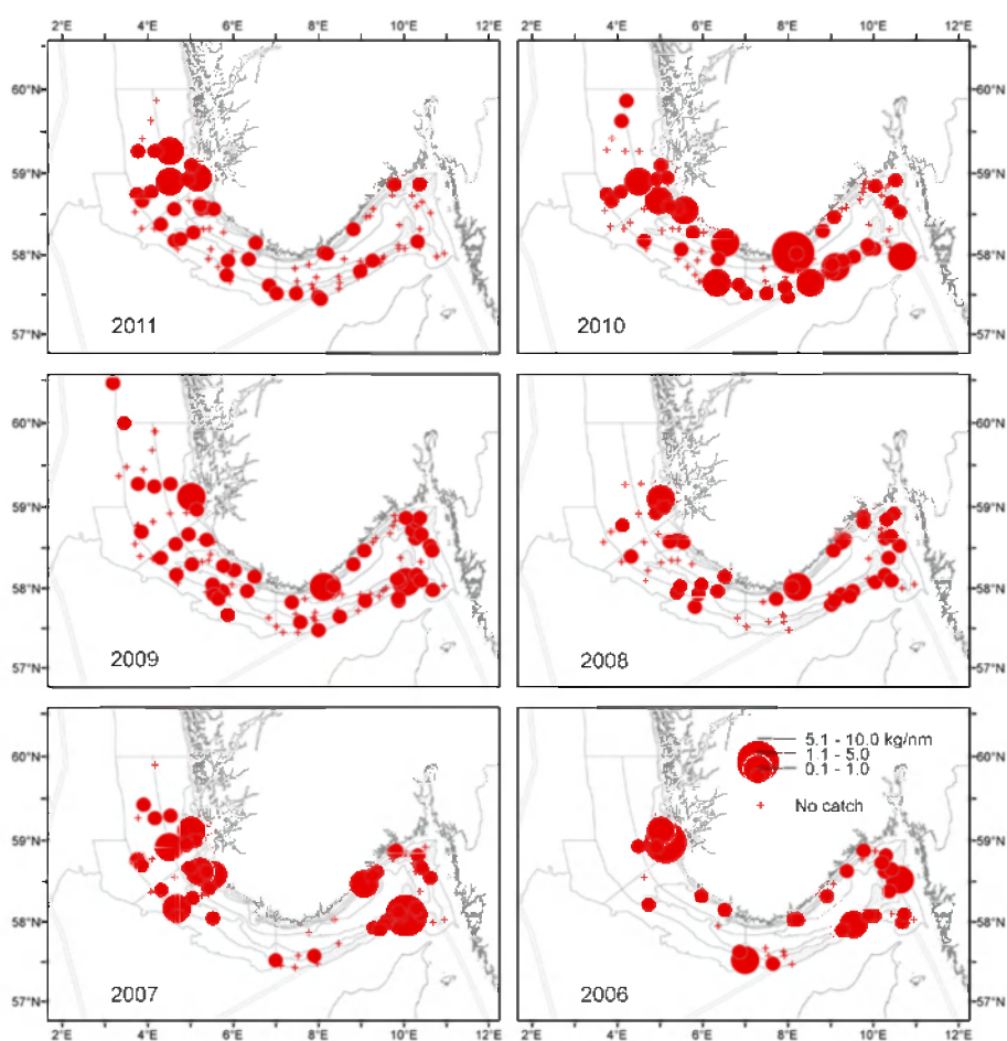
Figure A1-1. Nephrops Norwegian Deep (FU 32). Catches (kg/nm trawled) from the Norwegian shrimp survey, January-February 2006-2011.
