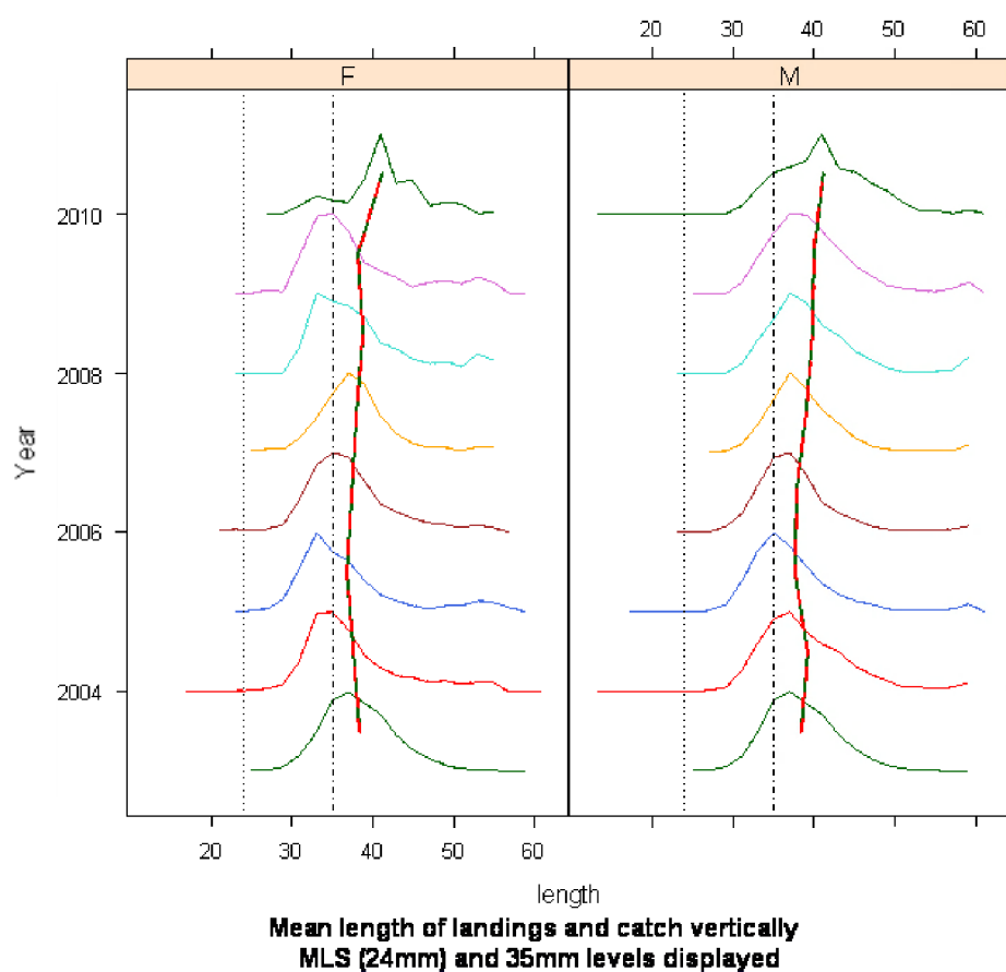
Figure 3.3.1.1 – FU5 Botney Gut/Silver Pit. Size distribution for Dutch landings, from 2003 to 2010. For 2003 the length distribution is given by sex combined.
