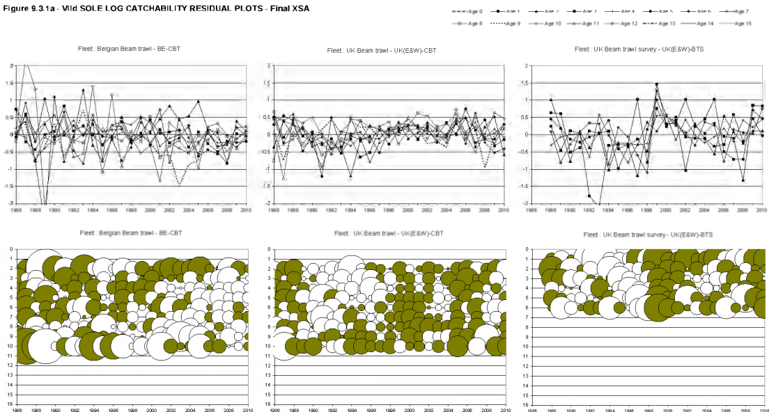
Figure 9.3.1a - Vld SOLE LOG CATCHABILITY RESIDUAL PLOTS - Final XSA
