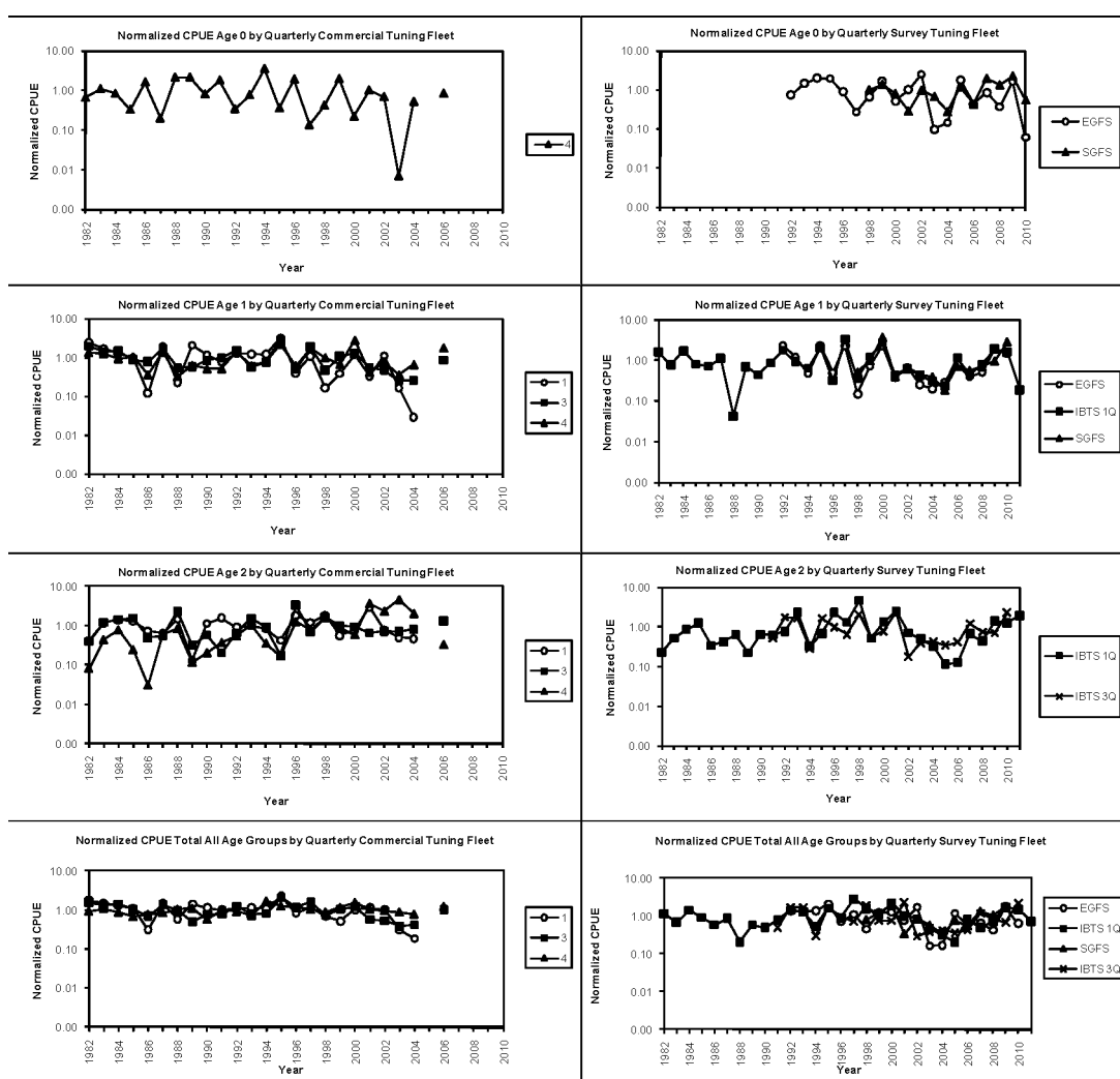
Figure 5.2.2 NORWAY POUT IV and IIIaN (Skagerak). Trends in CPUE (normalized to unit mean) by quarterly commercial tuning fleet and survey tuning fleet used in the Norway pout SXSA assessment for each age group and all age groups together.
