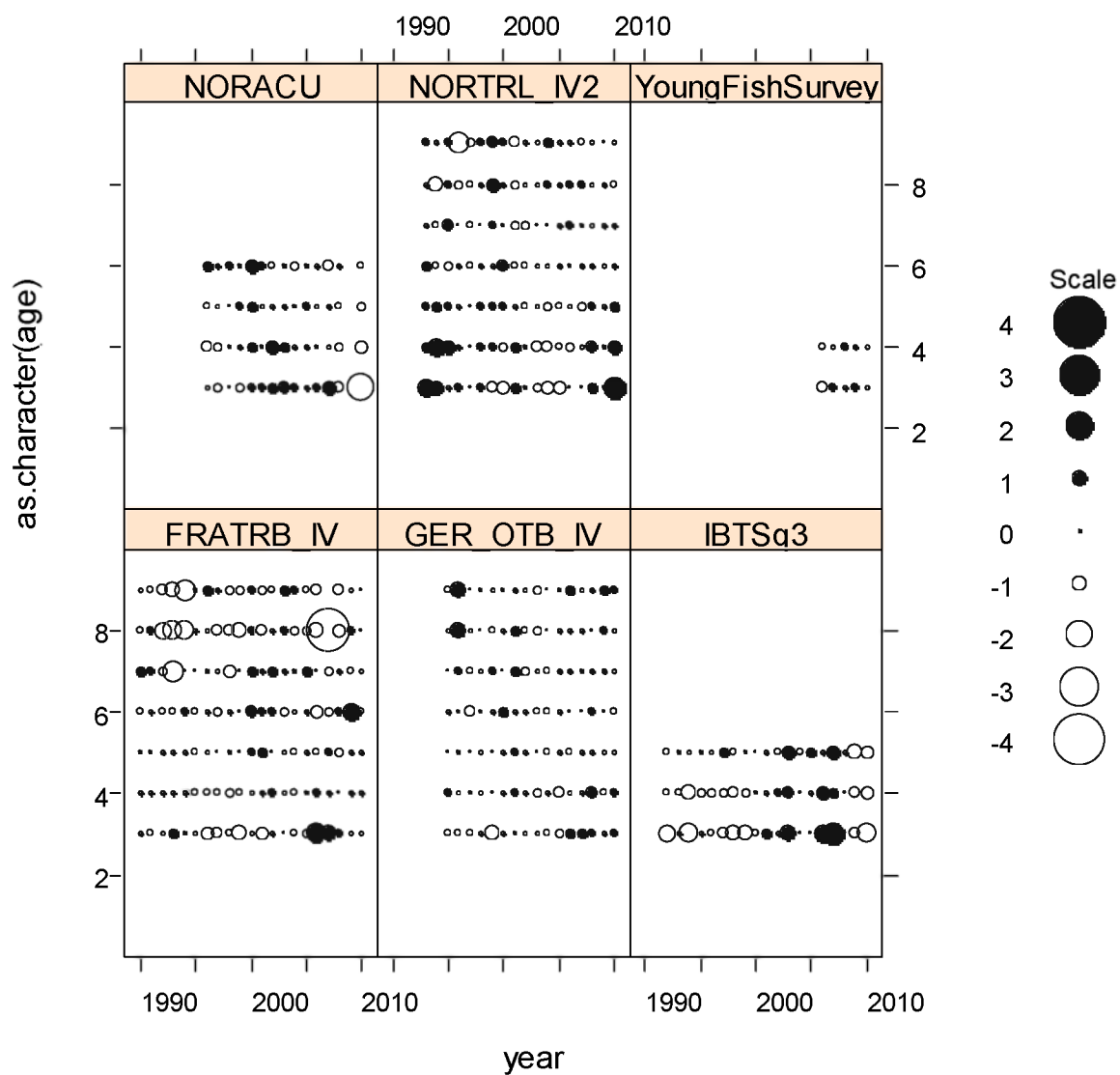
Figure 2: Residual plot
