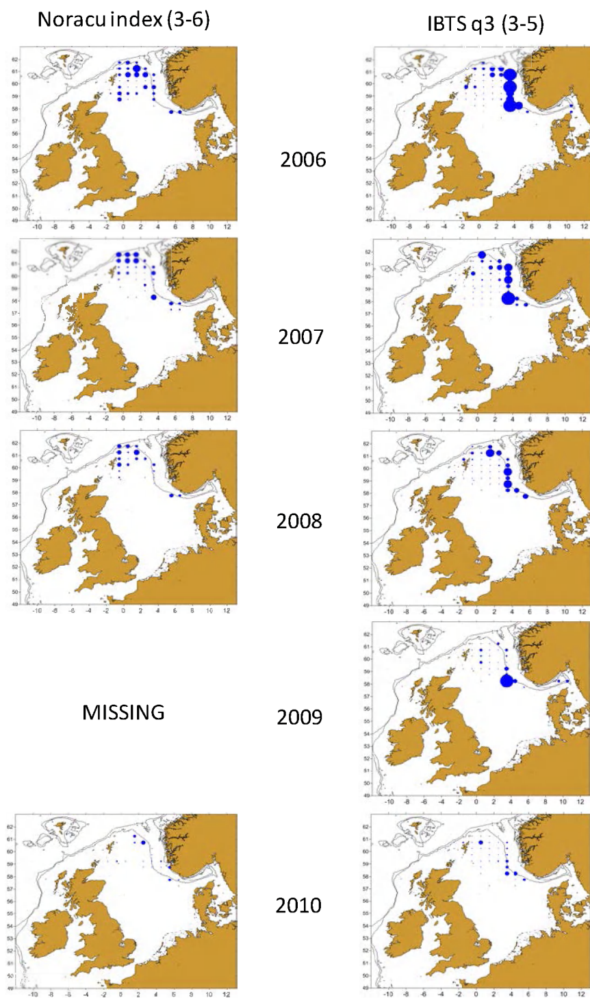
Figure 11.2.4. NORACU and IBTS Q3 indexes in the period 2006-2010.
