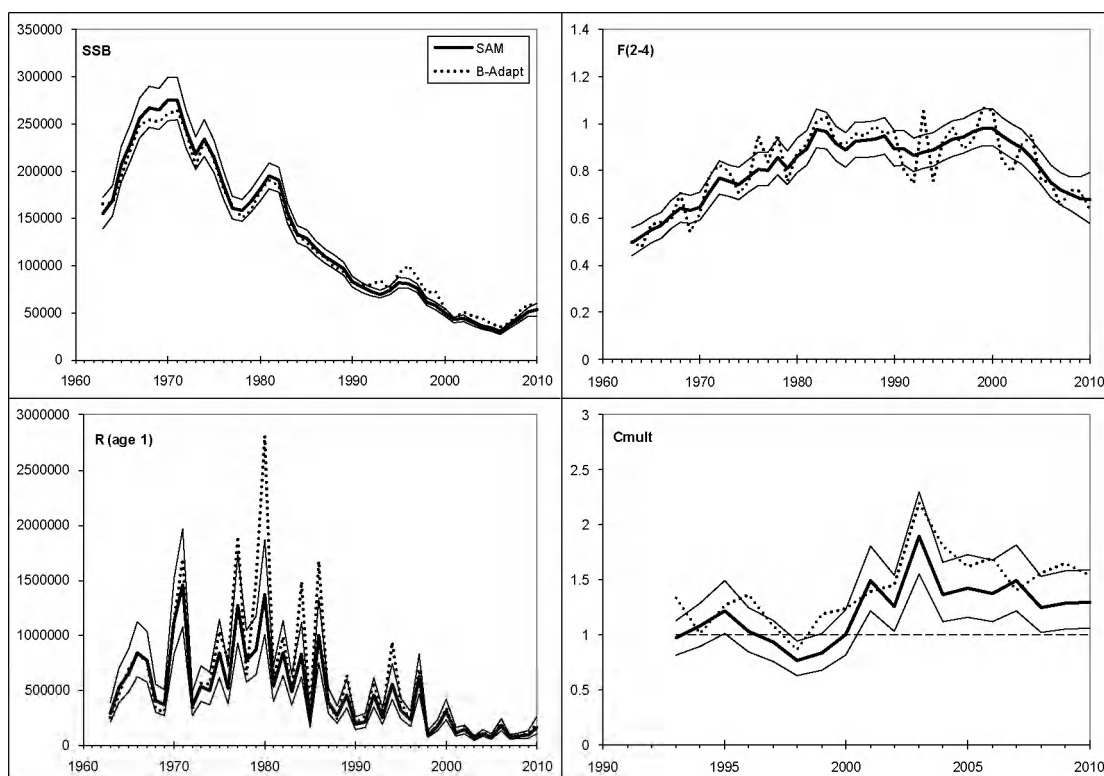
Figure 14.9 Cod in Subarea IV and Divisions IIIa (Skagerrak) and VIId. Estimated SSB, F(2-4) , recruitment (age 1) and the catch multiplier from the SAM base run. Solid black lines (heavy lines=estimate, light lines=point-wise 95% confidence intervals) are from the SAM model, and dotted lines medians from the B-ADAPT model using the same data as the SAM base run.
