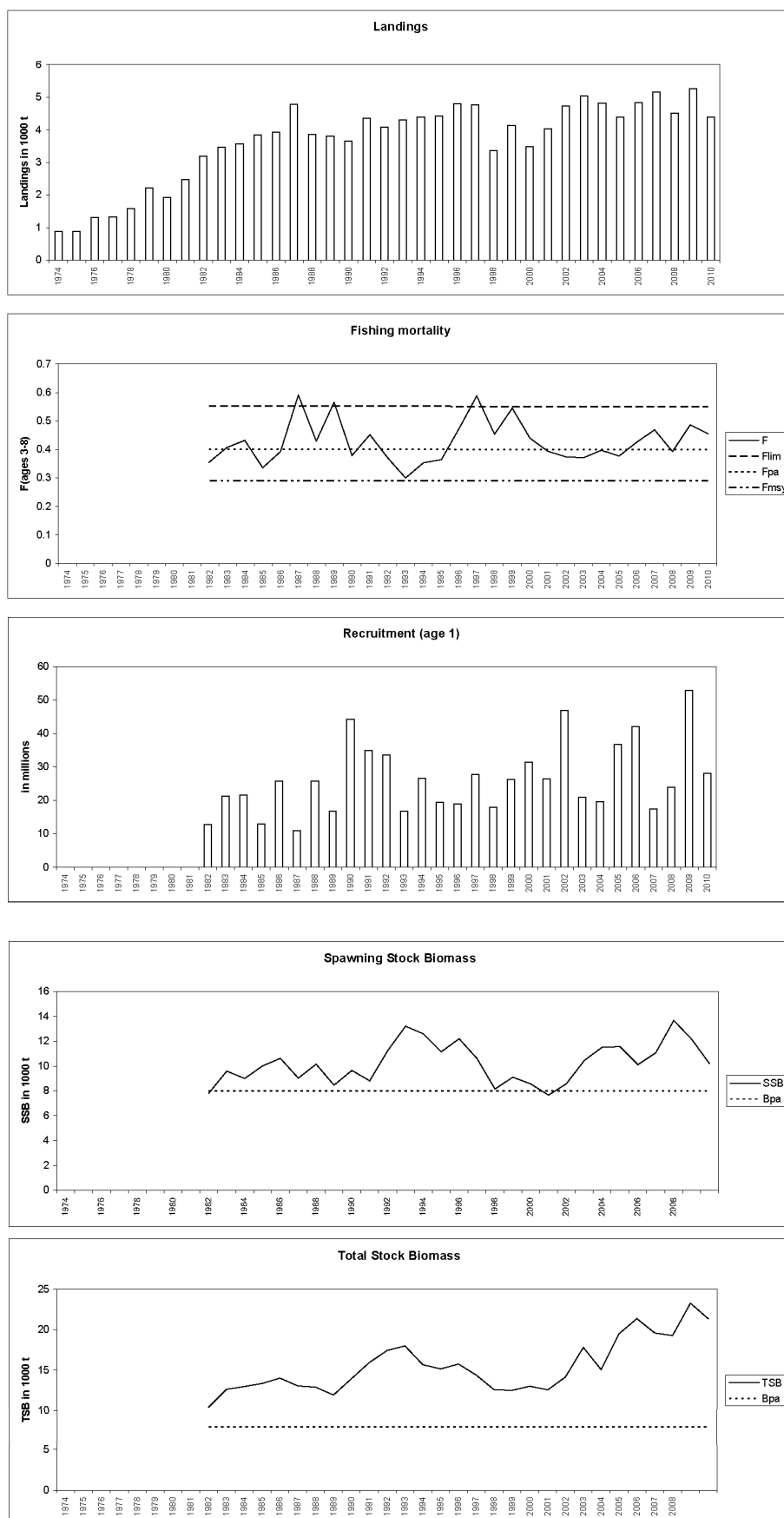
Figure 9.3.3 Sole in VIId. Summary plots
