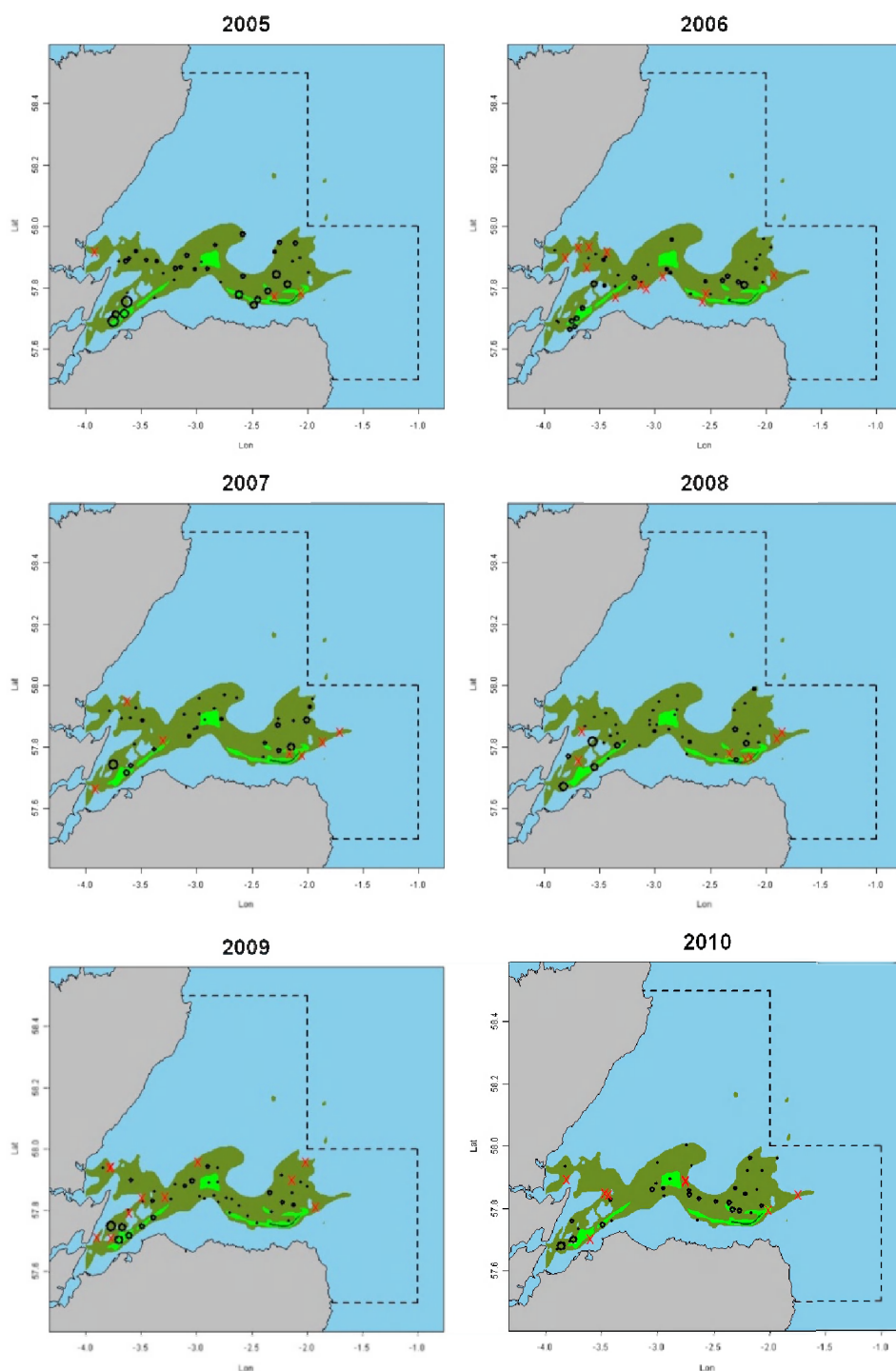
Figure 3.3.5.4 Nephrops , Moray Firth (FU 9). TV survey distribution and relative density (2005-2010). Green and brown areas represent areas of suitable sediment for Nephrops . Density proportional to circle radius. Red crosses represent zero observations.
