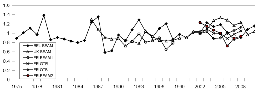
Figure 9.2.2c Sole VIId - Relative LPUE series
