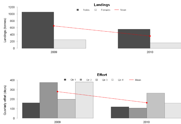
Figure 3.3.9.3. Nephrops , Devil's Hole (FU 34). Landings by sex and effort by quarter from Scottish Nephrops trawlers.
