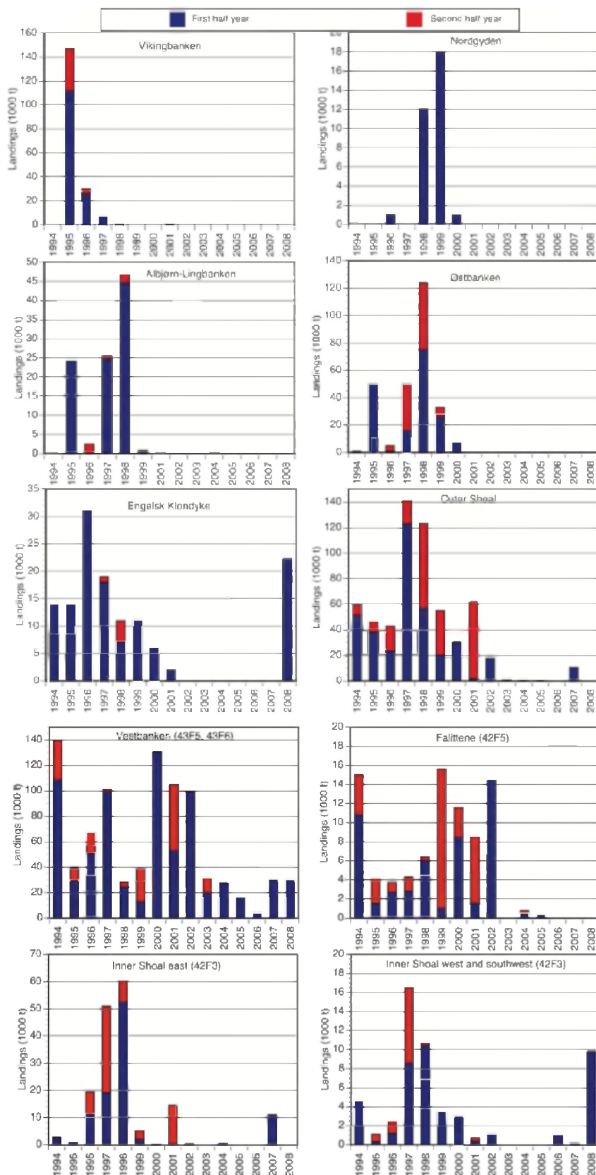
Figure 4.1.4. Sandeel in IV. Sandeel landings from Norwegian fishing banks 1994-2008 in the 1 st (blue) and 2 nd (red) half-year. Landings in 2 nd half-year are mainly 0-group
