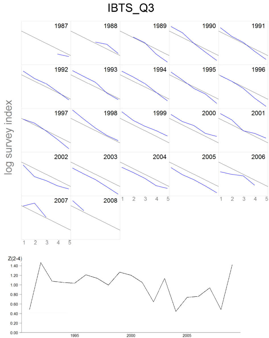
Figure 12.3.5 Whiting in IV and VII. Top panel: Log indices by cohort for the IBTS Quarter 3 survey (ages 1 to 5). The year specifies the year-class. A reference line with constant intercept and gradient representing a Z of 0.8 has been drawn in grey. Bottom panel: a raw estimate of annual mean Z averaged over ages 2 to 4, Z at age was estimated as \log \text{index}(y, a) - \log \text{index}(y+1, a+1) .
