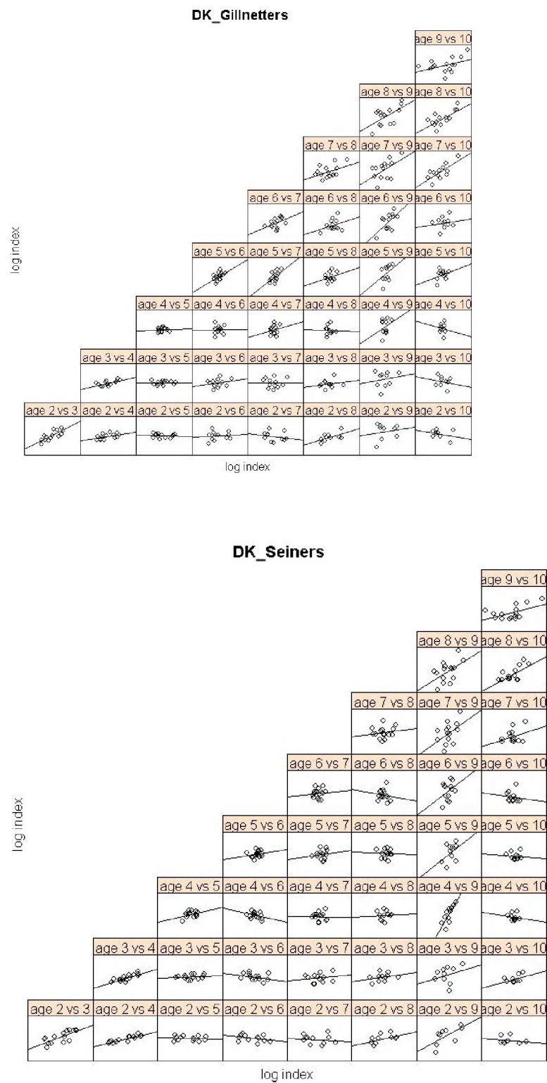
Figure 7.3.2. Plaiice IIIa. Internal consistency for the commercial tuning fleets: matrix scatterplots and Log cohort abundance. Up : DK_Gillnetters. Bottom: DK_Seiners.
