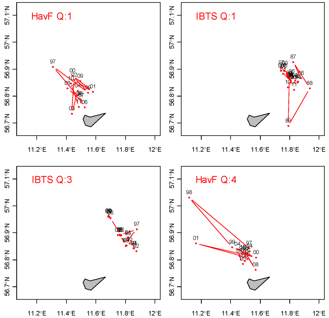
Figure COG-1. Centre of gravity for trawl stations in the Quarter 1 Havfisken, Quarter 1 IBTS, Quarter 3 IBTS and Quarter 4 Havfisken surveys.
