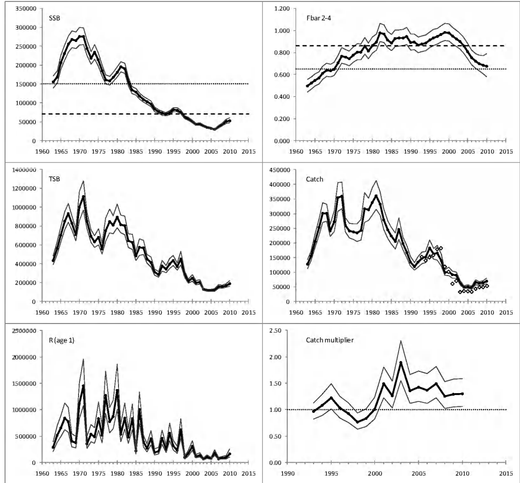
Figure 1a. North Sea cod. Clockwise from top left, point-wise estimates and 95% confidence intervals of spawning stock biomass (SSB), total stock biomass (TSB), recruitment ( R(\text{age } 1) ), the catch multiplier, catch and F_{\text{bar}} (catch, ages 2-4), from the SAM base run. The heavy lines represent the point-wise estimate, and the light lines point-wise 95% confidence intervals. The open diamonds given in the catch plot represent model estimates of the total catch excluding unallocated mortality, while the solid lines represent the total catch including unallocated mortality from 1993 onwards. The horizontal broken lines in the SSB plot indicate B_{\text{lim}}=70\,000\text{t} and B_{\text{pa}}=150\,000\text{t} , and those in the F_{\text{bar}} plot F_{\text{pa}}=0.65 and F_{\text{lim}}=0.86 . The horizontal broken line in the catch multiplier plot indicates a multiplier of 1. Catch, SSB and TSB are in tons, and R in thousands.
