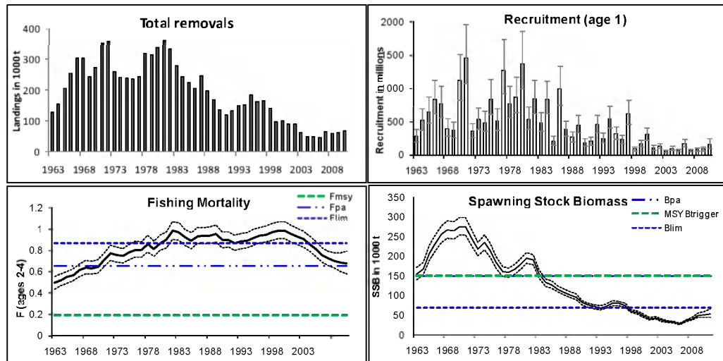
Figure 4: Cod in Subarea IV (North Sea), Division VIIId (Eastern Channel), and IIIa West (Skagerrak). Summary of stock assessment with point-wise 95% confidence intervals, catch estimated, and adjusted for unallocated removals (from 1993), weights in tonnes
