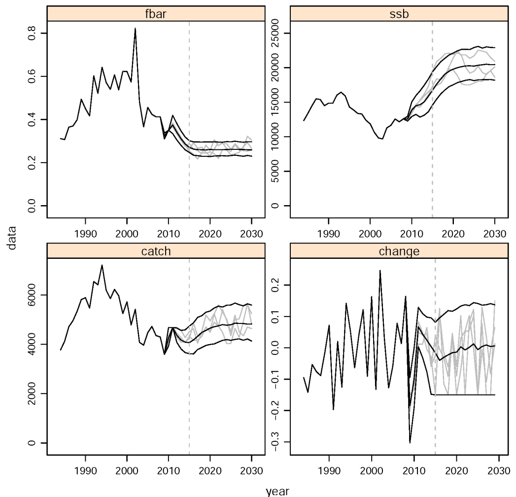
Figure 9.3. Fishing mortality, ssb, landings and proportion change in landings (TAC) for a progressive 9% reduction in fishing mortality until F=F_{msy} (0.26) with 15% limit to annual change in TAC, applied over the period 2012 to 2030. solid lines show 5th, 50th and 95th percentiles, light grey lines show a small random selection of actual trajectories. Vertical dotted line drawn at 2015.
