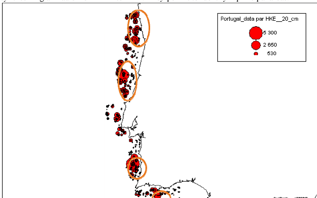
Fig. 9: <20cm hake distribution in number per haul (P-GFS survey from 2003-2010) with the main concentration areas identified along the years.
