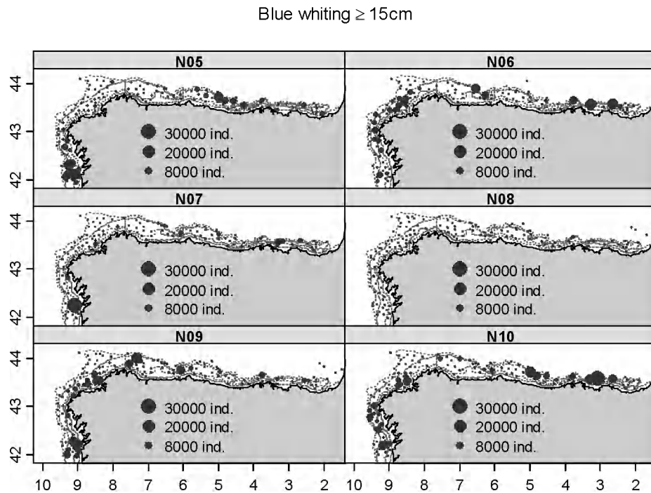
Figure 29. Distribution of blue whiting larger than MLS ( \geq 15\text{ cm} ) in Northern Spanish Shelf Ground-fish between 2005 and 2010
