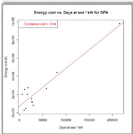
Fig. 4 Energy cost vs. Days at sea*kW for DFN
