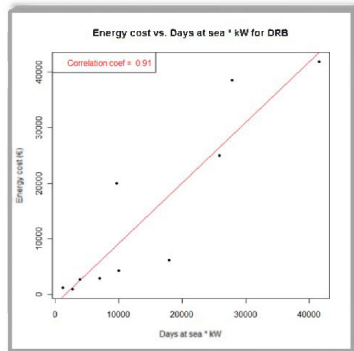
Fig. 5 Energy cost vs. Days at sea*kW for DRB
