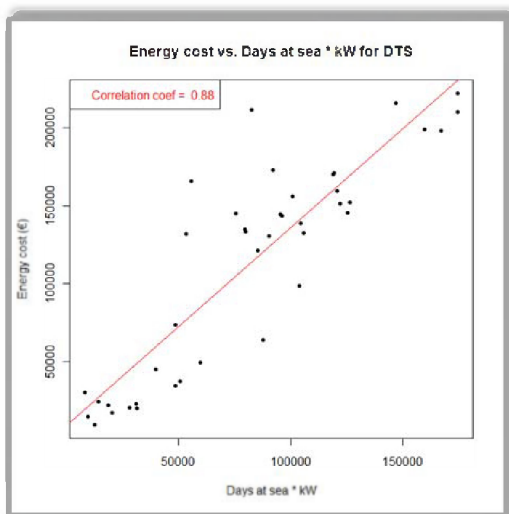
Fig. 6 Energy cost vs. Days at sea*kW for DTS
