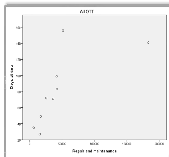
Fig. 45 Repair and maintenance costs vs. Days at sea for OTT
