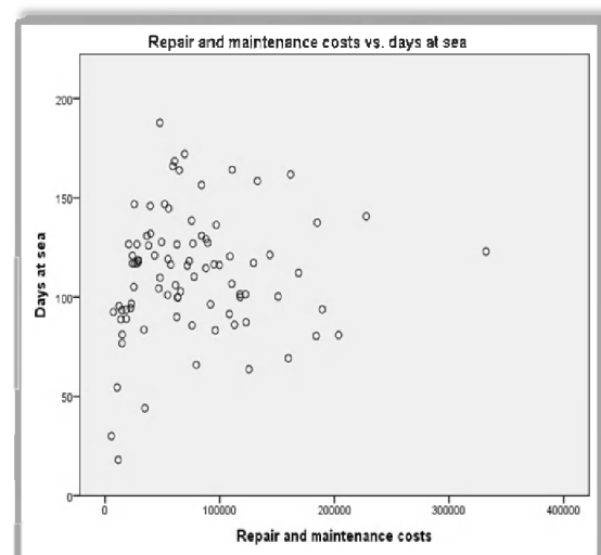
Fig. 40 Repair and maintenance costs vs. Days at sea
