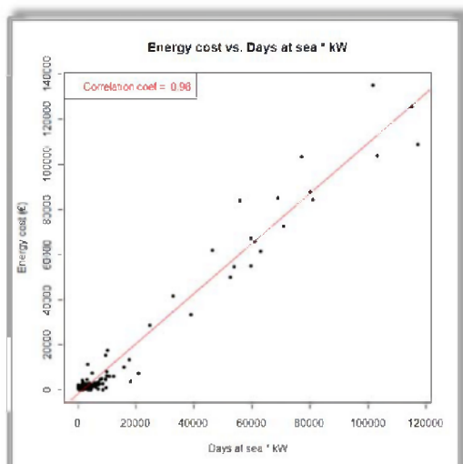
Fig. 49 Energy cost vs. Days at sea * kW
