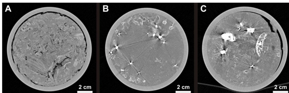
Fig. 4.4 Expressions of early diagenetic processes within the mounds: (A) dissolution of the cold-water corals, (B) the formation of small pyrite crystals (white structures), and (C) the formation of large pyrite nodules (white structures) and the pyritisation of the cold-water coral fragments.
