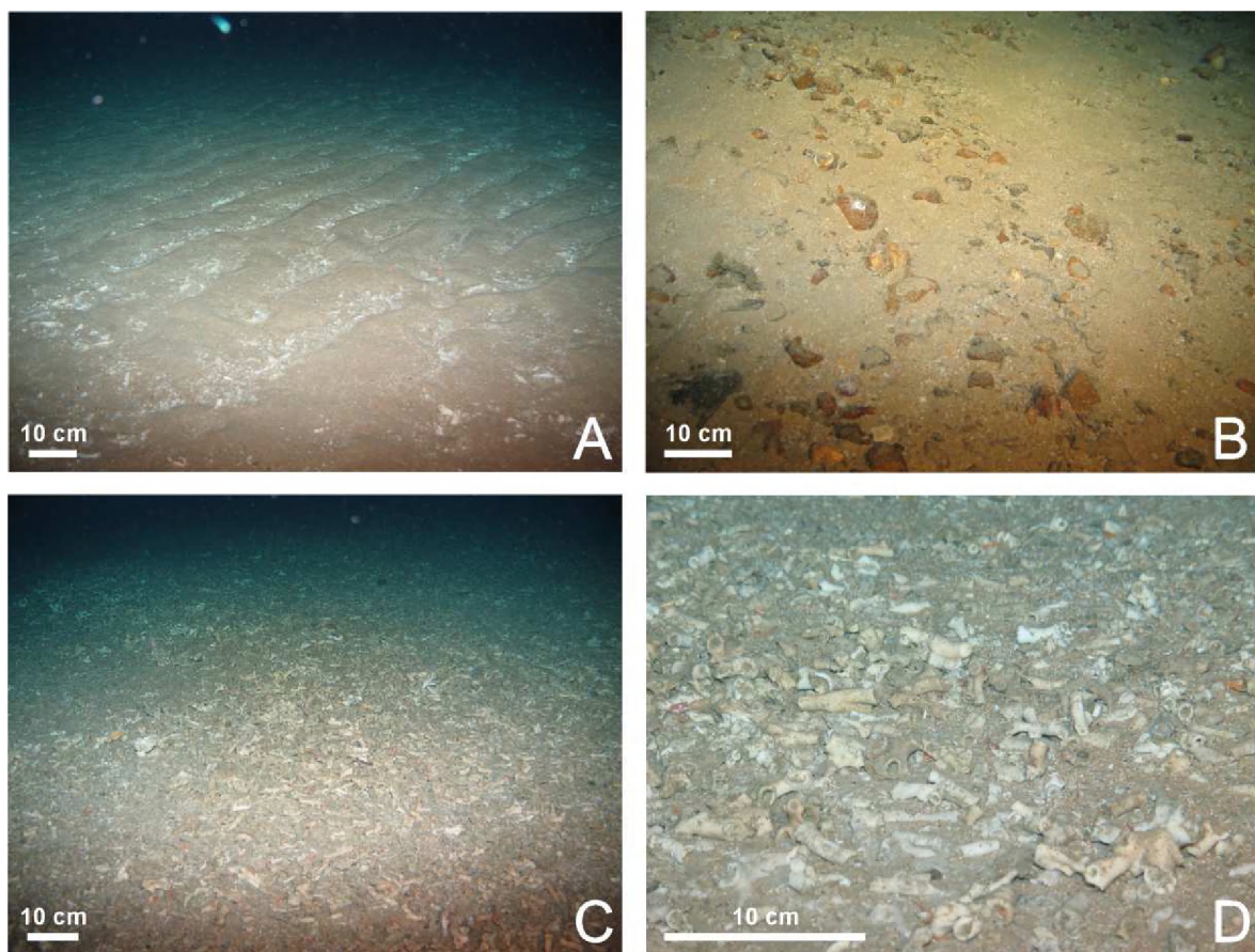
Fig. 5.3 ROV images from the shallow-water setting (ROV dive B08-03): (A) rippled seabed with a patchy distribution of cold-water corals, (B) coarse sand with a high amount of gravel, (C) the dense cold-water coral rubble coverage on top of the small mounds, and (D) zoom in this coral rubble facies with predominantly Lophelia pertusa .
