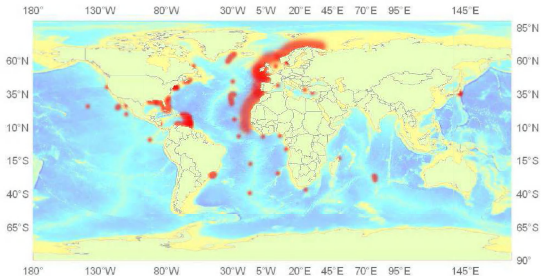
Fig. 1.4 Distribution of Lophelia pertusa (after Freiwald et al., 2004; source: http://www.lophelia.org ).
