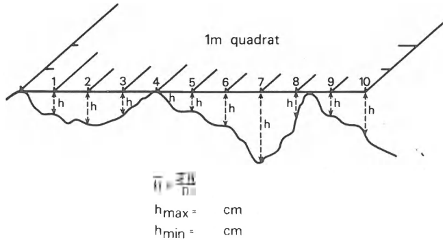
FIG. 23. Measurements of dissection, h.
