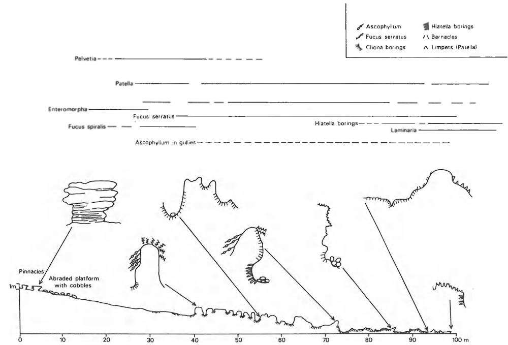
FIG. 30. Coastal section at Penmon, Anglesey, N. Wales.
