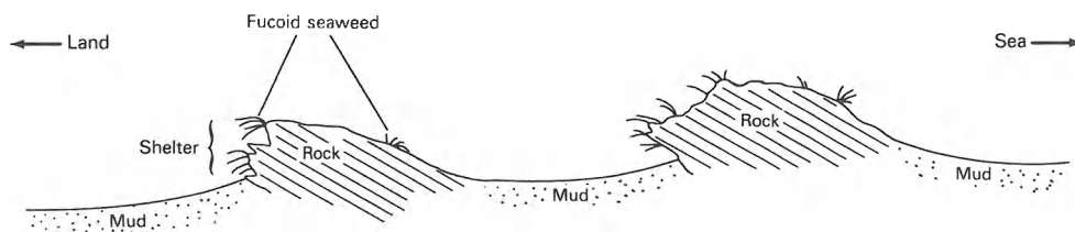
FIG. 33. Field Sketches, Blue Anchor Bay, Somerset.
