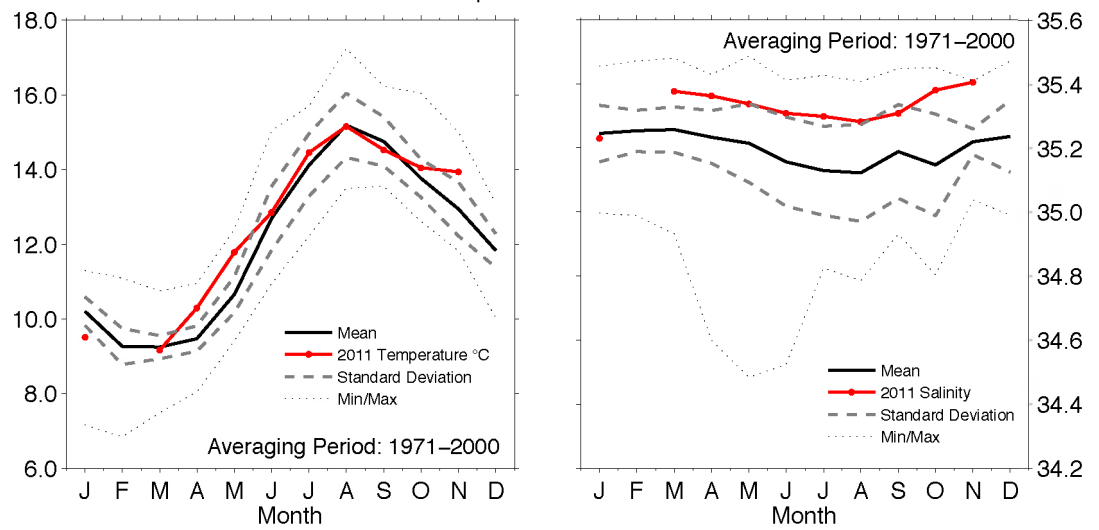
Figure 42. Area 4b – Northwest European continental shelf. 2011 monthly temperature (left panel) and salinity (right panel) of surface water at Station E1 in the western English Channel (50.03°N 4.37°W).
