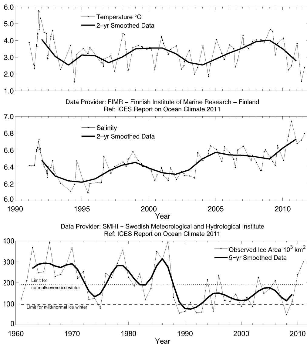
Figure 62. Area 9b – Skagerrak, Kattegat, and the Baltic. Temperature (upper panel) and salinity (middle panel) at Station SR5 in the Bothnian Sea, and ice extent (lower panel) starting from 1961
