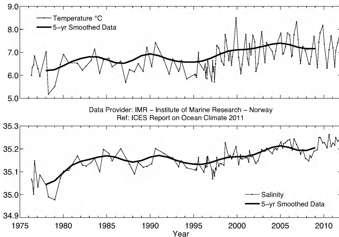
Figure 64. Area 10 – Norwegian Sea. Average temperature (upper panel) and salinity (lower panel) above the slope at Gimsoy Section (69°N).
