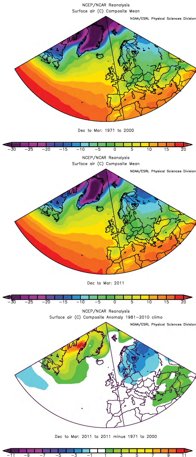
Figure 12. Winter (DJFM) surface air temperature fields. Top panel: surface air temperature averaged over 30 years (1971–2000). Middle panel: temperatures in winter 2011 (December 2010, January to March 2011). Bottom panel: winter 2011 surface air temperature anomaly – the difference between the top and middle panels. Images provided by the NOAA/ESRL Physical Sciences Division, Boulder, CO (available online at http://www.cgd.noaa.gov/ ).
