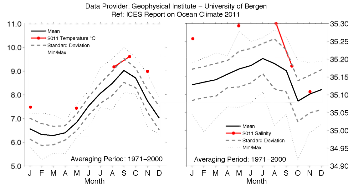
Figure 67. Area 10 – Norwegian Sea. 2011 monthly temperature (left panel) and salinity (right panel) at 50 m at Ocean Weather Station "M" (66°N 2°E).
