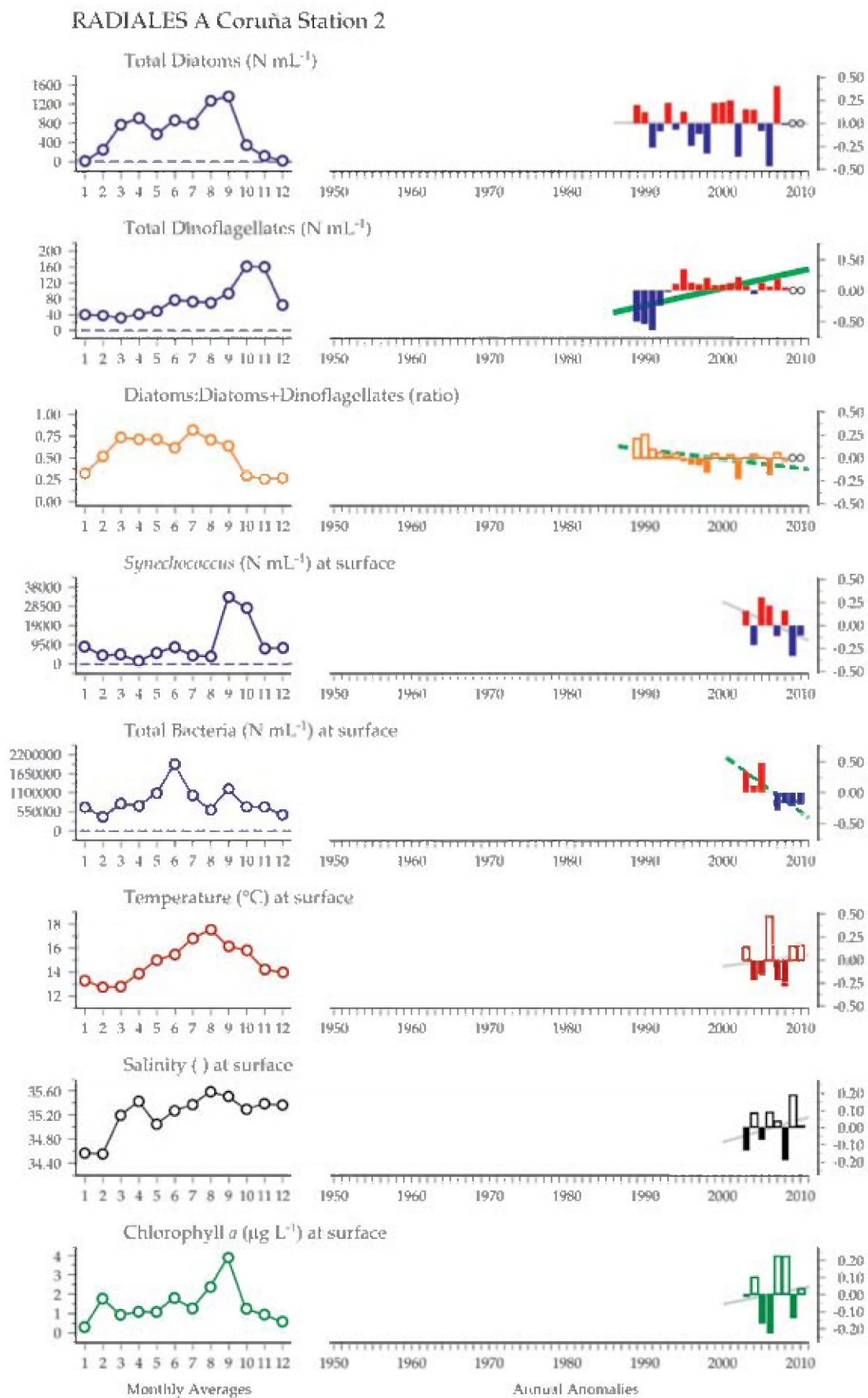
Figure 8.5.2 Multiple-variable comparison plot (see Section 2.2.2) showing the seasonal and interannual properties of select cosampled variables at the RADIALES A Coruña station 2 plankton monitoring site. Additional variables from this site are available online at http://wgpmc.net/time-series .
