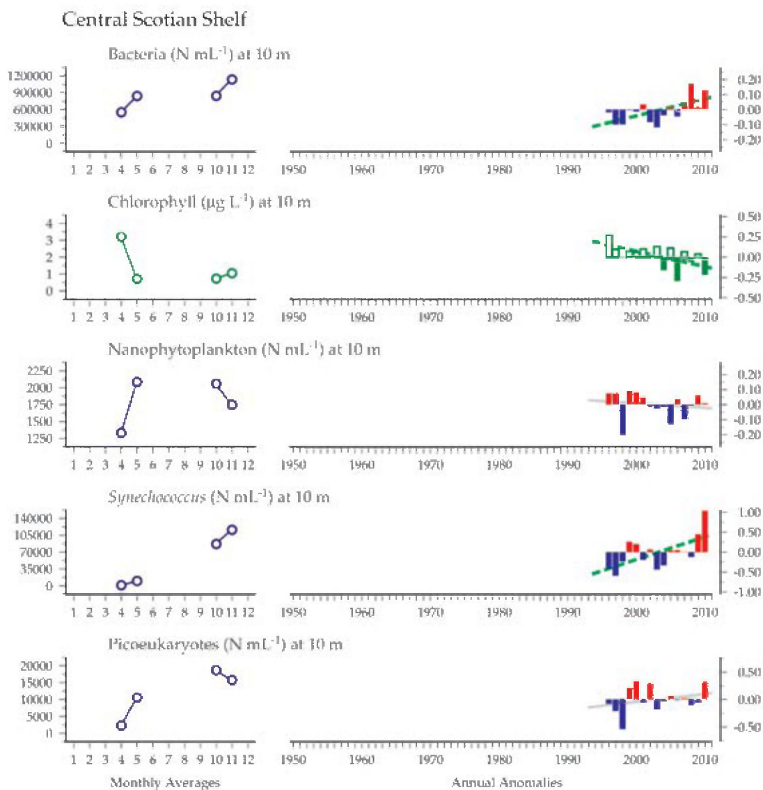
Figure 3.4.3 Multiple-variable comparison plot (see Section 2.2.2) showing the seasonal and interannual properties of select cosampled variables at the Central Scotian Shelf plankton monitoring site. Additional variables from this site are available online at http://wgpme.net/time-series .
