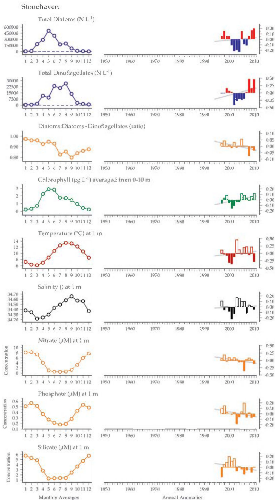
Figure 6.4.2 Multiple-variable comparison plot (see Section 2.2.2) showing the seasonal and interannual properties of select cosampled variables at the Stonehaven plankton monitoring site. Additional variables from this site are available online at http://wgpmc.net/time-series .
