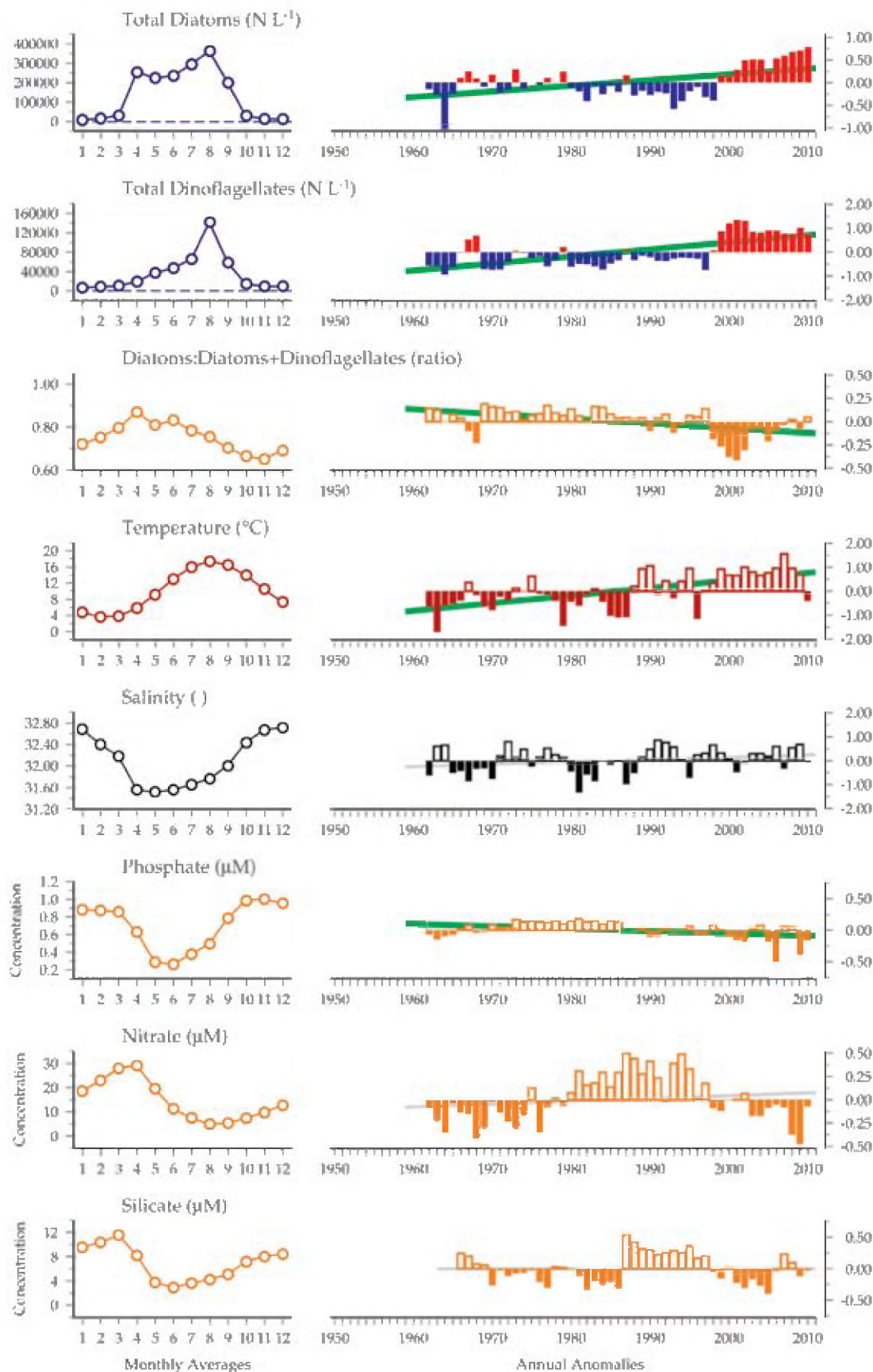
Figure 6.1.2 Multiple-variable comparison plot (see Section 2.2.2) showing the seasonal and interannual properties of select cosampled variables at the Helgoland Roads plankton monitoring site. Additional variables from this site are available online at http://wgpme.net/time-series .
