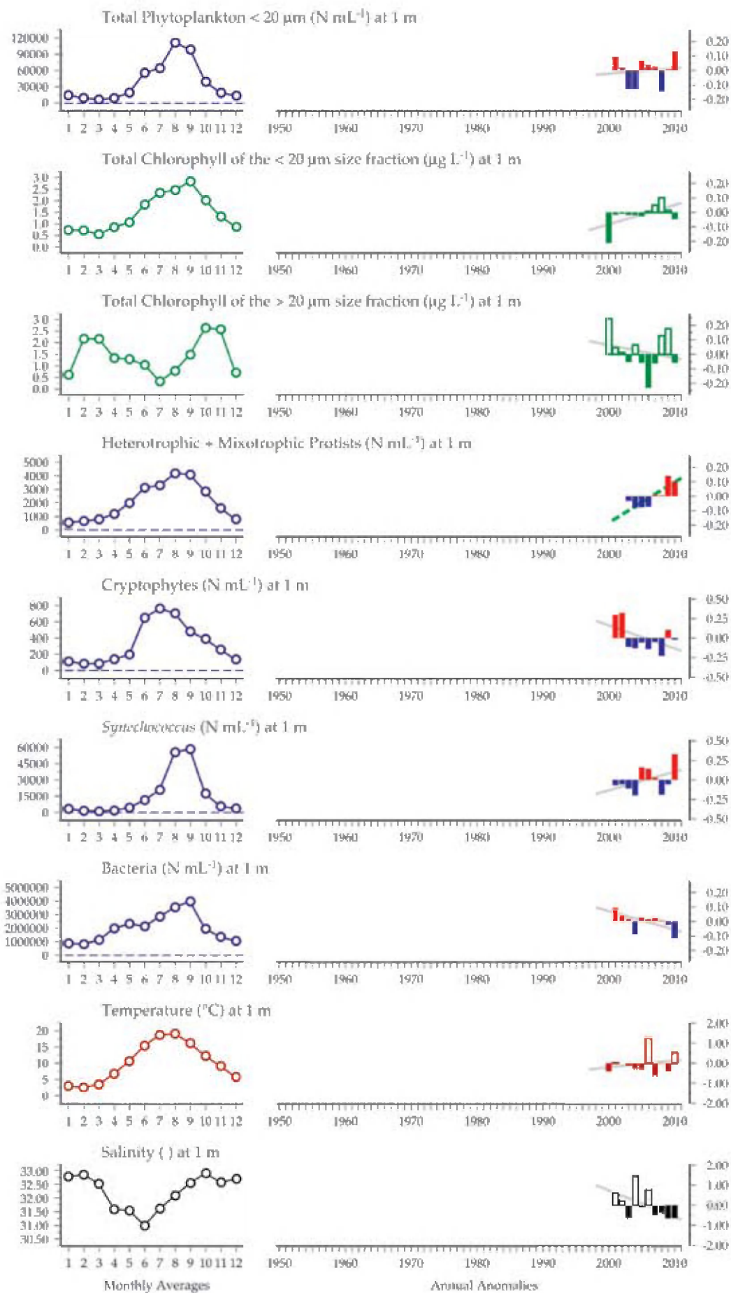
Figure 3.1.2 Multiple-variable comparison plot (see Section 2.2.2) showing the seasonal and interannual properties of select cosampled variables at the Booth Bay, Maine plankton monitoring site. Additional variables from this site are available online at http://wgpme.net/time-series .
