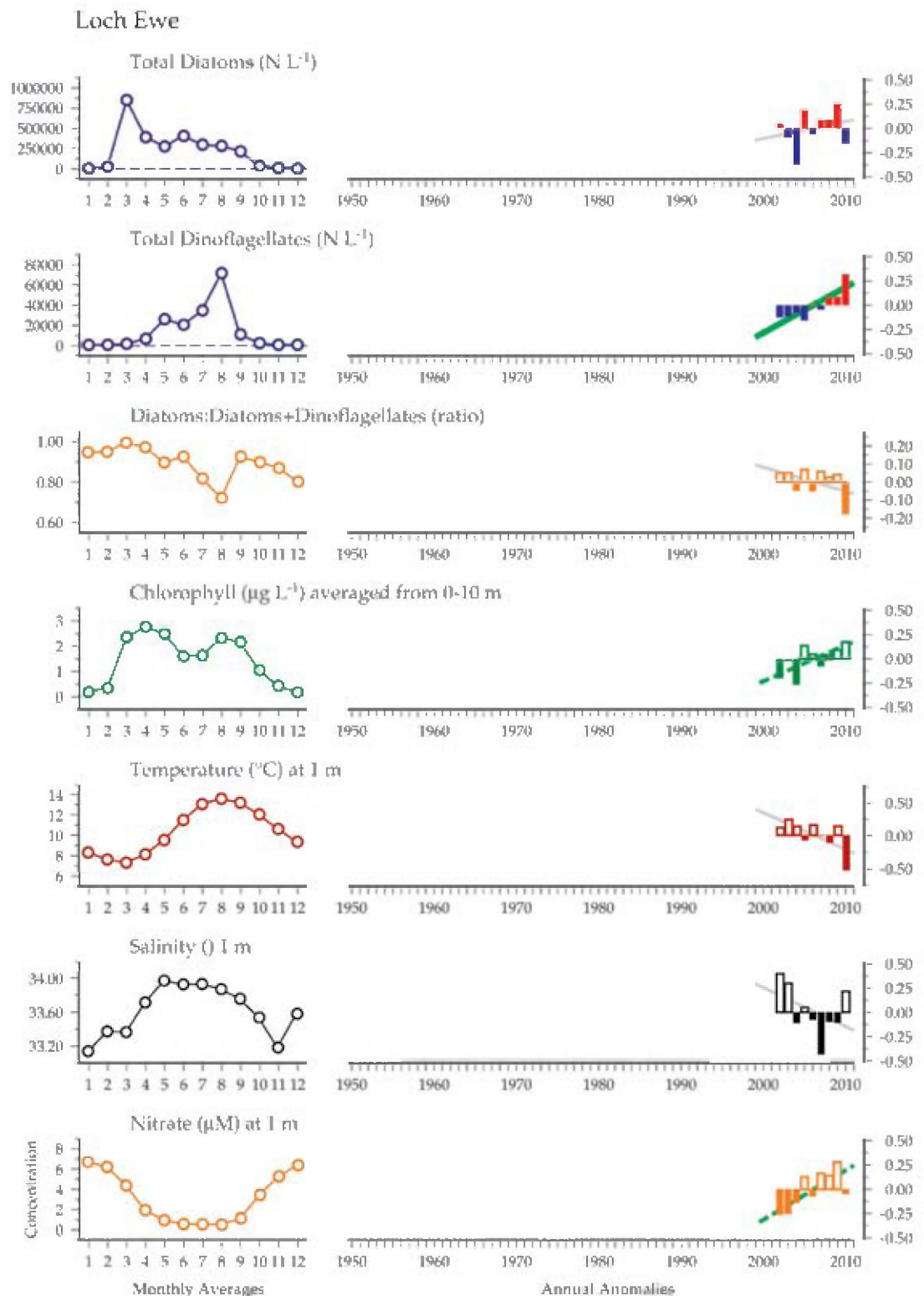
Figure 7.1.2 Multiple-variable comparison plot (see Section 2.2.2) showing the seasonal and interannual properties of select cosampled variables at the Loch Ewe plankton monitoring site. Additional variables from this site are available online at http://wgpmc.net/time-series .
