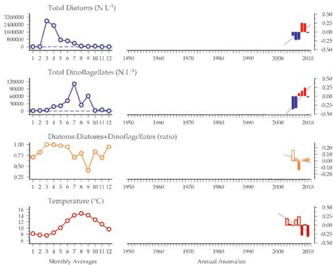
Figure 7.3.2 Multiple-variable comparison plot (see Section 2.2.2) showing the seasonal and interannual properties of select cosampled variables at the Millport plankton monitoring site. Additional variables from this site are available online at http://wgpme.net/time-series .
