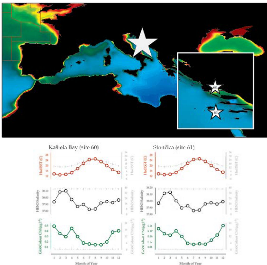
Figure 9.5.1 Locations of the Kaštela Bay and Stončica plankton monitoring areas (Sites 60–61), plotted on a map of average chlorophyll concentration, and their corresponding environmental summary plots (see Section 2.2.1).
