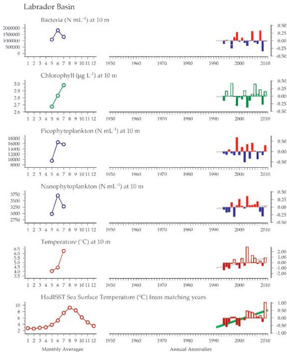
Figure 4.1.3 Multiple-variable comparison plot (see Section 2.2.2) showing the seasonal and interannual properties of select cosampled variables at the Labrador Basin plankton monitoring site. Additional variables from this site are available online at http://wgpme.net/time-series .
