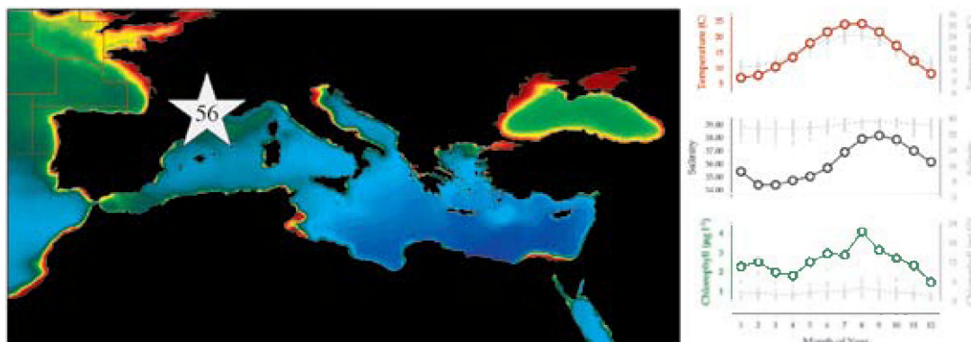
Figure 9.2.1 Location of the Thau Lagoon plankton monitoring area (Site 56), plotted on a map of average chlorophyll concentration, and its corresponding environmental summary plot (see Section 2.2.1).
