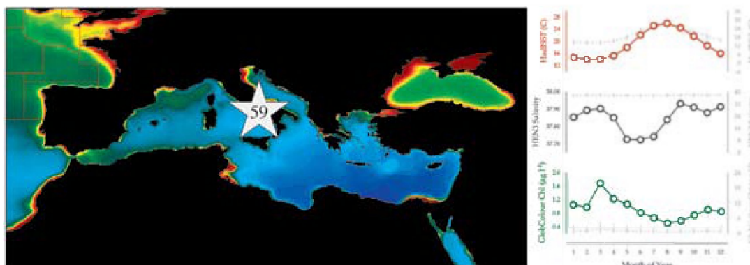
Figure 9.4.1 Location of the Gulf of Naples LTER-MC plankton monitoring area (Site 59), plotted on a map of average chlorophyll concentration, and its corresponding environmental summary plot (see Section 2.2.1).
